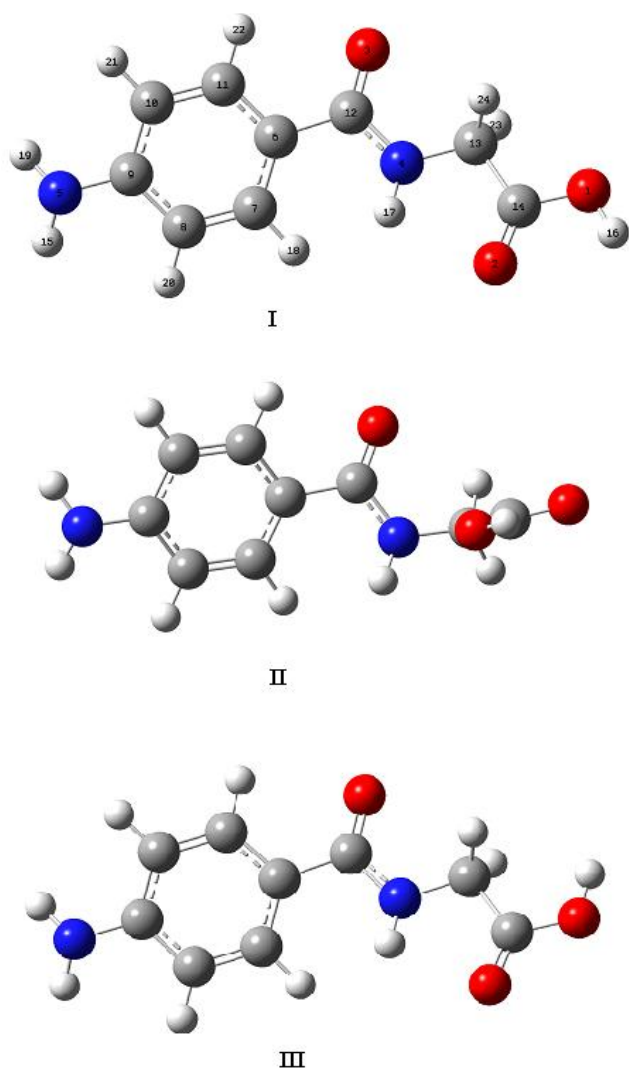
Fig. 1. Optimized structures of the three most stable conformers of PAH.
