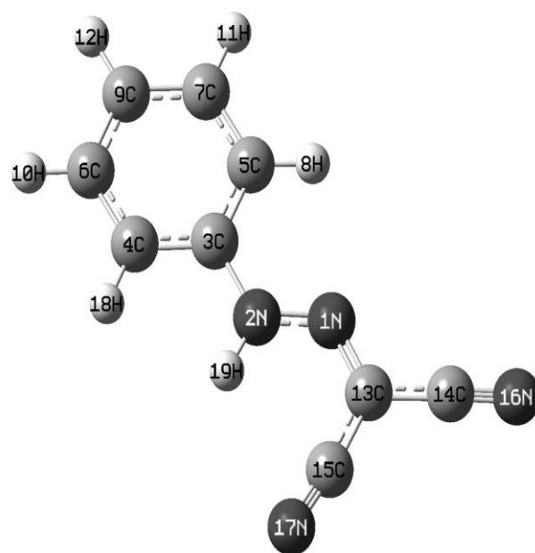
Hydrazo
