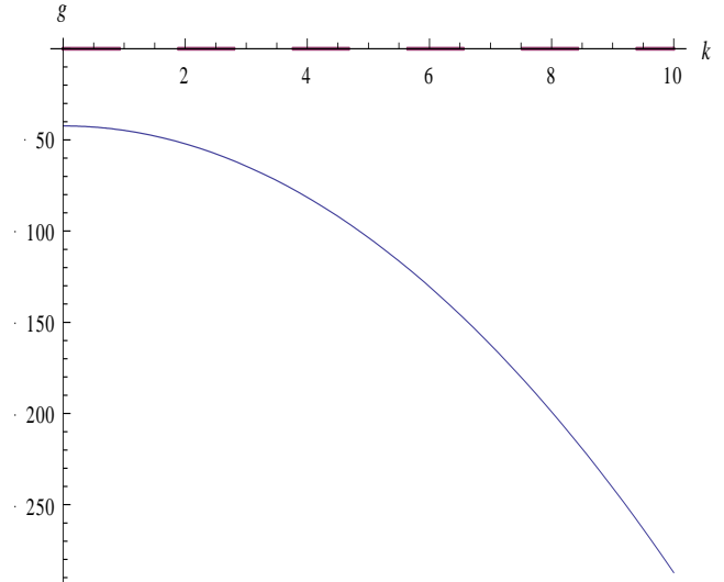
Fig. 2. Wave vector dependence of the ground state g -factor for the electron.
