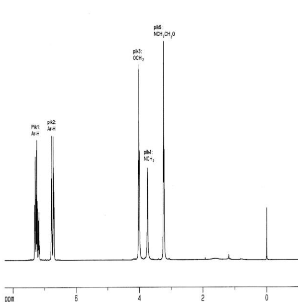
Fig.3. 400 MHz ^1\text{H-NMR} spectrum of ligand1 ( \text{CDCl}_3 ). Peak1:Ar-H; peak2:Ar-H; peak3:OCH 2 ; peak4:NCH 2 ; peak5:NCH 2 CH 2 O
