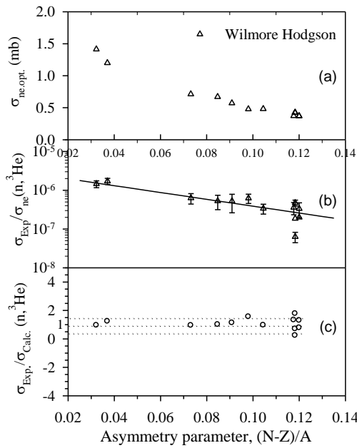
Fig.2. a) Optical model neutron non-elastic cross-section from Wilmore-Hodgson built-in parameters by depending upon asymmetry parameter, b) The experimental points were fitted with \sigma(n,^3\text{He})=C' \sigma_{ne-opt} \exp[bs] and correlation coefficient for Wilmore-Hodgson (solid line) built-in parameters was determined as R = 0.96 , c) Ratios of the ( n,^3\text{He} ) experimental cross sections to the cross-sections calculated with empirical and semi-empirical formulae.
