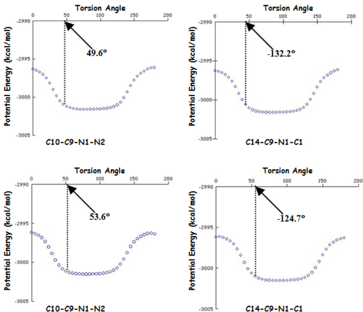
Fig.3. The potential energies as a function of torsion angles.
