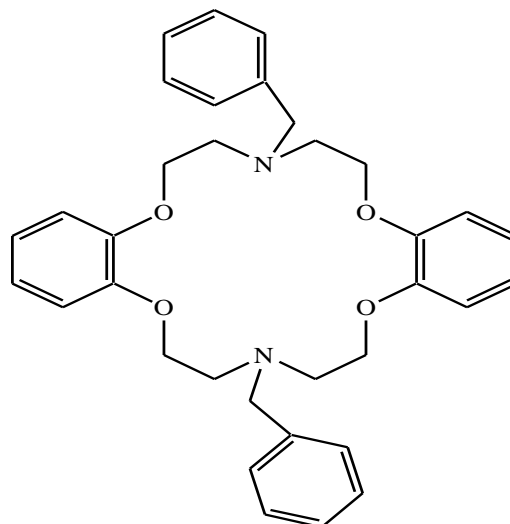
Fig.1. Ligand 1 N,N'-Dibenzil-7,16-diaza-1,4,10,13-tetraoksa-2,3,11,12-dibenzosikloktadeka-2,11-dien
