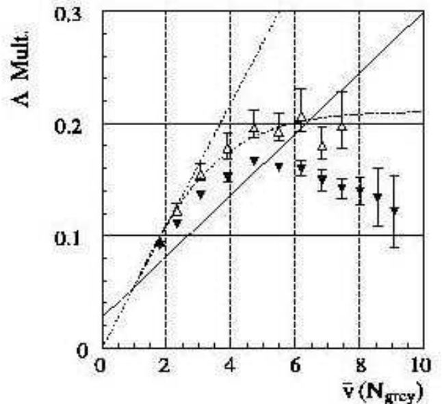
Fig.3 The A yield versus \bar{v} .
