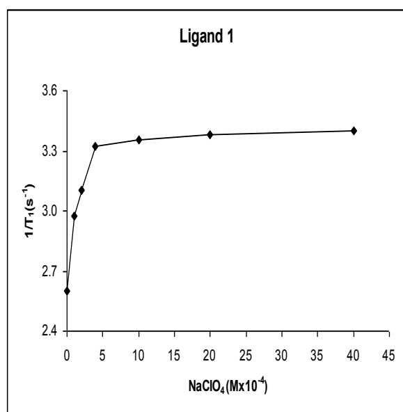
Fig. 2. Spin-lattice relaxation rates versus concentration of Na+ ions for ligand 1
