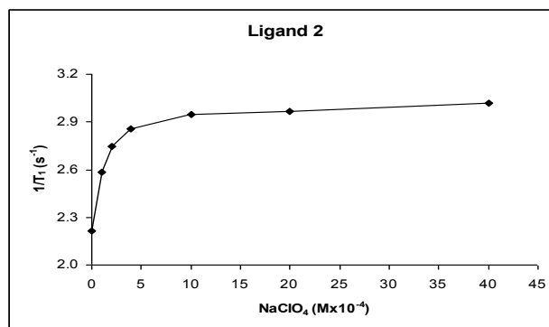
Fig.3 Spin-lattice relaxation rates versus concentration of Na+ ions for ligand 2
