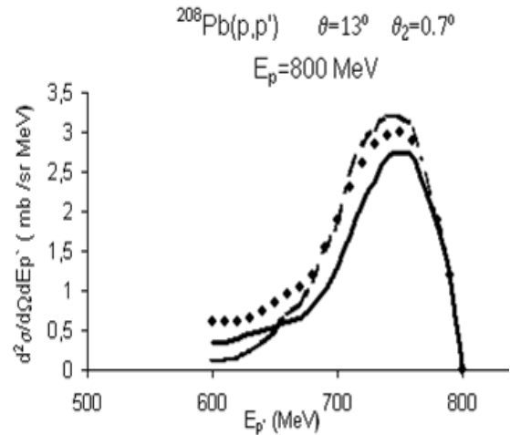
Fig.2. Energy spectra for 800 MeV ( p, p' ) reactions on ^{208}\text{Pb} at scattering angle 13^\circ . The dots curve is the measured spectra, the dashed curve is the calculated results in the surface response model [4], solid curve - of the calculated results.
