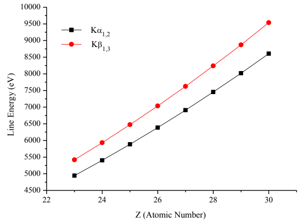
Fig. 2 Line energy of the 3d elements as a function of the atomic number.
