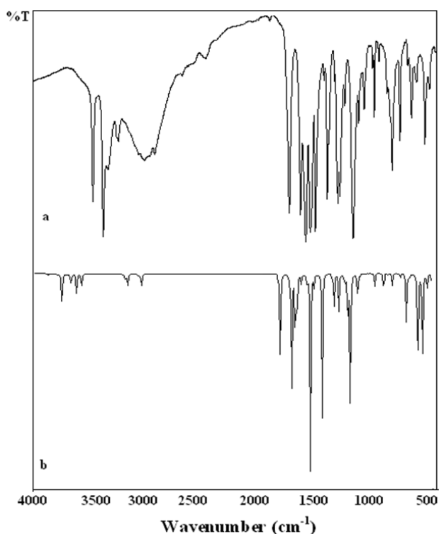
Fig. 3. FTIR spectrum of solid PAH in a KBr disk (a) and calculated spectrum (b)
