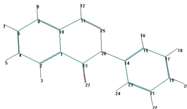
Fig. 2. A HyperChem drawing of molecule.
