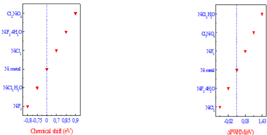
Fig. 3. Chemical shift and \Delta FWHM (eV) for K\alpha lines of Ni compounds.
