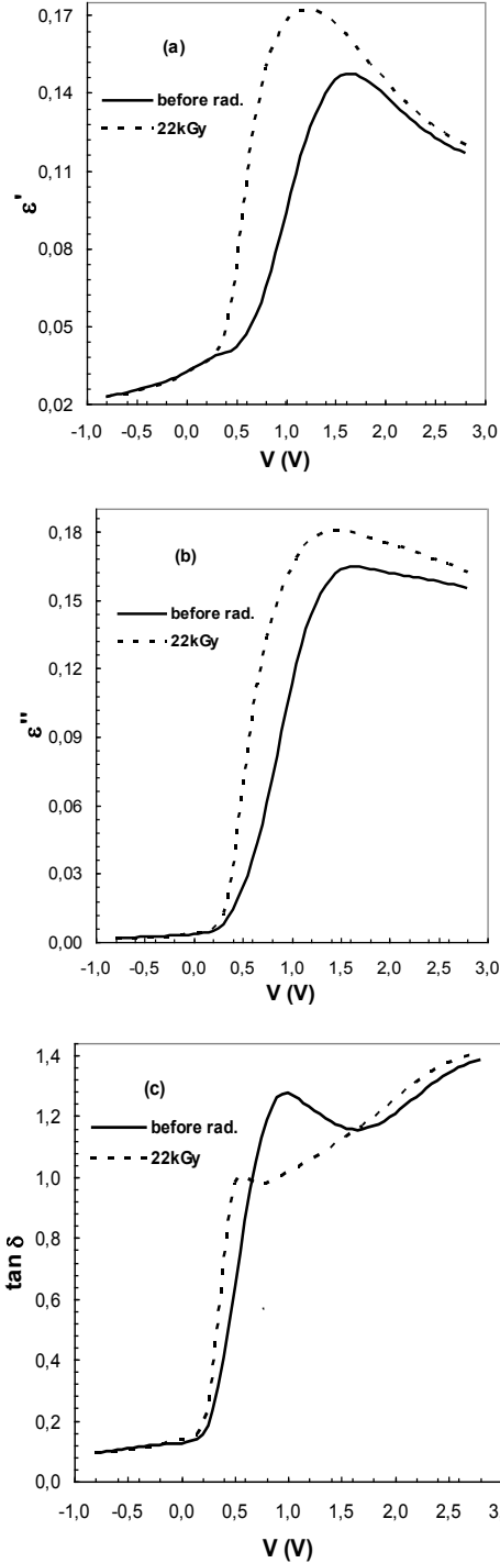
Fig. 1. The voltage dependence of (a) dielectric constant ( \epsilon' ), (b) dielectric loss ( \epsilon'' ) and (c) loss tangent ( \tan\delta ) at 1 MHz and at room temperature for Au/PVA (Co, Zn-doped) n-Si SBD before and after radiation.
