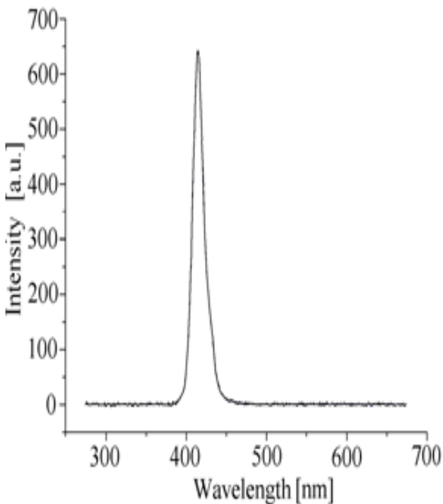
Fig.1 (b). Electroluminescence spectra of InGaN structure
