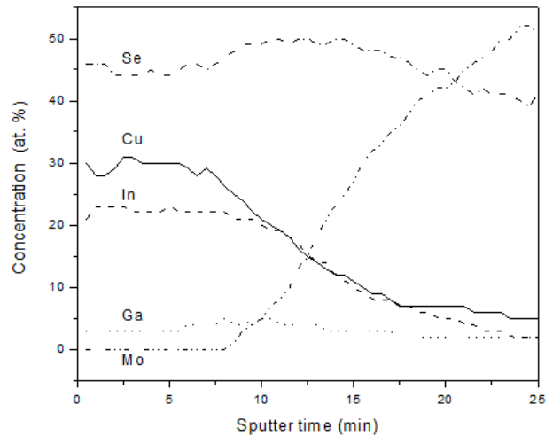
Fig. 2 A AES depth profile of CIGS films on Mo foil (sample 2X118)
