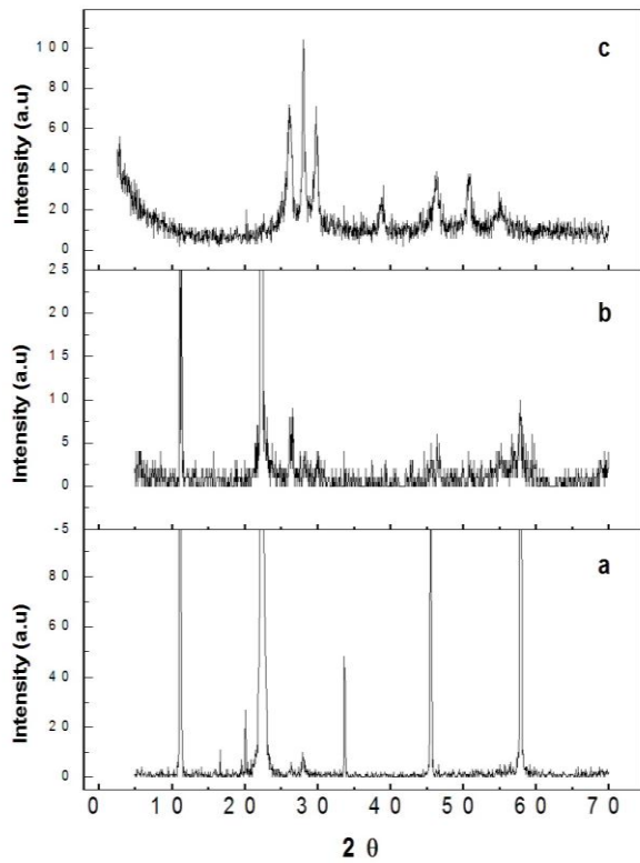
Fig.1. The XRD spectra of a) GaSe substrate, b) MnS film grown on GaSe substrate, c) MnS film grown on glass substrate.
