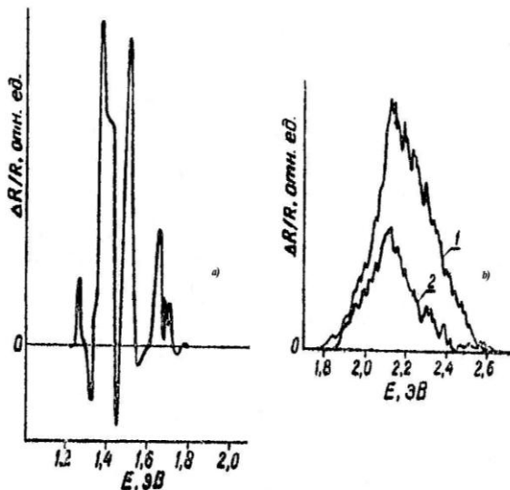
Fig.1. \text{Bi}_2\text{Te}_3 ER spectra obtained in nonpolarized (a) and polarized (b) light where curve 1 is in agreement with polarization \vec{E} \perp C , curve 2 - \vec{E} \parallel C .
