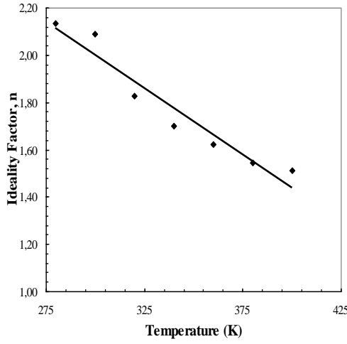
Fig. 3. The variation in the ideality factor with temperature for Au/ PVA (Co, Ni-doped)/n-Si Schottky diodes.
