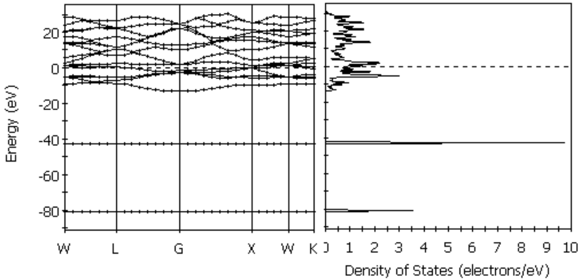
Fig. 5. Calculated band structure of ReB in phase B1
