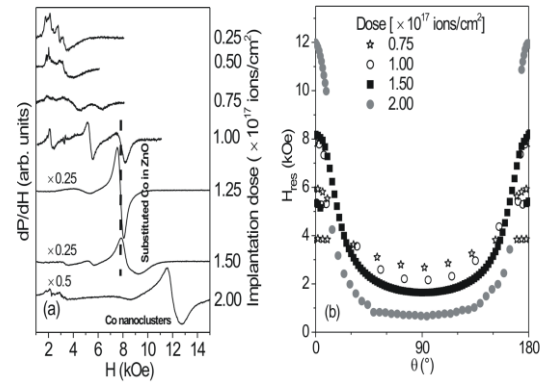
Fig.2 Out-of-plane FMR spectra (a) and the resonance field of FMR signal as a function of polar angle (b) for different cobalt implantation doses.
