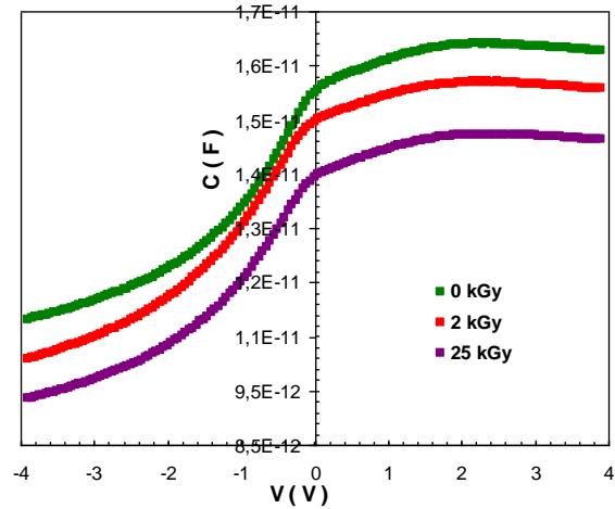
Fig.1. The irradiation dependent curves of the C-V characteristic of the Au/CdTe Schottky barrier diodes.
