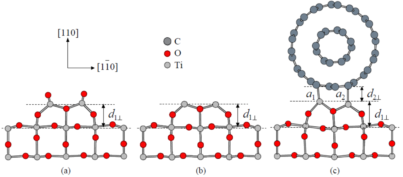
Fig. 1. Schematic side views for the atomic structures of slabs used for (a) rutile \text{TiO}_2(110)-(1 \times 2) ARM surface, (b) oxygen-removed added-row (ORAR) surface, and (c) (3,3)-in-(7,7) DWCNT adsorbed on the ORAR rutile surface.
