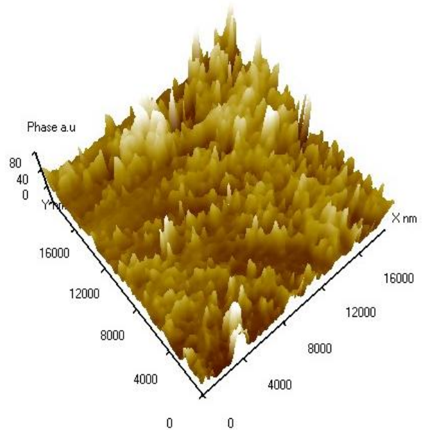
Fig 2. Atomic force microscopy images of Cd 0.1 Zn 0.9 S 0.2 Se 0.8 thin films at deposition potential of U=-0.86 V
