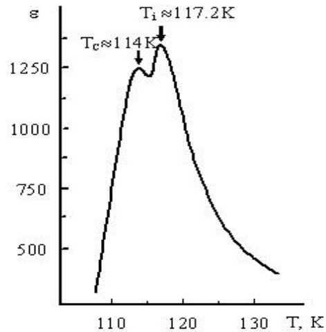
Fig.2. The temperature dependence of the dielectric permittivity of \text{TlGaSe}_2 .
