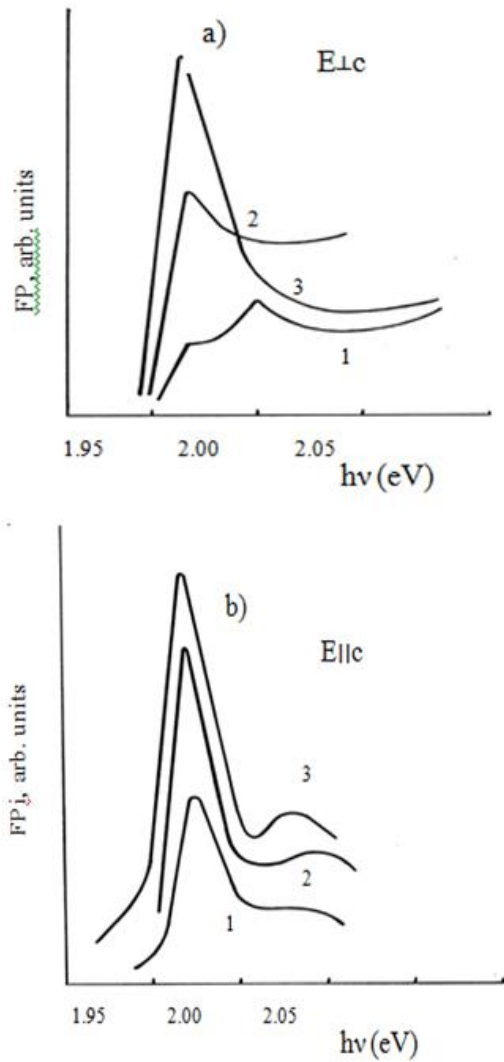
Fig.3. Photoconductivity (FP) spectra of GaSe crystals for two contact configurations: (a) E \perp c , excitation intensities of (1) 0.05, (2) 0.16 and (3) 0.40 \text{MW}/\text{cm}^2 ; (b) E \parallel c , excitation intensities of (1) 0.55, (2) 1.15 and (3) 6.40 \text{MW}/\text{cm}^2 .
