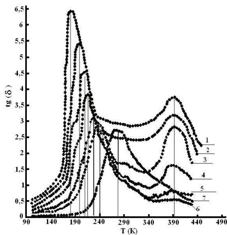
Fig.2. Temperature dependences of the dielectric loss tangent of TlGaTe 2 : 1-0, 2-1, 3-20, 4-50, 5-100, 6-500, 7-1000 kHz.
