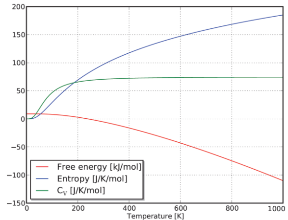
Fig. 6. Temperature dependence of free energy, entropy and heat capacity for NiZrSn in C1b phase
