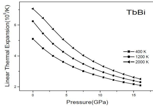
Fig. 10. The thermal expansion verses pressure for TbBi.
