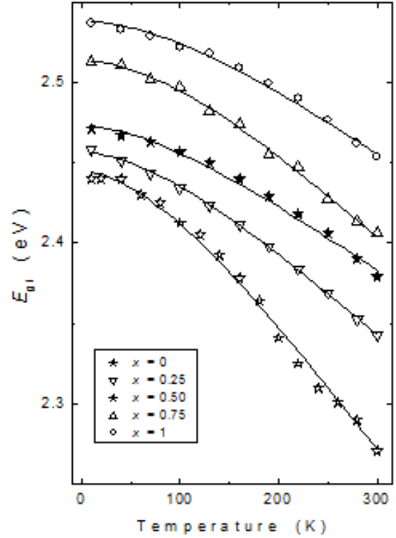
Fig. 4. The indirect band gap energies as a function of temperature for \text{TlGa}_x\text{In}_{1-x}\text{S}_2 mixed crystals. The solid lines represent the fits using equation (4).
