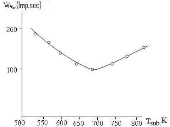
Fig.2. Dependence of swing curve of X-ray diffraction from temperature of substrate of Pb_{1-x}Mn_xSe ( x=0.02 ) epitaxial films.
