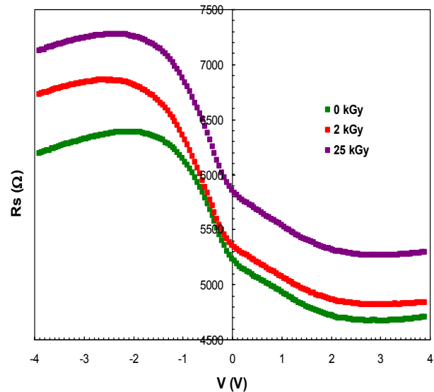
Fig.3. The irradiation dependence of series resistance as a function of bias voltage for the Au/CdTe Schottky barrier diodes.
