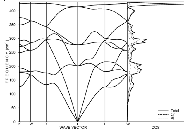
Fig. 2. The calculated phonon dispersions and total and partial density of states for CrAl in B32 structure
