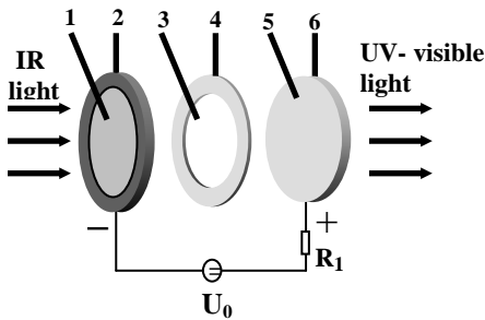
Fig.1. Scheme of the gas discharge cell; 1 – semi-transparent Au - contact; 2 - GaAs cathode; 3 - gas discharge gap; 4 – mica foil; 5 - transparent conductive SnO 2 contact; 6 - flat glass disk.
