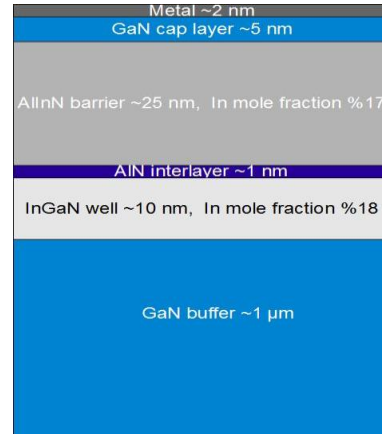
Fig.8. This structure is optimized for high 2DEG carrier density.
