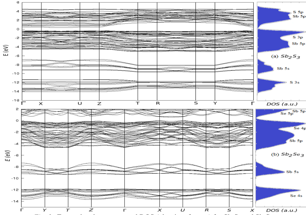
Fig. 1. Energy band structure and DOS ( density of states) for Sb_2S_3 and Sb_2Se_3 .
