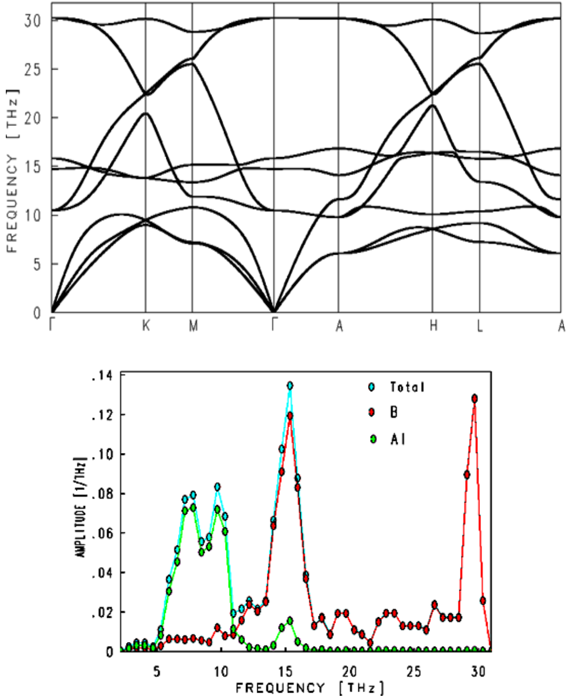
Fig. 1. The calculated phonon dispersion curve, total and partial density of states for AIB 2 .
