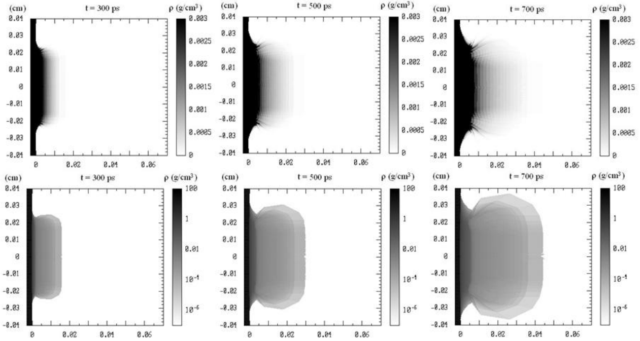
Fig. 2. The result of 2D MULTI hydro code simulation of plasma expansion for a gold target with laser beam parameters corresponded to considered shots: in linear (up) and in logarithmic (down) scales.
