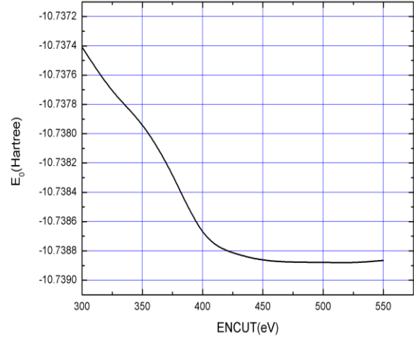
Fig. 1. Total energy versus cut-off energy of NdTe in NaCl(B1)
