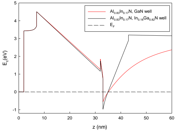
Fig.7. Optimized of the GaN and InGaN wells are band structure.
