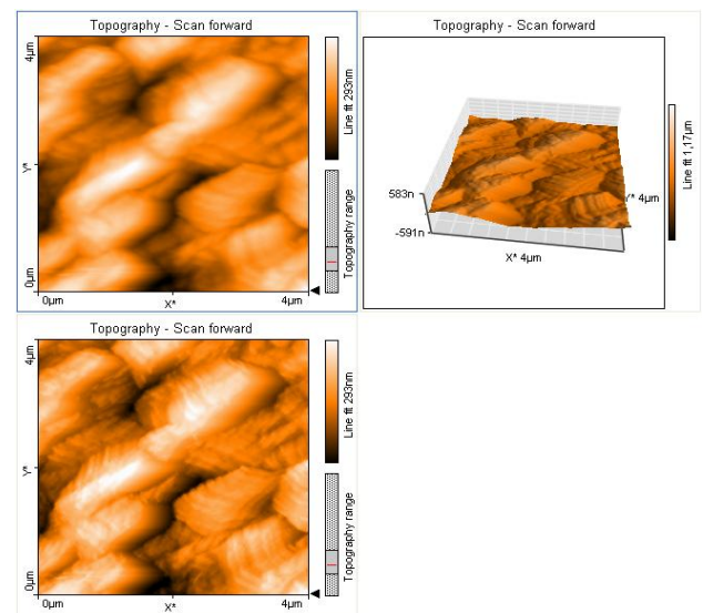
Fig.3. The AFM image of MnS thin film grown on crystalline GaSe substrate.
