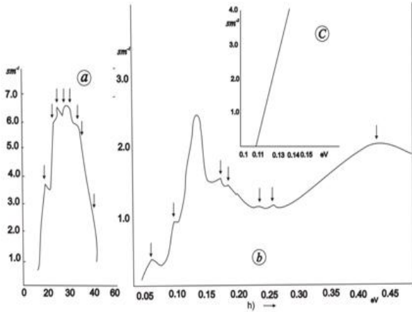
Fig.2. The absorption spectrums of p-CuAgTe a-in range 1.0 ÷ 6.2eV; b-in range 0.05 ÷ 0.50eV; c- \alpha^2 \sim h\nu
