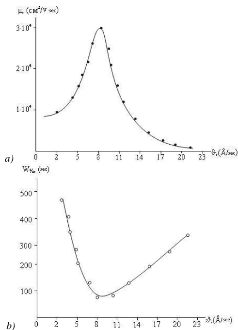
Fig.4. Dependence of mobility of charge carriers (a) and crystal perfection (b) from condensation rate Pb_{1-x}Mn_xTe ( x=0.02 ) epitaxial films.
