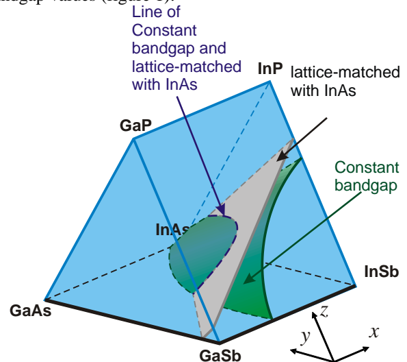
Fig.1. Lattice-matched with InAs and constant bandgap ( E_g=0.37 eV) surfaces in concentration prism of Pentanary Solid Solutions \text{Ga}_{1-x}\text{In}_x\text{As}_y\text{P}_z\text{Sb}_{1-y-z} .
