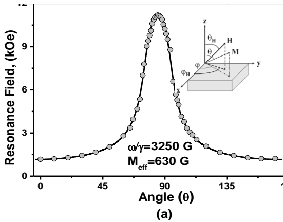
Fig.3. (a) Angular dependence of resonance field at 215 K for the rotation of magnetic field in (100) plane of single crystalline BaTiO 3 . (b) Angular dependence of resonance field at 220 K for the rotation of magnetic field in (001) plane of single crystalline BaTiO 3 . The solid circles show the experimental position of each resonance line in EPR spectra. The solid lines show the simulation of angular behaviors of the resonance lines.
