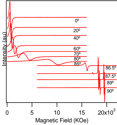
Fig. 4. Angular behavior of experimental SWR spectra taken at room temperature from 1000 Å thickness Co thin film. Magnetic field is parallel to film surface where the spectrum corresponding 0° degree and it is perpendicular to the film surface where angle is 90°.
