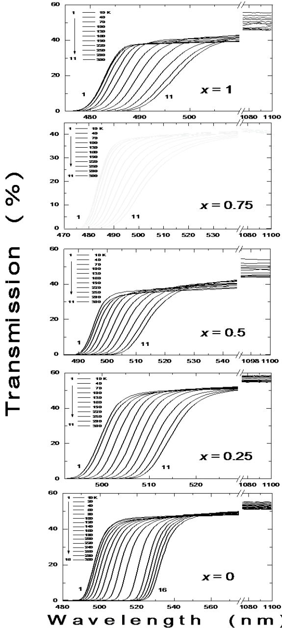
Fig.1. The spectral dependencies of transmission for \text{TlGa}_x\text{In}_{1-x}\text{S}_2 mixed crystals in the temperature range of 10–300 K.
