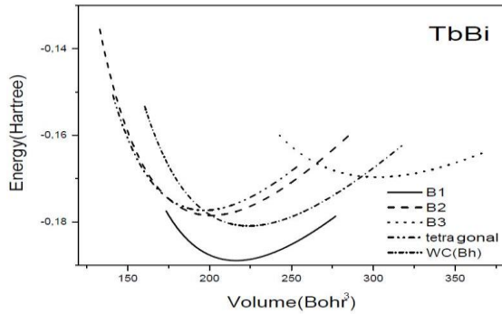
Fig. 1. Total energy versus volume curve of TbBi in B1(NaCl), B2(CsCl), B3(ZB), Bh(WC) and tetragonal phases.
