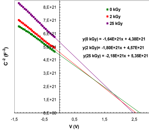
Fig.4. The C -2 -V curves of Au/CdTe Schottky barrier under various irradiation doses at room temperature
