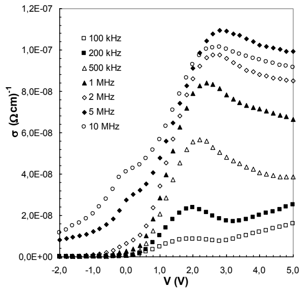
Fig. 3 The variations of ac electrical conductivity ( \sigma_{ac} ) with frequency for Al/SiO 2 /p-Si (MIS) structure at room temperature.
