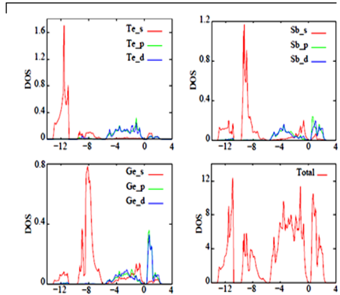
Fig 3. The calculated PDOS and total DOS of \text{Ge}_2\text{Sb}_2\text{Te}_5 compound for model II.
