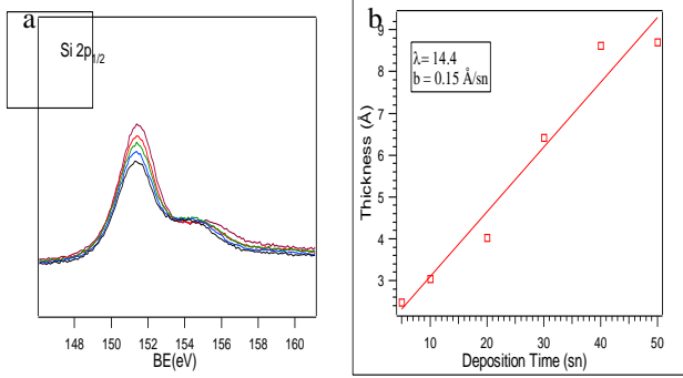
Fig. 1. Since the peaks of Co2s and Si2p 3/2 are at the same place at the photoemission spectrum the Si2p 1/2 attenuation was used to calculate Co coverage for this work. The figure (a) shows the attenuation of the Si2p 1/2 photoemission intensity as a function of Co film thickness. (b) The Co film thickness is calculated from equation 1 using a value of 14.4 Å for the Si2p 1/2 inelastic mean free path.
