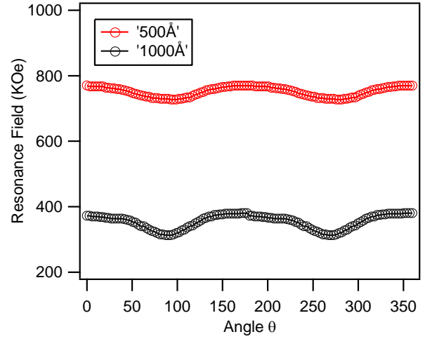
Fig. 7. The angular dependence of the resonance fields for both 500 Å and 1000 Å thickness cobalt films taken at room temperature. Here magnetic field is rotated within the film plane
