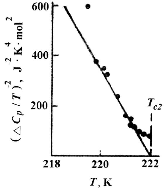
Fig.2. Temperature dependence \left(\frac{\Delta C_p}{T}\right)^2 for TlFeTe 2
