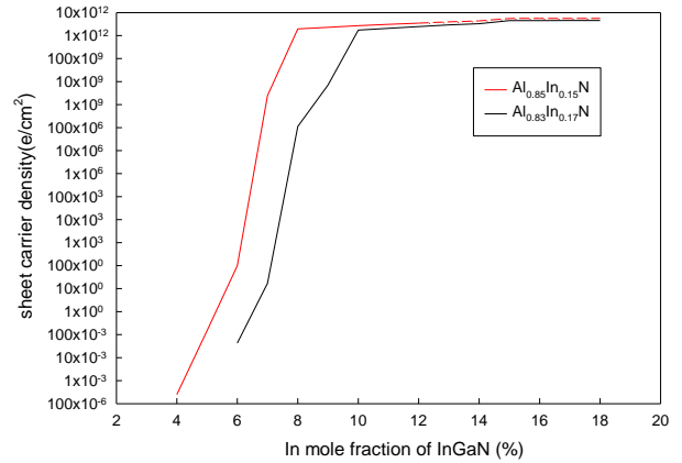
Fig.5. Sheet carrier density for different In mole fractions of InGaN layer in cases Al 0.85 In 0.15 N and Al 0.83 In 0.17 N.
