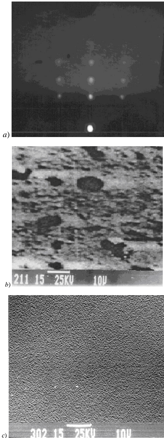
Fig.1. Electronogram (a) and electronmicroscopic pictures (b,c) of Pb_{1-x}Mn_xSe ( x=0.02 ) epitaxial films: b) without additional Se vapor source, c) with additional Se vapor source.
