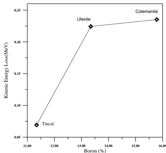
Fig.3. Kinetic Energy Losses as a Function of Boron Percentages
