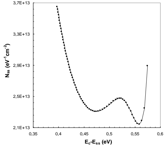
Fig 5. The N_{ss} plot of Au/SrTiO 3 /n-Si (MFS) SBD.
