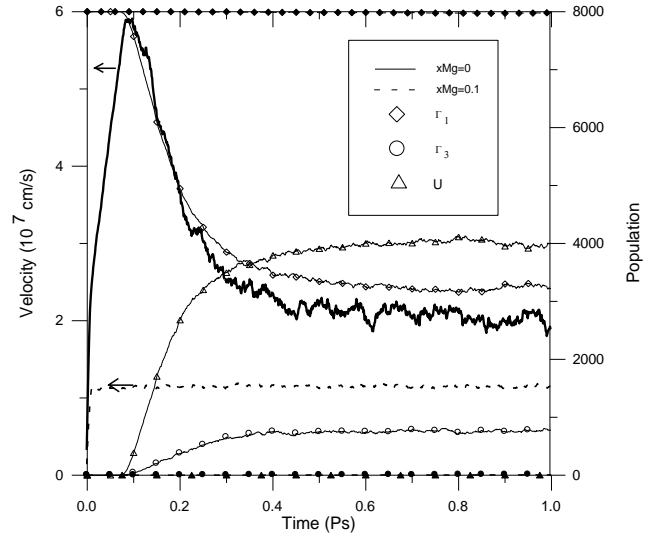
Fig.4 The drift velocity in ZnO and in Zn_{1-x}Mg_xO for the case of x=0.1 and the occupancies of \Gamma_1 , \Gamma_3 , U valleys at an applied field of F_x= 600 kV/cm at room temperature.
