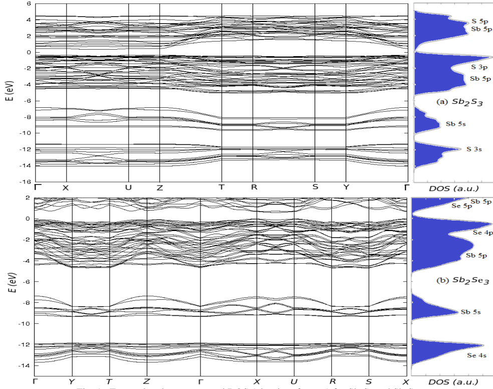
Fig. 1. Energy band structure and DOS ( density of states) for Sb_2S_3 and Sb_2Se_3 .
