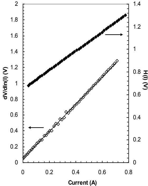
Fig.. 2. Plots of d(V)/d(\ln I) - I and H(I) - I of the Au/n-GaP Schottky barrier diode in darkness.
