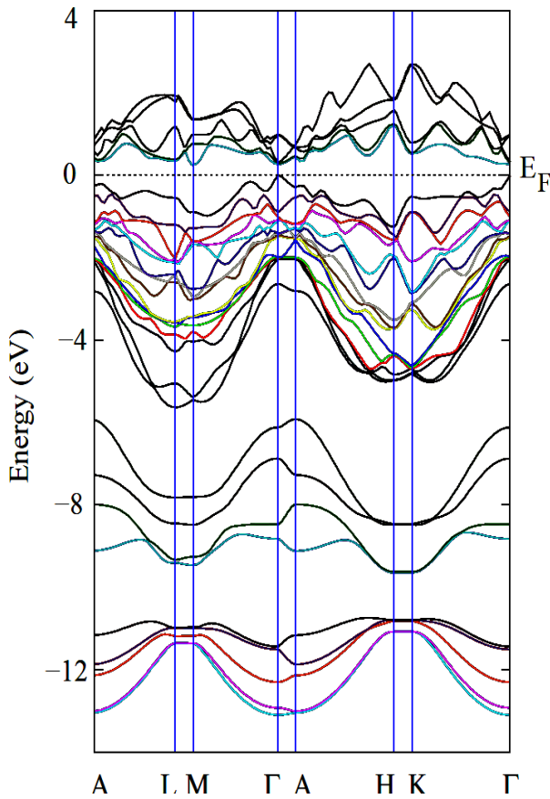
Fig2. Electronic band structure of \text{Ge}_2\text{Sb}_2\text{Te}_5 compound for model II.
