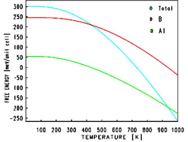
Fig. 3. Temperature dependence of free energy for for \text{AlB}_2
