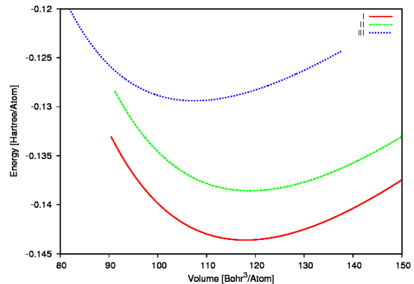
Fig. 1. The Energy-Volume curves of LiAlSi compounds.
