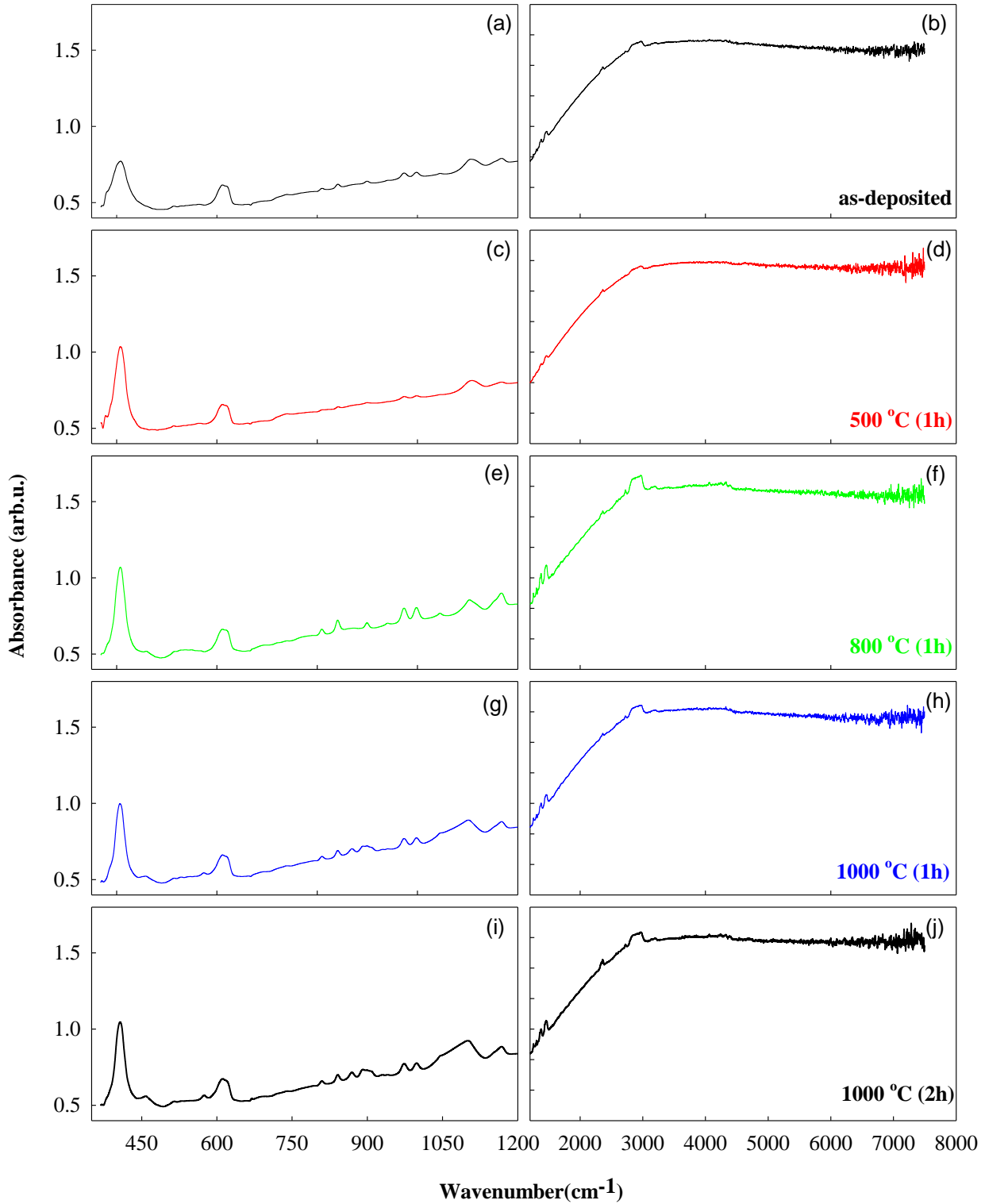
Fig.2. The FTIR spectra of the sample (a, c, e, g, i) in range of 375-1200 \text{cm}^{-1} (b, d, f, h, j) in range of 1200-8000 \text{cm}^{-1} .
