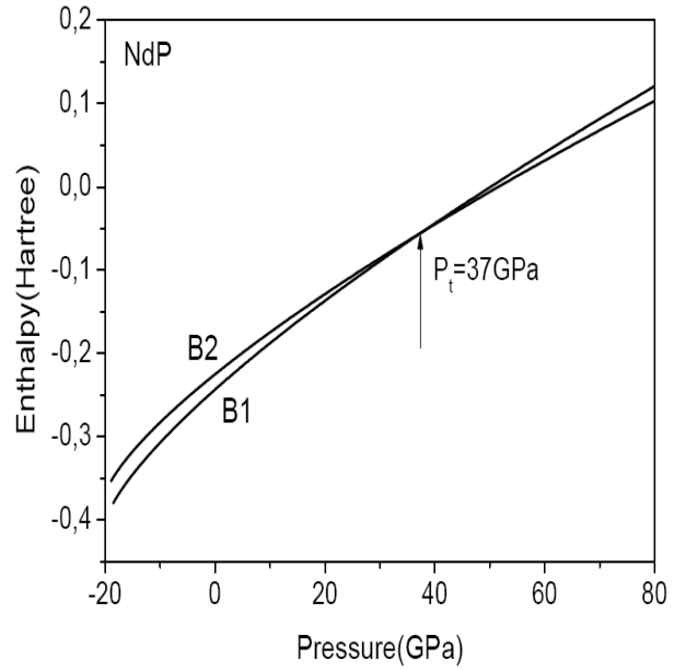
Fig. 3. Estimation of phase transition pressure from B1 to B2 of NdP
