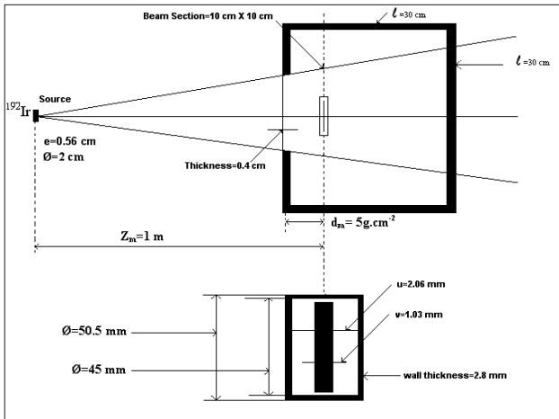
Fig. 1. Experimental arrangement used at the SSDL for measuring the adsorbed dose in the water phantom, and schematic view of the cavity ionization chamber [3].
