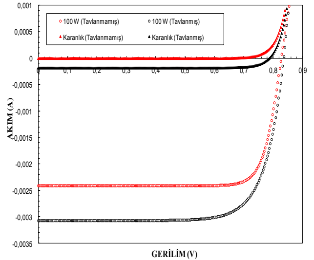
Fig.3. The photovoltaic forward bias dark and under AM1.5G illumination current-voltage characteristics of the as deposited and annealed InGaAs/GaAs solar cells.
