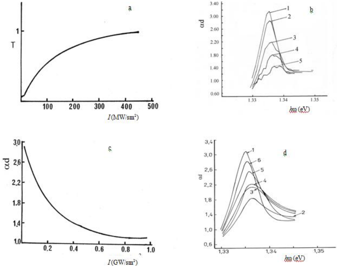
Fig.1. (a) Dependence of the transmission coefficient on the excitation intensity in InSe (in the case of resonant excitation of exciton, h\nu=1,327\text{eV} ) at 77 K; (b) Absorption spectra of InSe for different excitation intensity I_{\text{pump}} ( \text{MW}/\text{cm}^2 ): 1 - 0, 2-12, 3-60, 4-250, 5-600 (time delay between the probe and pump pulses \Delta t=0 ) at T=4,2\text{ K} ; (c) Dependence of the optical density on the excitation intensity ( h\nu_{\text{pump}} = 2,34\text{eV} , h\nu_{\text{probe}} = 1,336\text{eV} , \Delta t = 0 ) at T=4,2\text{ K} ; (d) Absorption spectra of InSe for different time delays between the probe and pump pulses: 1 - I_{\text{pump}}=0 , 2 - \Delta t = 24\text{ps} , 3 - \Delta t = 98\text{ps} , 4 - \Delta t = 297\text{ps} , 5- \Delta t = 660\text{ps} , 6- \Delta t = 910\text{ps} , I_{\text{pump}} = 600\text{ MW}/\text{cm}^2 , h\nu_{\text{pump}} = 2,34\text{eV} , T=4,2\text{ K} .
