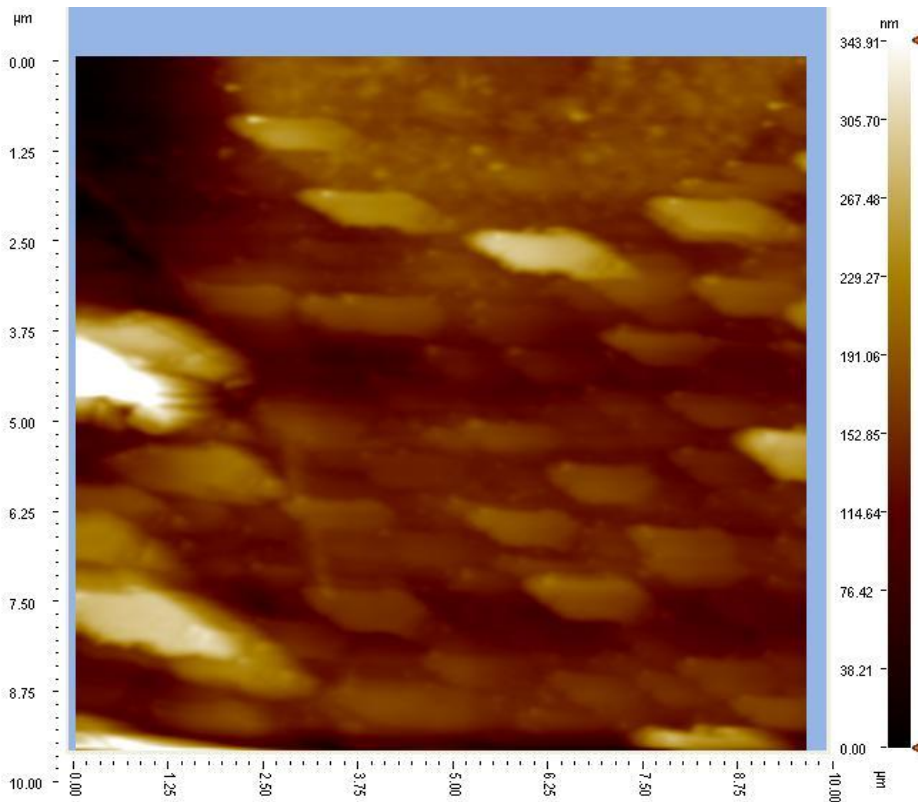
Fig. 3-a AFM image of iron oxide nano thin films at 500 °C.
