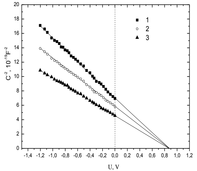
Fig. 4. Capacitance-voltage dependences for heterostructures for p-GaAs/n-Cd 1-x Zn x S 1-y Se y heterojunctions without (1) and after thermal annealing (2, 3). 2- 200 o C for 15 min; 3- 300 o C, for 15 min
