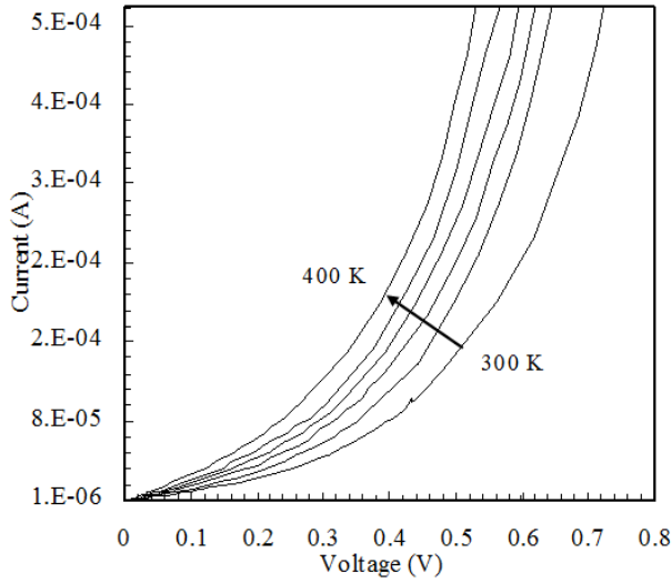
Fig.1. The I - V characteristics of the Au/n-GaAs Schottky diode
