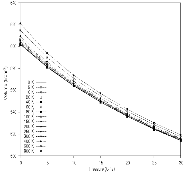
Fig. 1. The variation of volume with the pressure of PtBi for various temperatures.
