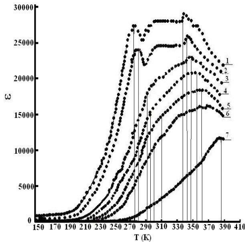
Fig.1. Temperature dependences of the permittivity of TlGaTe 2 : 1-0, 2-1, 3-20, 4-50, 5-100, 6-500, 7-1000 kHz.
