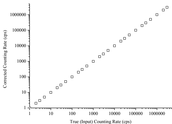
Fig. 5 Variation of the corrected rate n as a function of the true rate n_0 for decaying source model of dead time losses
