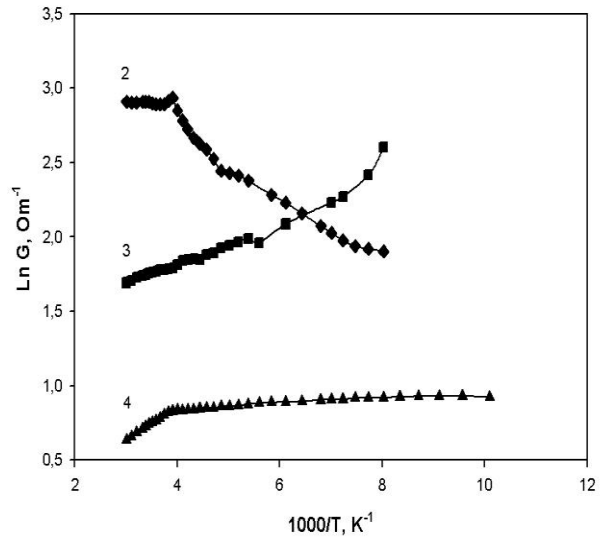
Fig. 4 Temperature dependences of resistivity for the p- Zn_{1-x}Cd_xMn_{0.06}GeAs_2 (№2), curve 2; p- Zn_{1-x}Cd_xMn_{0.1}GeAs_2 (№3), curve 3; and p- Zn_{1-x}Cd_xMn_{0.14}GeAs_2 (№4), curve 4.
