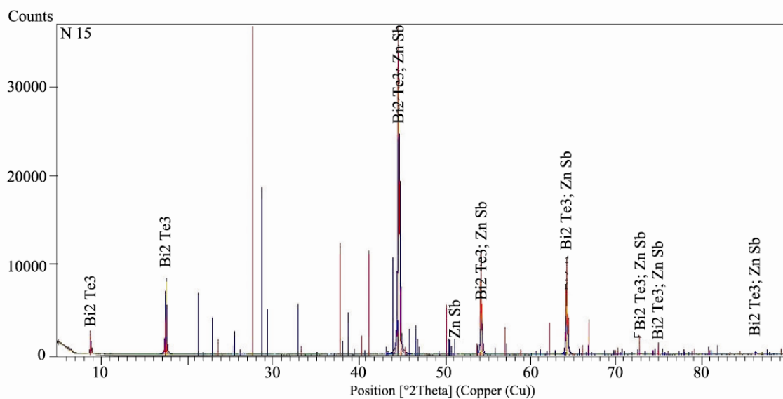
Fig.1(a, b, c) X-ray diffraction patterns A_2^V B_3^{VI} <impurity> spelled systems. a). Bi_2Te_3<Cu> , b) Bi_2Te_3<Ni> , c) Sb_2Te_3<ZnSb> .
