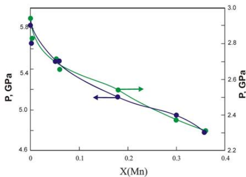
Fig.2. Dependence of position of point of phase transition from percent content of doping element (Mn) at pressure rise – left scale, dark symbols and at pressure fall – right scale, light symbols.
