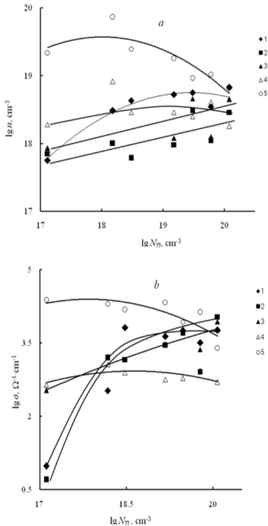
Fig.3. Dependence of concentration of charge carriers (a) and electrical conductivity (b) on concentration of thallium in PbTe single crystals at \sim 77 K. Curves 1-5 refers to the sample unannealed and samples annealed at 473, 573, 673, 873 K respectively.
