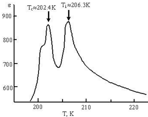
Fig.1. The temperature dependence of the dielectric permittivity of \text{TlInS}_2 .
