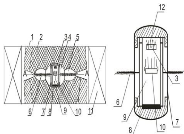
Fig. 1 A device for measuring of baric dependence parameters of solids at high hydrostatic pressure up to 10 GPa: 1 – ring of support; 2 – insert from WC-6M; 3 – manganin pressure pickup; 4 – catlinite insert; 5 – catlinite ring; 6 – electrical leads; 7 – teflon capsule; 8 – copper lid; 9 – cooper lids; 10 – sample; 11 – solenoid.
