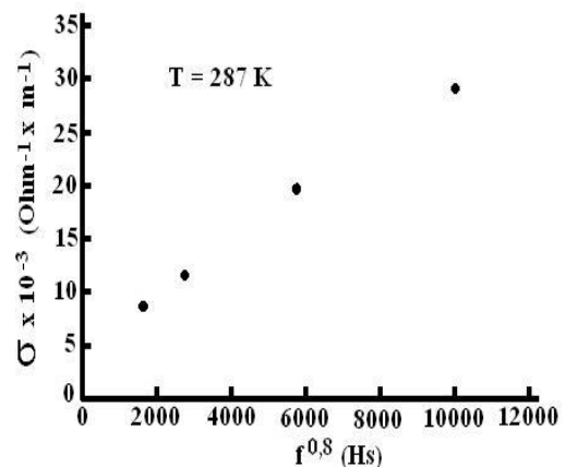
Fig.4. Frequency dependence conductivity of TlGaTe 2 .
