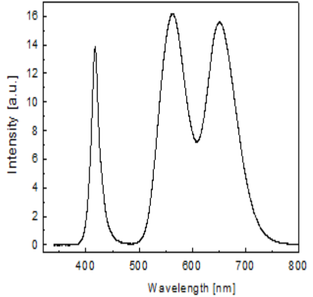
Fig.2. Emission spectrum of InGaN chip with phosphor
