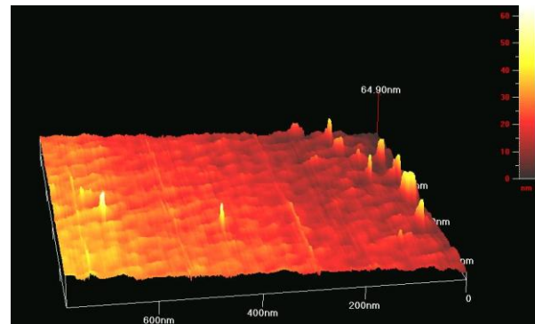
Fig. 5. AFM images (700 nm * 700 nm) of ZrO 2 coated lenses
