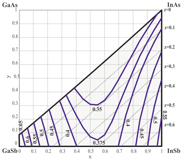
Fig.2. Projections on composition square of the intersection lines between lattice-matched with InAs and constant bandgap surfaces for pentenary solid solutions Ga_{1-x}In_xAs_yP_zSb_{1-y-z} . Numbers indicate E_g values.
