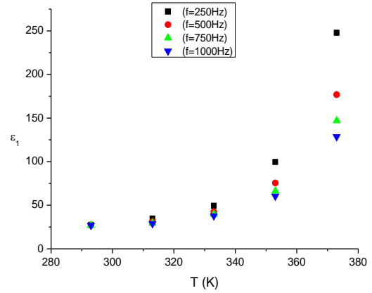
Fig.3. Temperature dependence of the dielectric constant \epsilon_1 , of TlSbS 2 thin films at different frequencies. Film Thickness: 4090 A°
