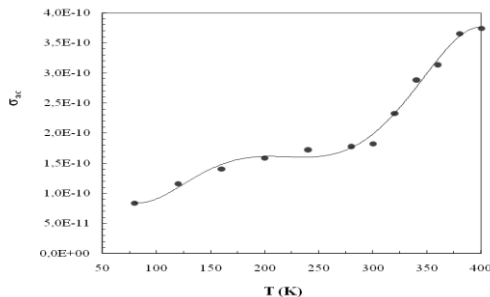
Fig. 3. Temperature dependence of ac electrical conductivity ( \sigma_{ac} ) of Au/ PVA(Co, Ni-doped)/n-Si structure.
