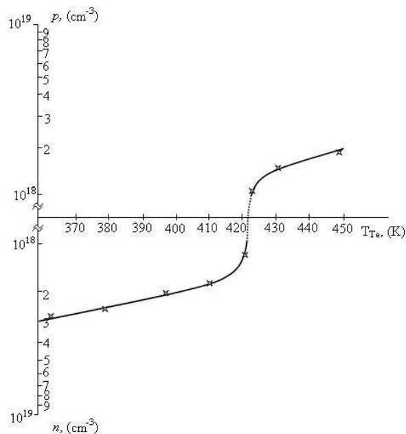
Fig.3. Dependence of concentration of charge carriers from temperature of an additional compensating Te vapor source in PbSe_{1-x}Te_x ( x=0.2 ) epitaxial films.
