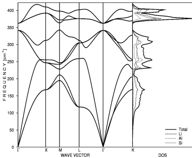
Fig. 2. The calculated phonon dispersions and total and partial density of states for arrangement I.
