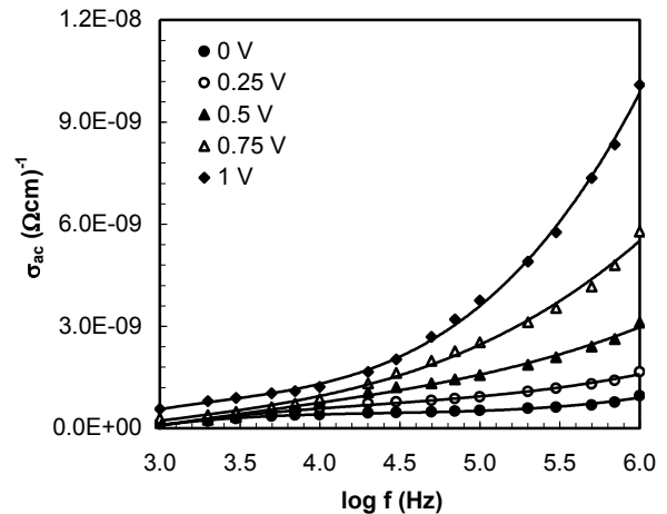
Fig. 3. Frequency dependence of ac electrical conductivity ( \sigma_{ac} ) for various applied voltage of Au/n-GaAs (MS) structure.
