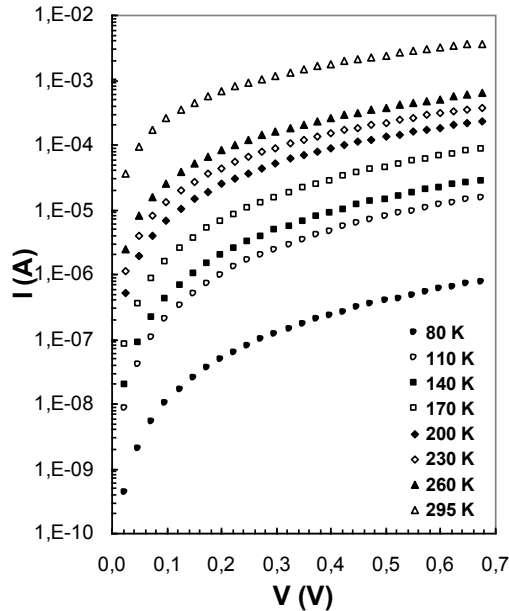
Fig. 2. The experimental forward bias I - V characteristics of the n- GaAs structure at various temperatures.
