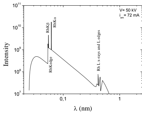
Fig. 2. X-ray tube spectrum calculated according to Ebel Algorithm [13].
