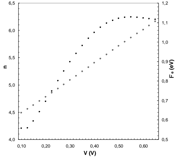
Fig 3. The voltage dependent n and \Phi_e plots of Au/SrTiO 3 /n-Si (MFS) SBD.
