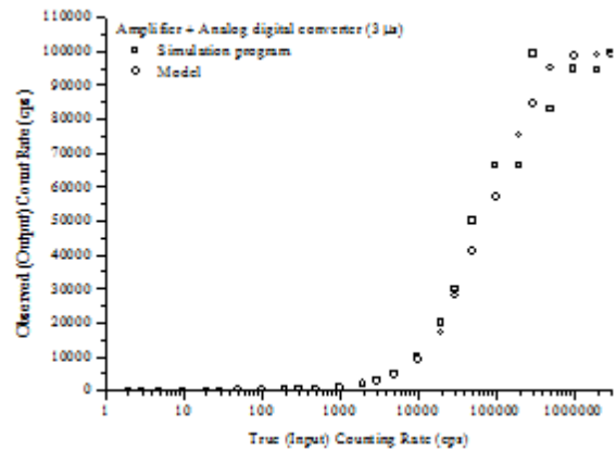
Fig. 4 For 3 \mu\text{s} peaking time of the amplifier, comparing proposed model in this study with simulation program in both the amplifier and the ADC case
