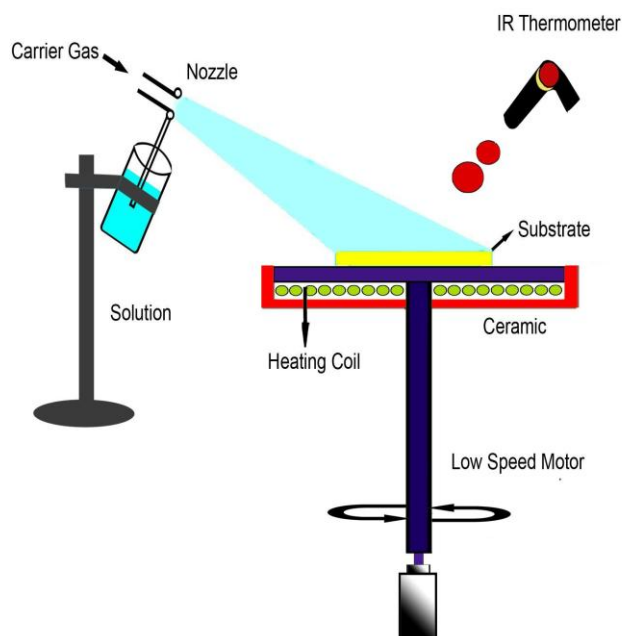
Fig. 1. Schematic diagram of chemical spray pyrolysis setup.
