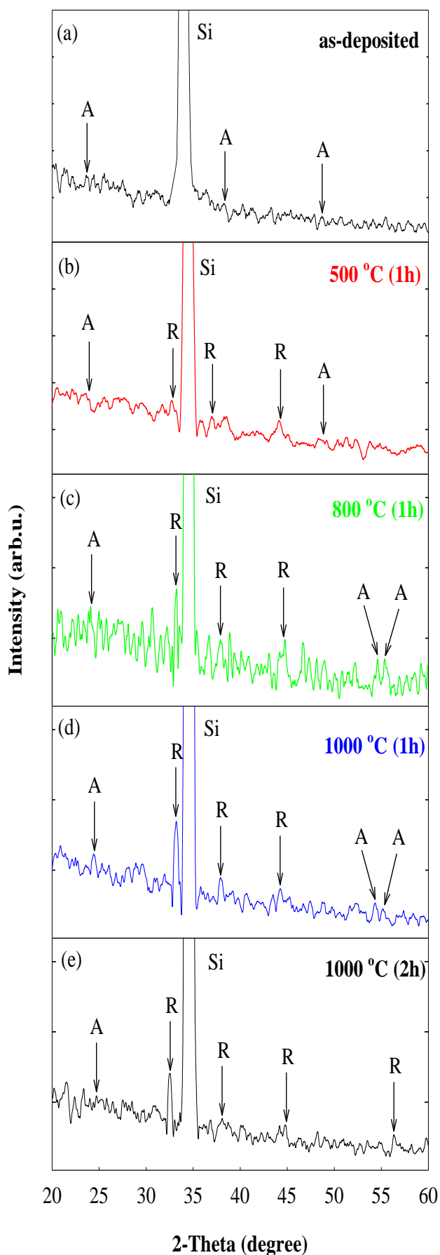
Fig.1. XRD pattern of TiO 2 thin film at different annealing temperatures.
