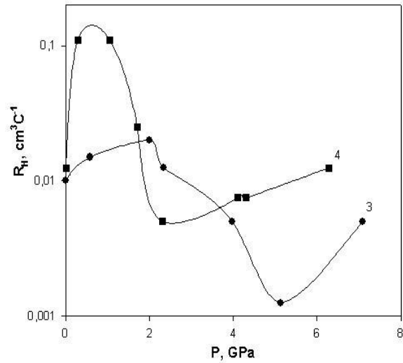
Fig. 3 Pressure dependences of Hall coefficient for the p- Zn_{1-x}Cd_xMn_{0.06}GeAs_2 (№2) and p- Zn_{1-x}Cd_xMn_{0.1}GeAs_2 (№3).
