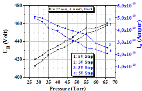
Fig.3. Dependence of U_B and minimum current I_B on ramping voltage k ( 3 \text{ V s}^{-1} and 5 \text{ V s}^{-1} ) for different gas pressures. System parameters: D = 22 \text{ mm} , d = 445 \text{ }\mu\text{m} and in darkness.
