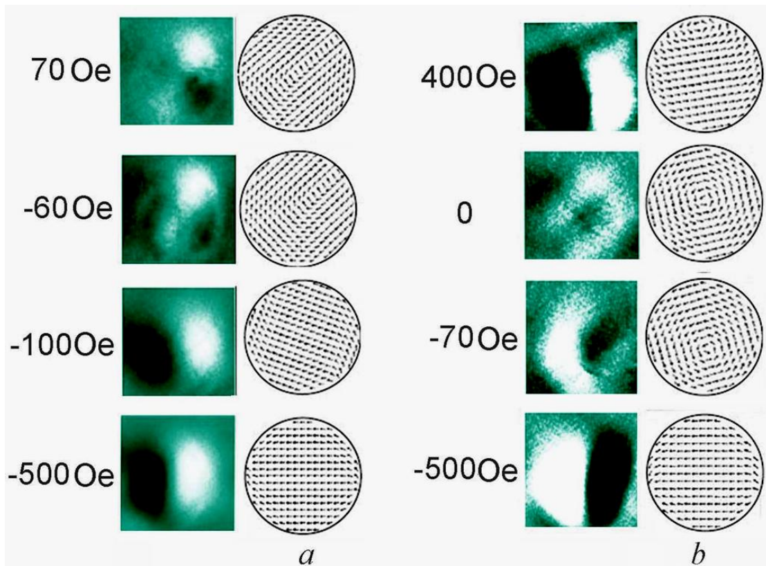
Fig.2 MCM image of micropoint magnetic structure and computer modeling of spin distribution of micropoint array for situations a) l=3d ; b) l=2d in external magnetic fields.
