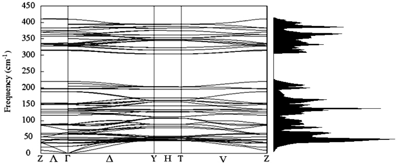
Figure 3. Calculated phonon spectra and phonon density of states (inset to the right side) of TlGaS 2 .
