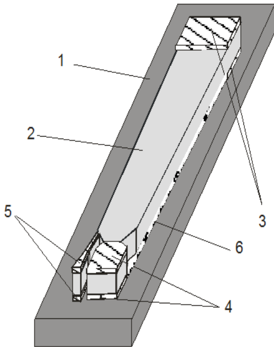
Fig. 2. General view of the photosensitive element of the proposed sensor. 1 - substrate, 2 - crystal Cd 0.2 Hg 0.8 Te; 3 and 4 - current contacts, 5 - reads the contact, 6 - glue.
