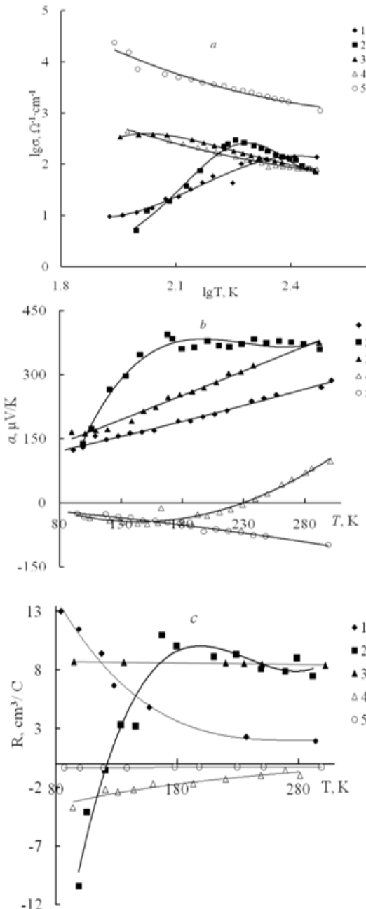
Fig.1. Temperature dependence of electrical conductivity (a), thermo-e.m.f (b) and Hall factor (c) of PbTe single crystals. Curves 1-5 refers to the sample unannealed and samples annealed at 473, 573, 673, 873 K respectively.
