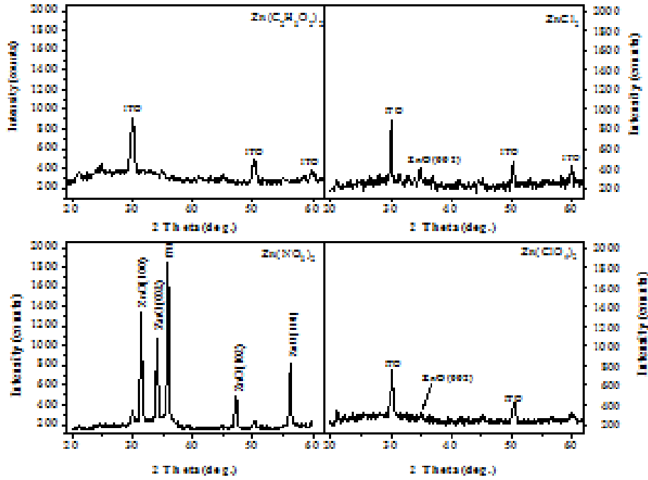
Fig. 1. XRD measurements of the ZnO thin films grown in DI water.
