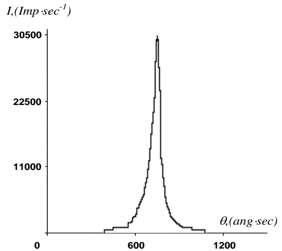
Fig.3. Swing curve of X-ray diffraction of Pb_{1-x}Mn_xSe ( x=0.02 ) epitaxial films.
