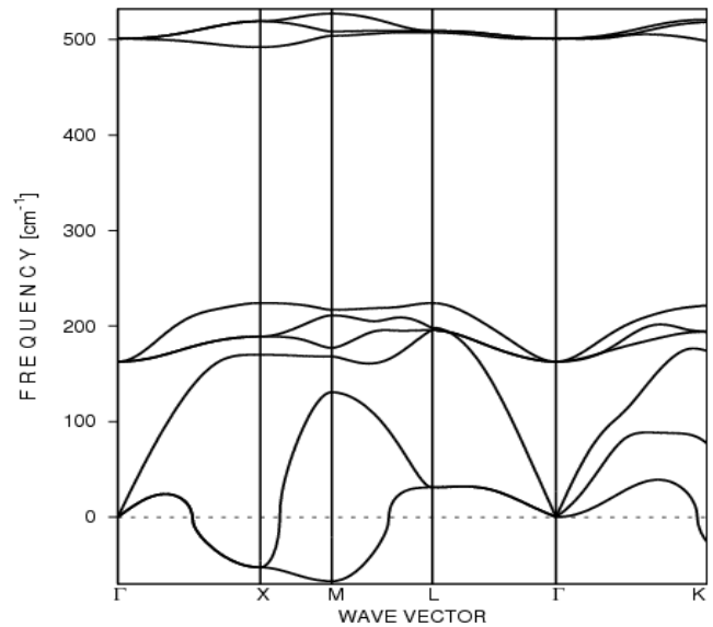
Fig. 4. The calculated phonon dispersion curves for arrangement III.
