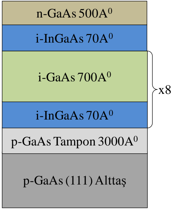
Fig.1. The schematic diagram of the MBE grown InGaAs/GaAs QWSC
