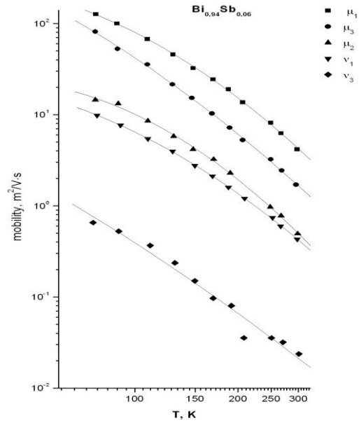
Fig.4. Temperature dependence of the charge carriers' mobilities.
