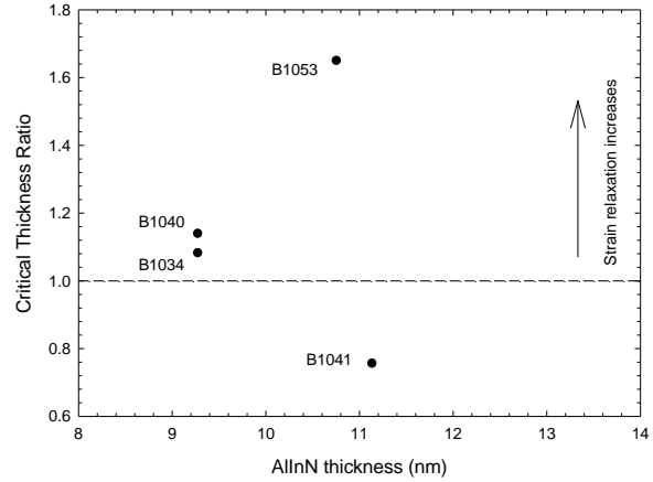
Fig. 3. The critical thickness ratio according to InAlN thickness of investigated samples.
