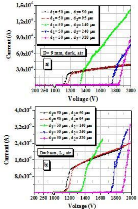
Fig 3. CVC of the modified ionization cell as a function of d in coupled air plasma a) under dark, b) under moderate illumination intensity L_2 .
