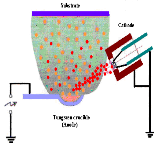
Fig. 1. Schematic representation of TVA's plasma
