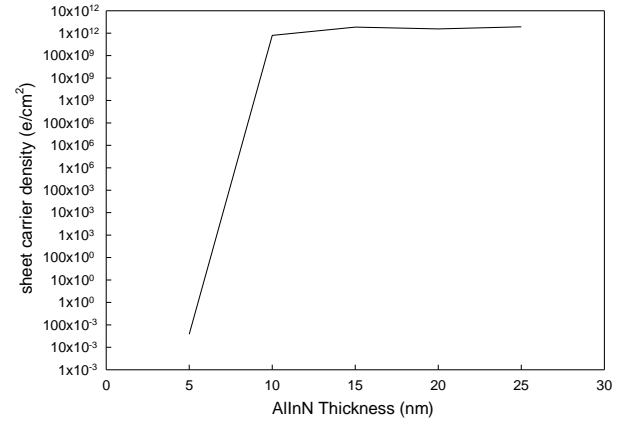
Fig 1. AlInN barrier layer thickness dependence of carrier density.
