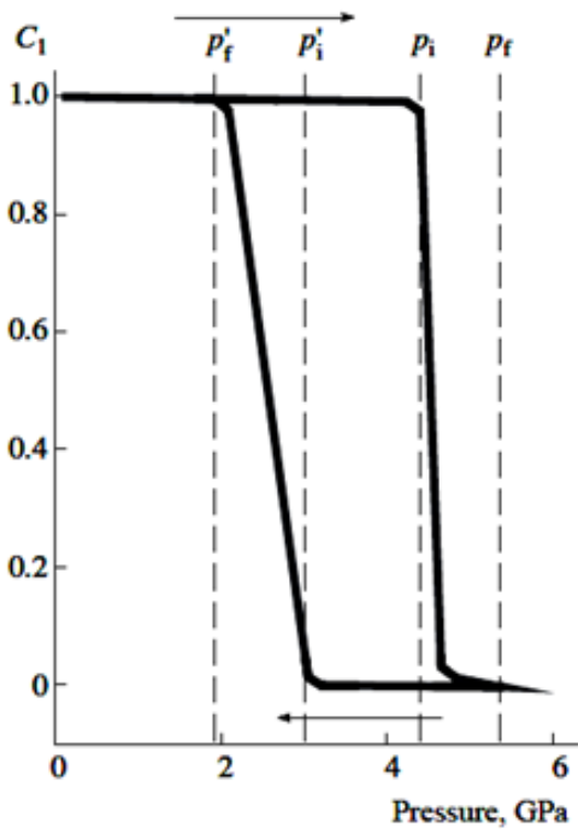
Fig.2. Volume fraction of phase 1 as a function of pressure for p\text{-}Cd_{1-x}Mn_xGeAs_2 with x = 0.18 .
