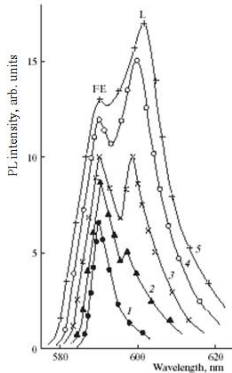
Fig. 4. Photoluminescence (PL) spectra of GaSe crystals at different excitation intensities I_0 ( \text{MW} \cdot \text{cm}^{-2} ): 1- 0.12, 2- 1.01, 3- 4.02, 4- 6.03 and 5- 12. T=80 K.
