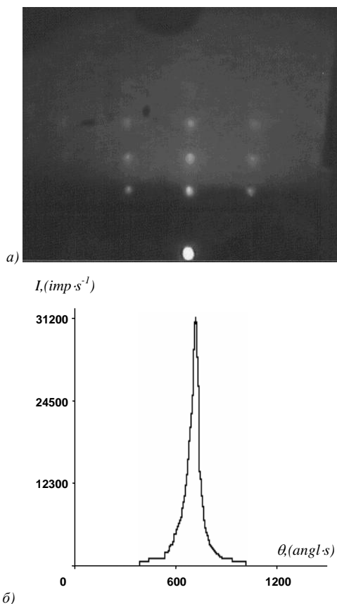
Fig.1. Electron-diffraction pattern (a) and swing curve of X-ray diffraction (b) of PbSe_{1-x}Te_x ( x=0.2 ) epitaxial films.
