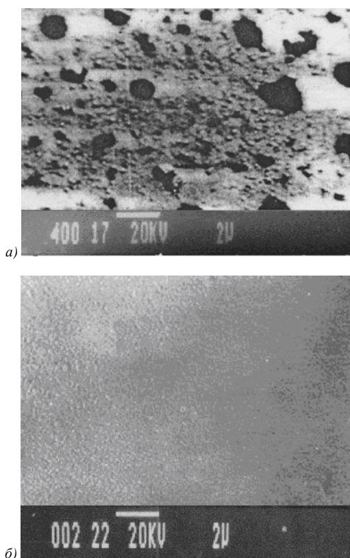
Fig.2. Electron microscopic picture of PbSe_{1-x}Te_x ( x=0.2 ) epitaxial films a) without additional compensation
