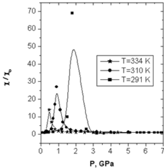
Fig.4 Dependence of relative magnetic susceptibility from pressure for pressure for various temperatures
