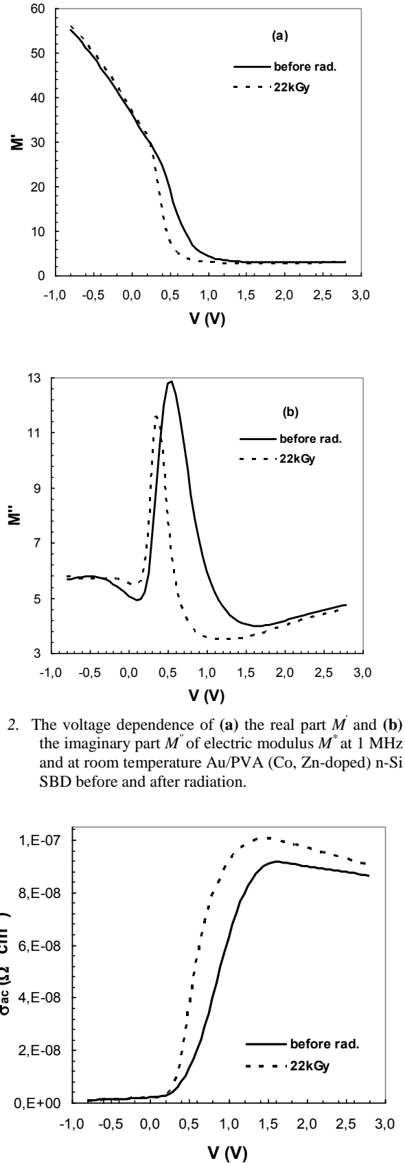
Fig. 3. The variation of the ac electrical conductivity \sigma_{ac} with applied bias for Au/PVA (Co, Zn-doped) n-Si SBD before and after radiation.
