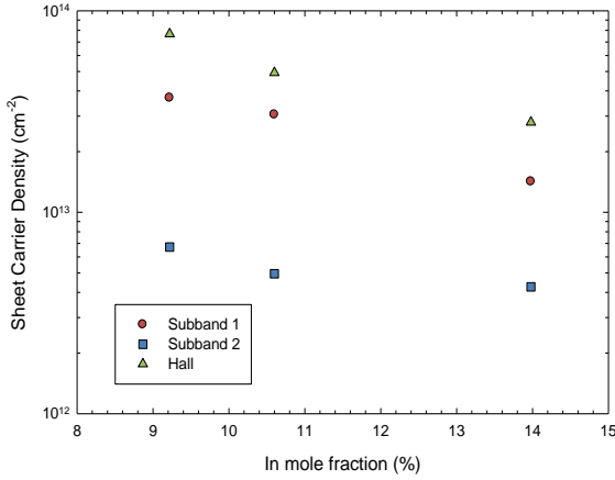
Fig. 4 In mole fraction dependent sheet carrier density for hall, first and second subband.
