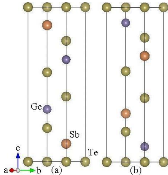
Fig.1. Schematic side views of \text{Ge}_2\text{Sb}_2\text{Te}_5 compound for (a) model I and (b) model II.
