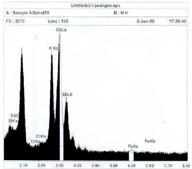
Fig. 3 EDS spectrum of the epilayers
