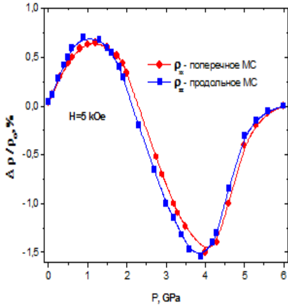
Fig.7 Dependence of cross (circles) and longitudinal (squares) magnetic resistivity from pressure
