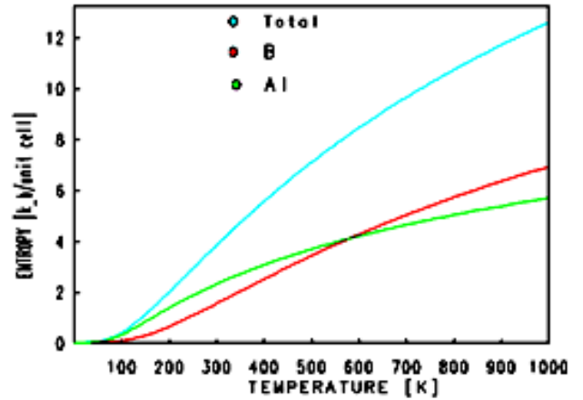
Fig. 4. Temperature dependence of entropy for for \text{AlB}_2
