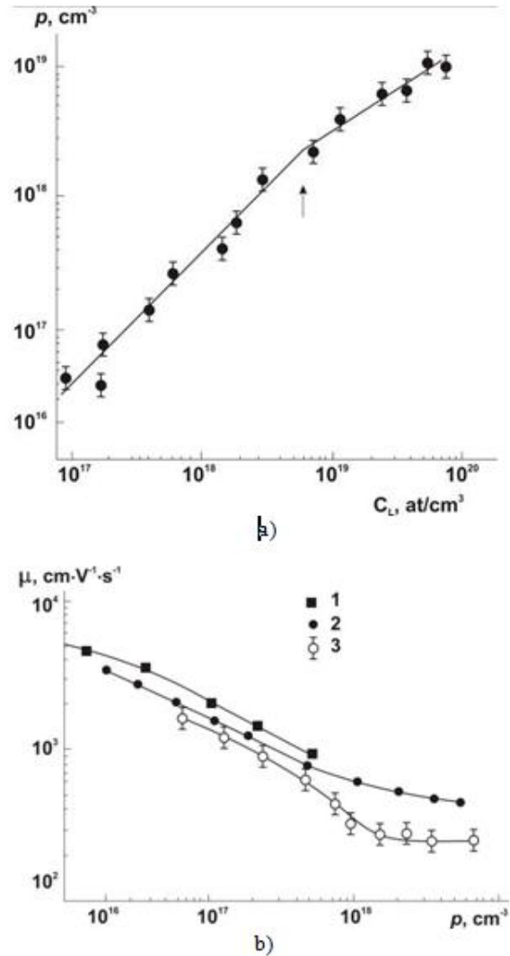
Fig.1 a) Dependence of holes concentration on Cd composition at liquid phase at 77K; b) Dependence of hole mobility on holes concentration (77K).
