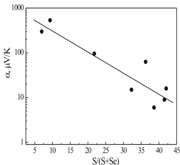
Fig.7. The thermopower dependence on the S/(S+Se) ratio for CIGSS films.
