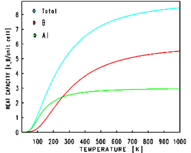
Fig. 5. Temperature dependence of heat capacity for for \text{AlB}_2
