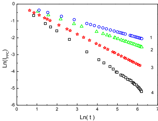
Fig. 4 The PPC decay curves in logarithmic scale for CdTe(Sb) in the temperature range 4 for temperatures T = 225 K (1), 245 K (2), 275 K (3), 295 K (4)
