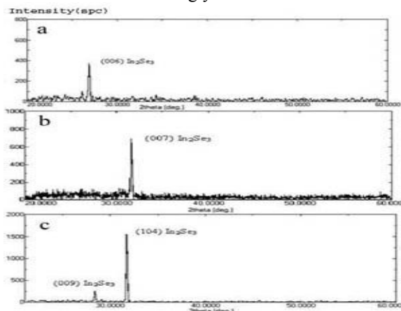
Fig1. X-ray diffraction spectrums of In_2Se_3 thin films prepared by sol-gel method.
