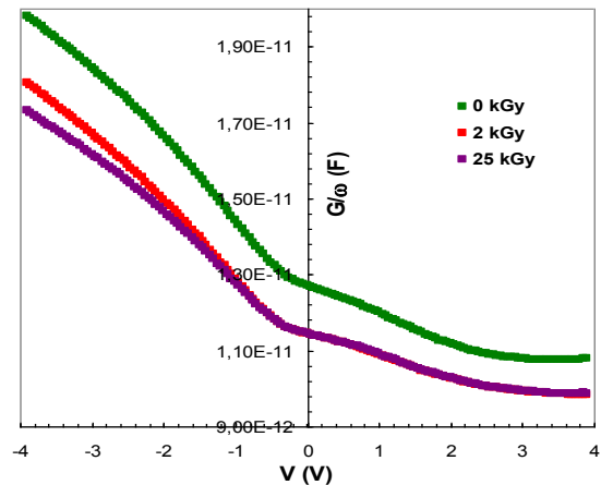
Fig.2. The irradiation dependent curves of G/ \omega -V characteristics of the Au/CdTe Schottky barrier diodes.
