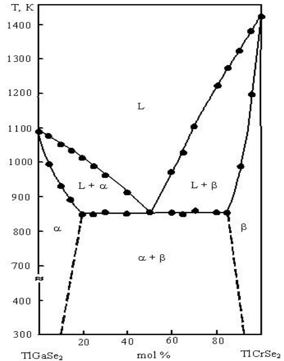
Fig.7. \text{TlGaSe}_2 - \text{TlCrSe}_2 system state diagram.
