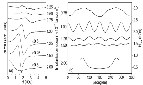
Fig. 1 FMR spectra at the in-plane geometry (a) and the angular dependence of the resonance fields (b) for different cobalt implantation doses.
