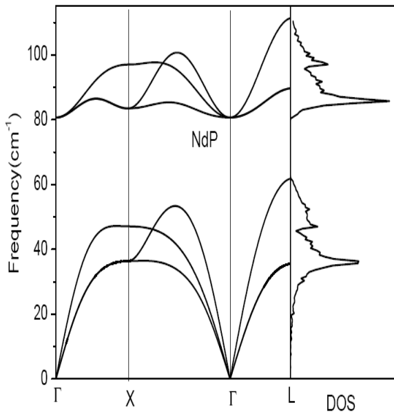
Fig. 6. Calculated phonon dispersions and total density of states for NdP in B1 structure
