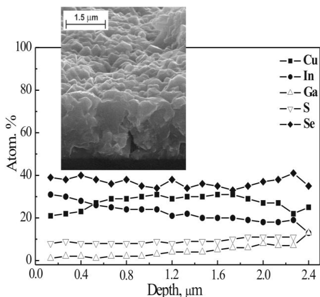
Fig. 1. SEM cross-section image and AES profiles of CIGSS layer grown under 400 °C
