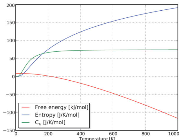
Fig. 7. Temperature dependence of free energy, entropy and heat capacity for NiHfSn in C1_b phase.
