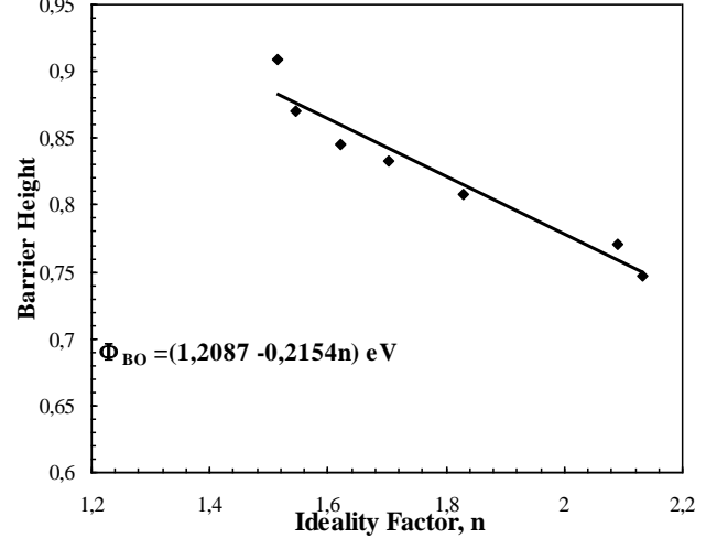
Fig. 5. Linear variation of apparent barrier height vs. ideality factors.
