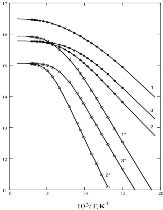
Fig. 1. Temperature dependences of the free-hole concentration for the (1-3) Ge<Cu, Al, Sb> and (1*-3*) Ge 0,88 Si 0,12 <Cu, Al, Sb> samples: (1,1*) after doping samples with copper at 1145 and 1170 K, respectively; (2,2*) after heat treatments at 1050 and 1070 K, respectively; and (3,3*) after annealing at 550 K for 20 h. The solid lines are the theoretical results that are in the best agreement with the experimental data; curves 1, 1*, 3, and 3* were calculated taking into account the effect of the partially compensated first Cu s level: E_{\text{Cu}1} = E_v + 40 meV in Ge and E_{\text{Cu}1} = E_v + 72 meV in Ge 0,88 Si 0,12 [18]; curves 2 and 2* were obtained taking into account two active levels: the first Cu s acceptor level and the additional acceptor center with E_k = E_v + 52 meV in Ge and E_k = E_v + 91 meV in Ge 0,88 Si 0,12 .
