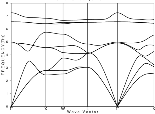
Fig. 3. Phonon dispersion curves with LO-TO along first Brillouin zone for NiHfSn compound.
