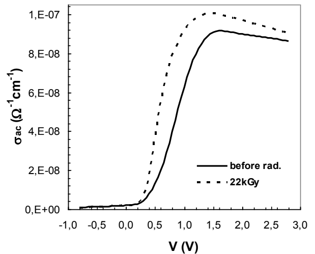
Fig. 3. The variation of the ac electrical conductivity \sigma_{ac} with applied bias for Au/PVA (Co, Zn-doped) n-Si SBD before and after radiation.
