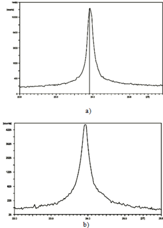
Fig 2 The rocking curves for epitaxial layer ( a) and (b)for substrate
