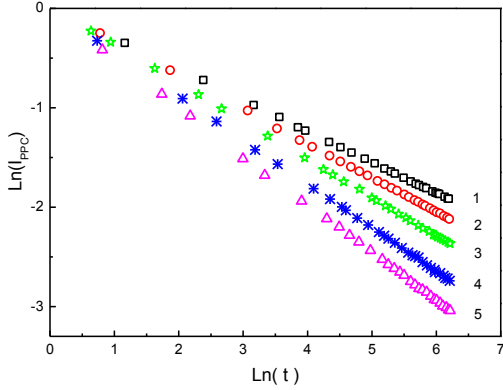
Fig. 3. The PPC decay curves in logarithmic scale for CdTe(Sb) in the temperature range 3 for temperatures T = 205 K (1), 175 K (2), 150 K (3), 125 K (4), 105 K (5)
