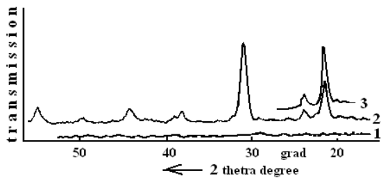
Fig. 3. Diffraction patterns of HPPE source and containing PZT - 5H. 1-HPPE +40% reported PZT-5H; 2-HPPE +40% vol. PZT-5H; 3- HPPE-hardened.
