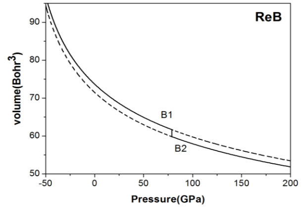
Fig. 2. Pressure versus volume curve of ReB
