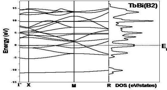
Fig. 6. Calculated band structure of TbBi in phase B2
