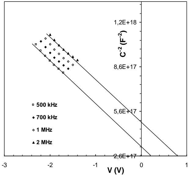
Fig 5. The C^{-2} -V plots of Au/SrTiO 3 /n-Si SBD for various frequencies.
