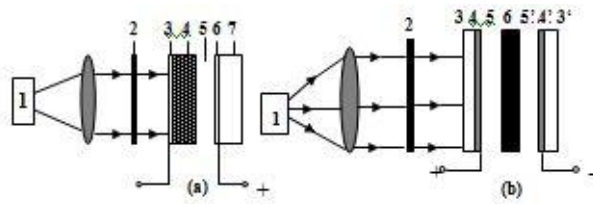
Fig 1 a) Schematic diagram of the gas discharge cell with a semiconductor GaAs cathode.: 1 - light source; 2 - Si filter; 3- semi-transparent Au -contact;4- semiconductor GaAs cathode; 5- gas discharge gap; 6- semi-transparent conductive SnO 2 contact; 7- flat glass disc. b) modified cell with dual short gaps between planar GaAs semiconductor plate and planar transparent electrodes: 1, light source; 2, Si filter; 3 and 3', flat glass disks; 4 and 4', planar transparent SnO 2 electrodes; 5 and 5', symmetrical short gas discharge gaps; 6, planar photosensitive GaAs semiconductor plate.
