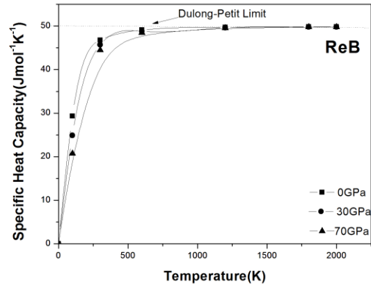
Fig.9. The variation of specific heat capacity with temperature at different pressures for ReB.
