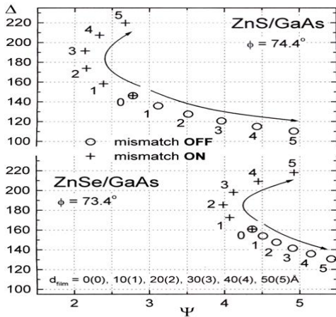
Fig 2. \Delta - \psi graphs with allowance for lattice mismatch effect in ZnS/GaAs and ZnSe/GaAs at various film thicknesses.
