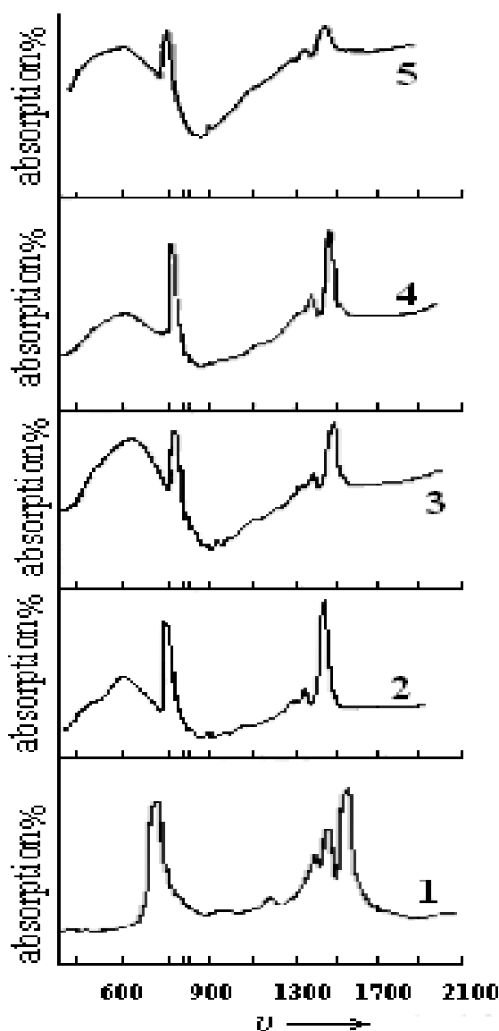
Fig. 7. Spectrum - IR absorption of the composites: 1-HPPE; 2-HPPE+5% vol. PZT - 2; 3-HPPE+10% vol. CaTiO 3 ; 4-HPPE+5% vol. PZT-4; 5-HPPE+10% vol. PZT-4.
