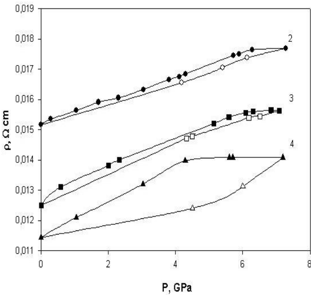
Fig.2 Pressure dependences of resistivity for the : p- Zn_{1-x}Cd_xMn_{0.06}GeAs_2 (№2), p- Zn_{1-x}Cd_xMn_{0.1}GeAs_2 (№3) and p- Zn_{1-x}Cd_xMn_{0.14}GeAs_2 (№4).
