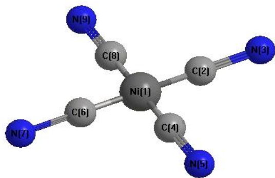
Fig. 3. Unit cell of [\text{Ni}(\text{CN})_4]^{2-} ions.
