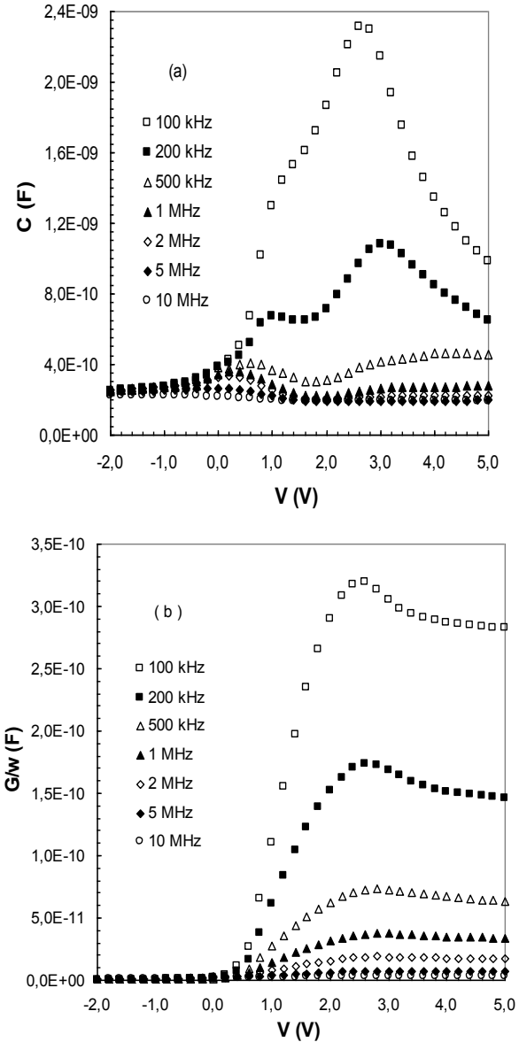
Fig. 1. Variation of the (a) capacitance (C) and (b) conductance (G/w) with frequency at room temperature for MIS structure.
