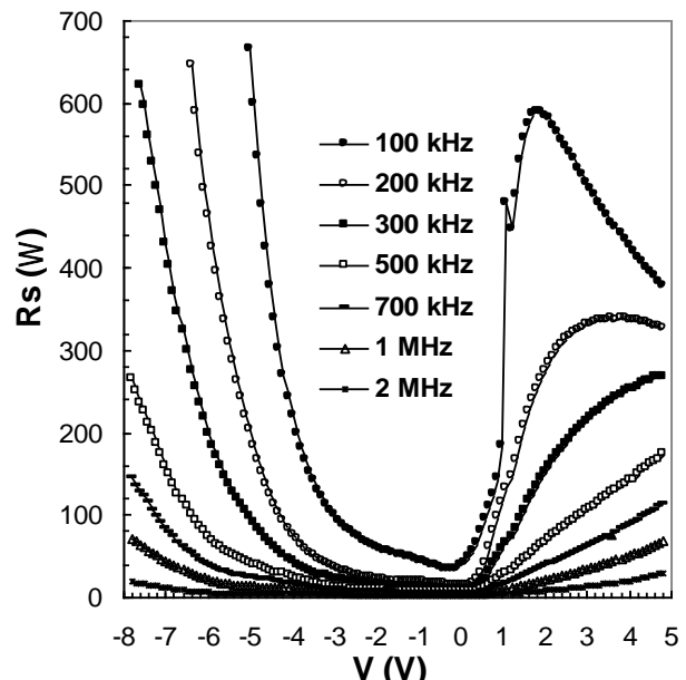
Fig.3. The frequency dependent series resistance in Au/SrTiO 3 /n-Si SBD.
