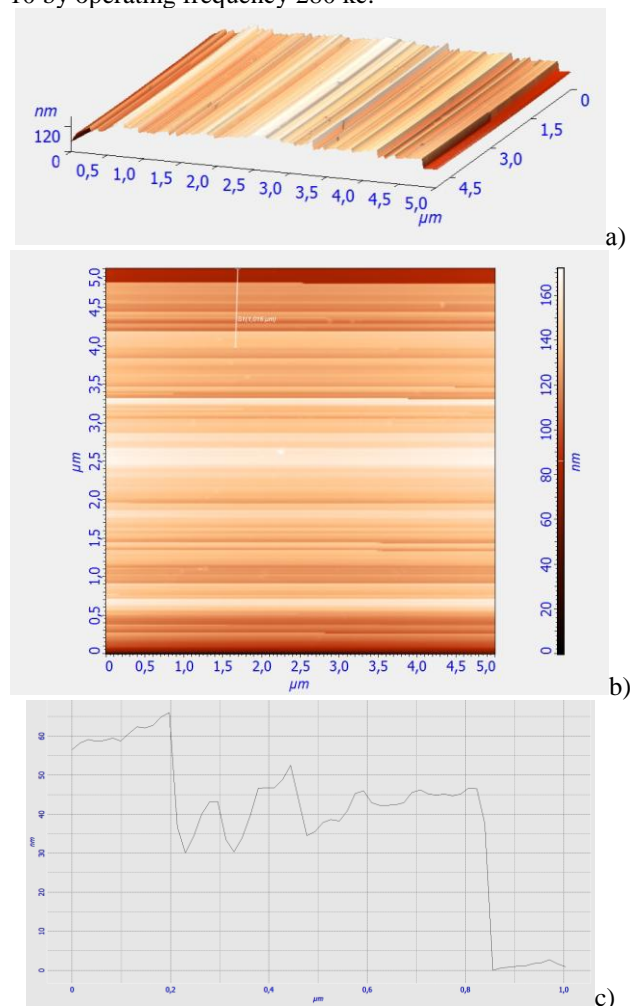
Fig.4 (a, b, c) SPM images of surface (0001) Sb_2Te_3<ZnSb> : a) images of step in 3D- scale; b) step in 2D- scale; c) surface profile along vertical like of pattern on the part b
