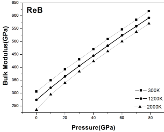
Fig. 6. The relationships of ReB between bulk modulus (B) and pressure P at temperatures of 300 K, 1200 K, 2000 K
