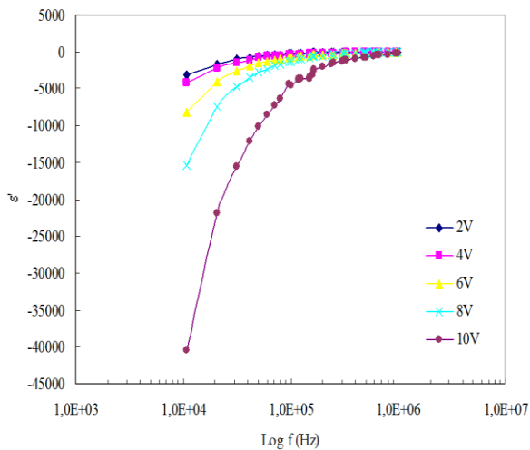
Fig. 3. Variation of dielectric constant ( \epsilon' ) with frequency at different voltages
