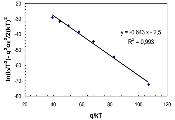
Fig. 6. The plot of \ln(I_0/T^2) - q^2\sigma_0^2/2(kT)^2 versus q/kT for n-GaAs structure.
