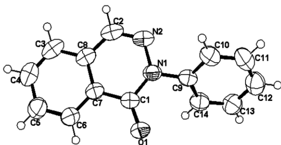
Fig.1. An ORTEP-III drawing of molecule. Thermal ellipsoids are drawn at %50 probability level.
