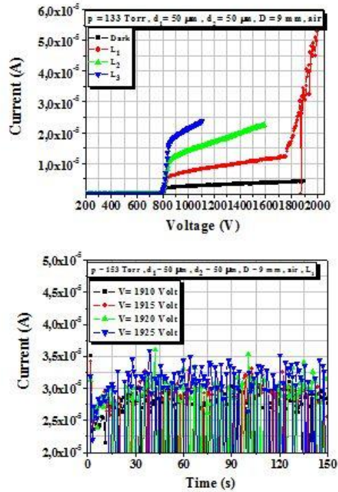
Fig 2. a) CVC of a modified ionization cell in darkness and under weak, moderate and maximum illumination intensity L_1 , L_2 and L_3 , respectively. b) Time dependence of current oscillations in the modified cell under different feeding voltages V_0 for weak illumination intensity L_1 .
