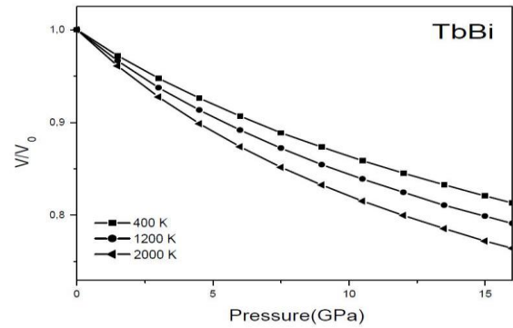
Fig. 4. The normalized volume-pressure diagram of the B1 for TbBi at different temperatures
