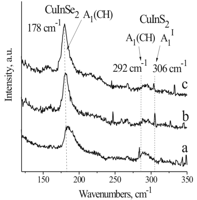
Fig. 6. Raman spectra of CIGSS layers with different S/(S+Se) ratios: a - 0.28; b - 0.19; c - 0.14.
