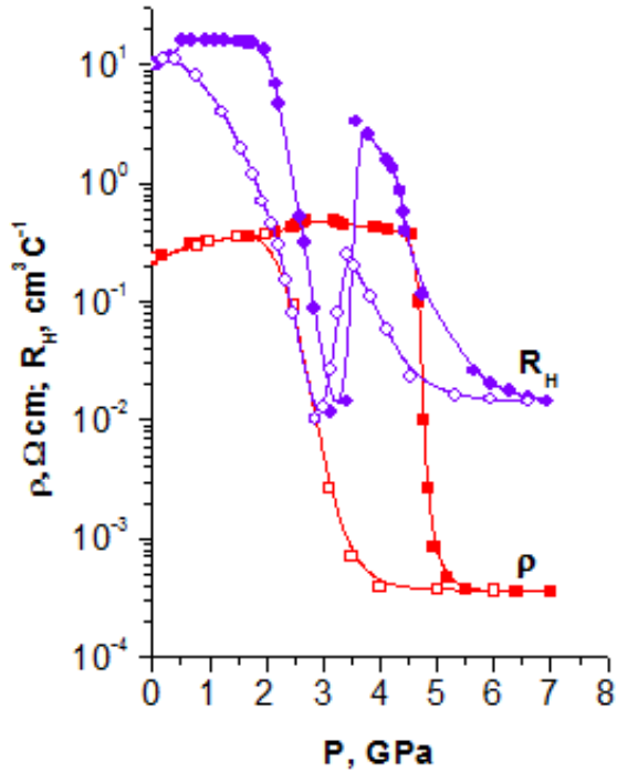
Fig.1. Dependence of specific resistivity – curve 1 and of Hall coefficient - curve 2, at rise of pressure (dark symbols) and fall (light symbols) in magnetic field H=5 kOe
