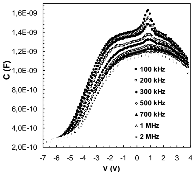
Fig.1. The frequency dependent C-V characteristics of Au/SrTiO 3 /n-Si SBD.
