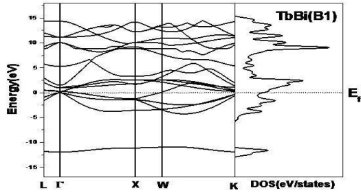
Fig. 5. Calculated band structure of TbBi in phase B1
