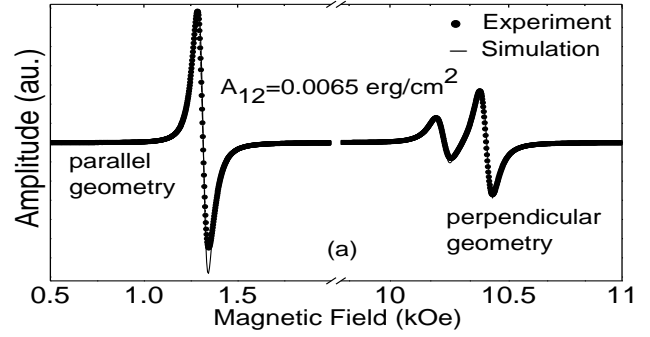
Fig.2. Experimental and simulated FMR spectra of Py(20 Å)/Cr(7 Å)/Py(30 Å) trilayer film for the external field parallel and perpendicular to the sample plane.
