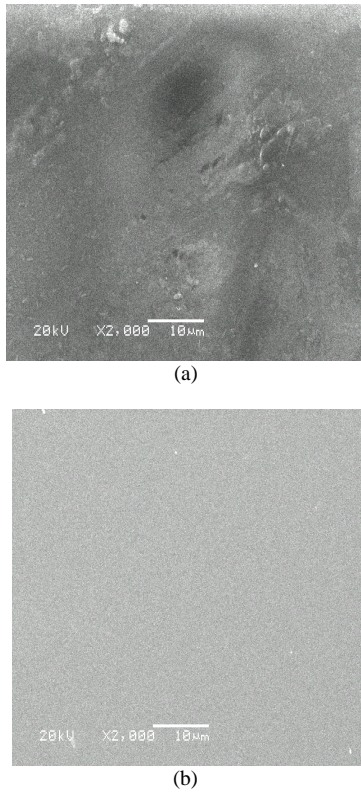
Fig. 6. SEM images of SiO 2 (a) and ZrO 2 (b) coated lenses
