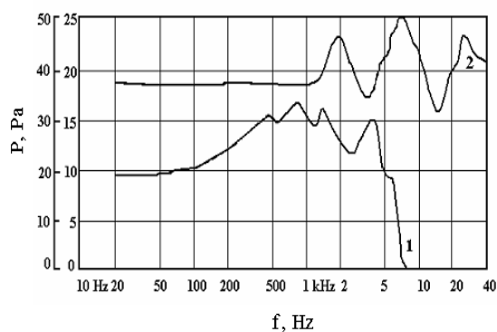
Fig.5. Amplitude-frequency characteristics of output acoustic signal of electroacoustic transducers.
