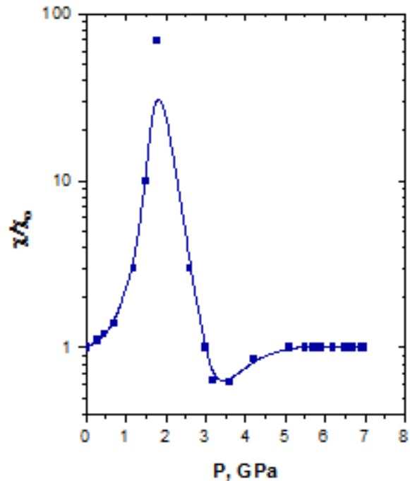
Fig.3. Dependence of relative magnetic susceptibility from pressure.
