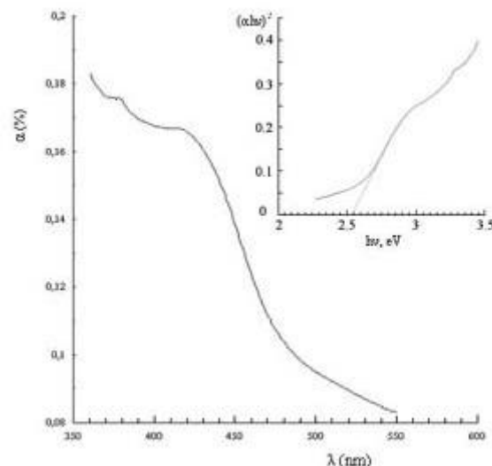
Fig.4. Optical absorption spectrum and energy band gap estimation (inserted figure show the (\alpha h\nu)^2 dependence to h\nu ) for \text{Ga}_2\text{Se}_3 thin films prepared by sol-gel method
