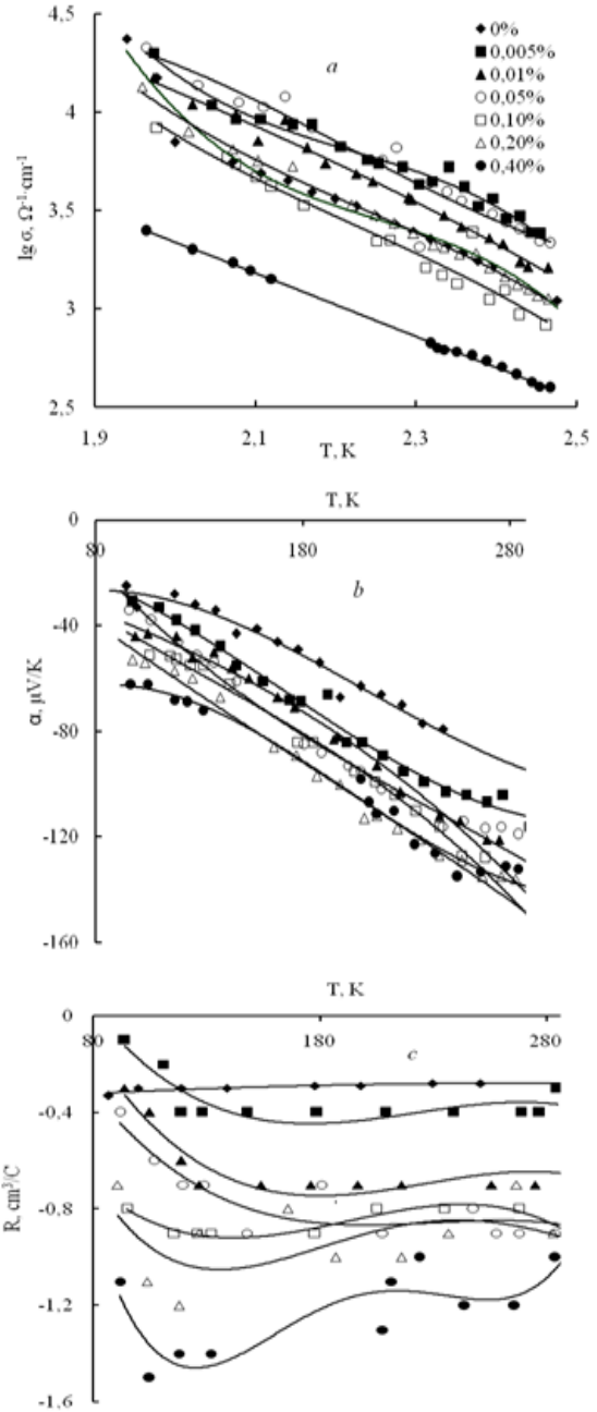
Fig.2. Temperature dependence of electrical conductivity (a), thermo-e.m.f (b) and Hall factor (c) of samples PbTe single crystals doped by Tl, annealed at 873K.
