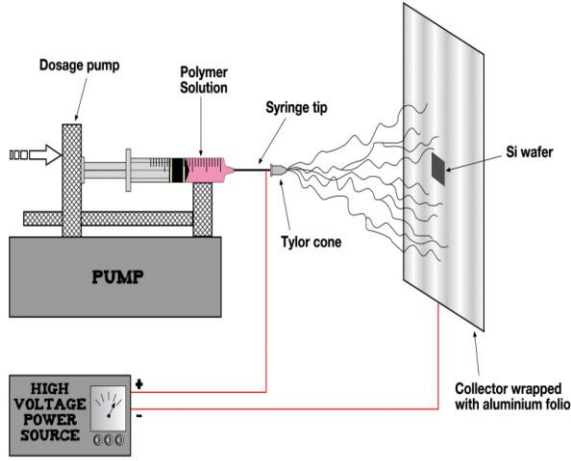
Fig. 1. Schematic representation of the electrospinning process.
