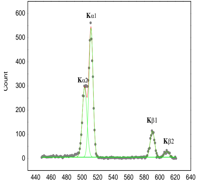
Fig. 2 Typical K X-ray spectra of Ce with Am-241 exciter.
