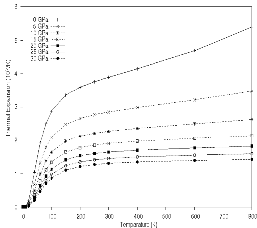
Fig.4. The variation of the thermal expansion coefficient with temperature at various pressures.
