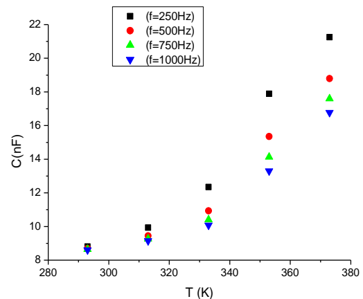
Fig.1. Variation of the capacitance with temperature of TlSbS 2 thin films at different frequencies. Film Thickness: 730 Å
