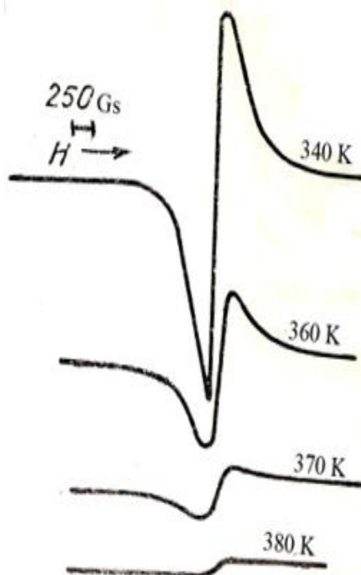
Fig. 1. ESR spectrum of \text{Co}_{0.7}\text{Cu}_{0.3}\text{Cr}_2\text{S}_4 .
