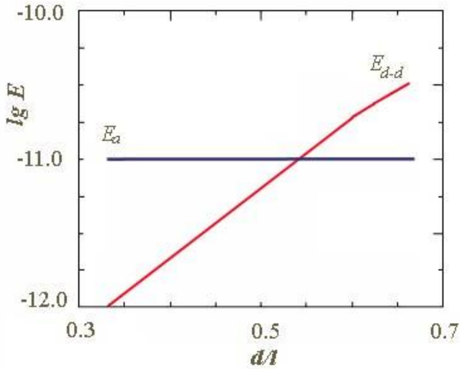
Fig.1 The dependence of energies of dipole-dipole interaction between micropoints E_{d-d} and magnetic anisotropy E_a on ratio d/l .
