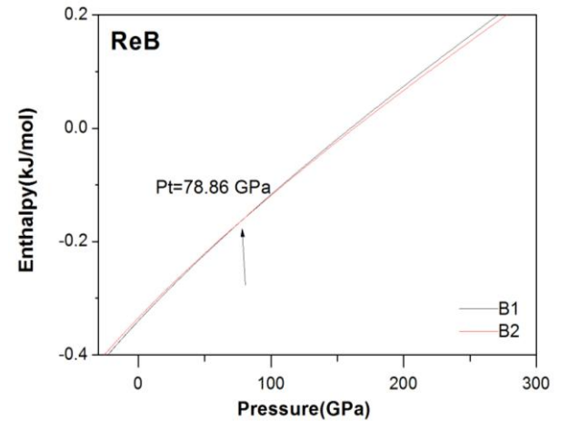
Fig. 3. Estimation of phase transition pressure from B1 to B2 of ReB
