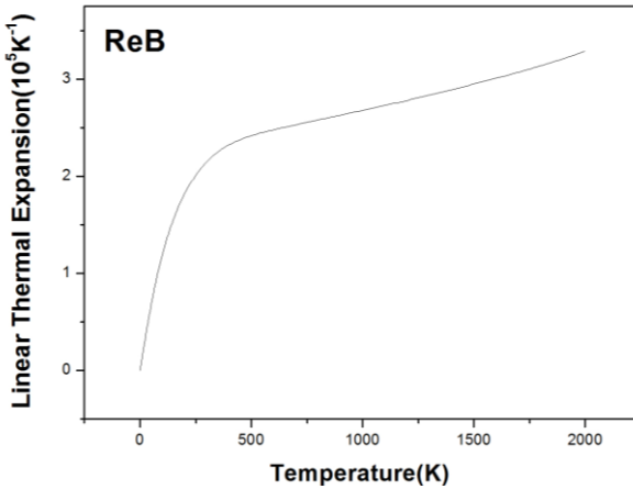
Fig.7. The thermal expansion versus temperature for ReB.
