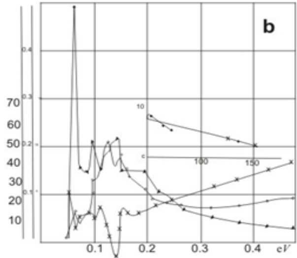
Fig.3. Spectrum of characteristic electronic losses ( -Im\epsilon^{-1} ) and fundamental optics constants ( \epsilon_1; \epsilon_2; n, k ) in range 0.05 ÷ 0.50eV
