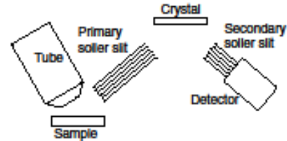
Fig. 1. A scheme of spectrometer.
