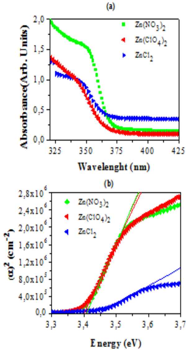
Fig. 3. a) Absorption spectra and b) \alpha^2 vs. energy plot of ZnO thin films.
