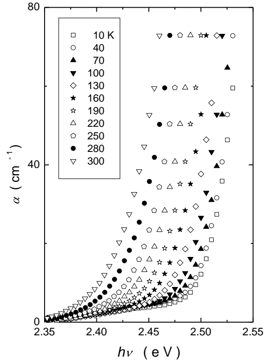
Fig.2. Absorption coefficient versus photon energy for \text{TlIn}_{0.5}\text{Ga}_{0.5}\text{S}_2 crystal in the temperature range of 10–300 K.
