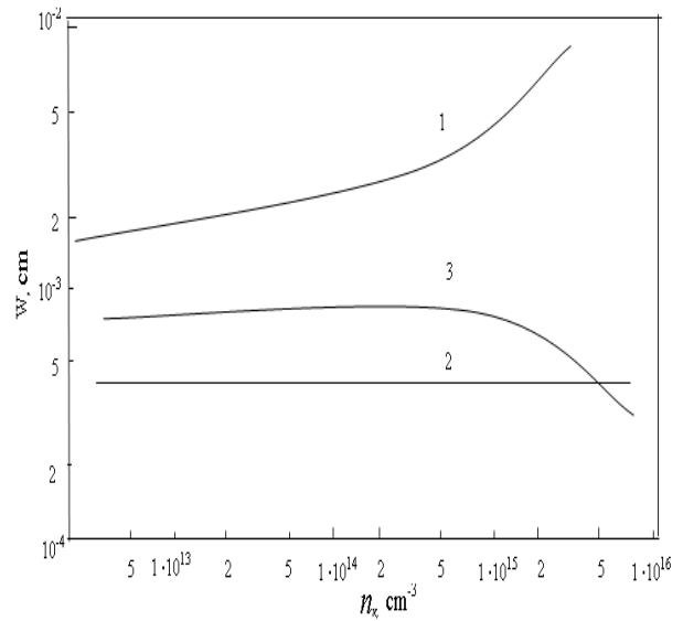
Fig.1. Calculated curves of dependences of width of the volume charge layer of collector junction on concentration of nonequilibrium carriers: 1- a_1=3.3 \times 10^{18} \text{cm}^{-4} , a_2=6.7 \times 10^{17} \text{cm}^{-4} , U_{rev}=50 \text{V} ; 2- a_1=a_2=1.3 \times 10^{20} \text{cm}^{-4} , a_2=6.7 \times 10^{17} \text{cm}^{-4} , U_{rev}=10 \text{V} ; 3- a_1=3.3 \times 10^{18} \text{cm}^{-4} , a_2=4.7 \times 10^{20} \text{cm}^{-4} , U_{rev}=50 \text{V}
