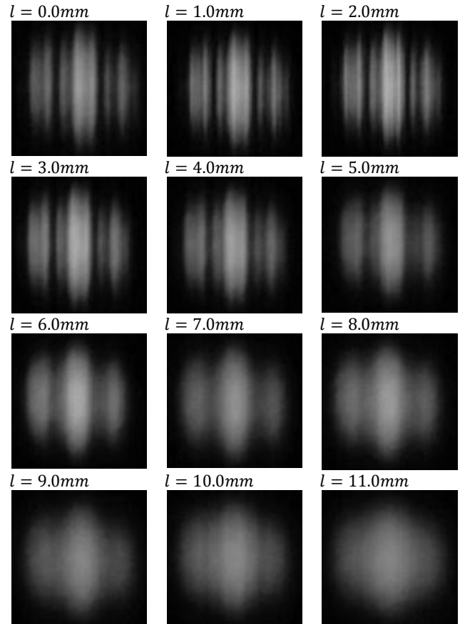
Fig.6. Interferogram generated by the mask, for increasing distances between focal point of the lens L_1 and RGG, starting from l = 0.0 mm to l = 11.0 mm .
