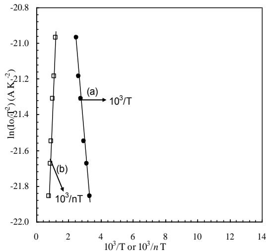
Fig.4. Richardson plots of the \ln(I_o/T^2) or 1/T or 1/nT and \ln(I_o/T^2) versus 1/nT for Au/n-GaAs Schottky diode.
