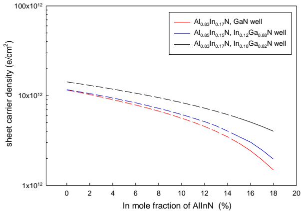
Fig.6. In different In mole fraction change In different wells of sheet carrier density for the AlInN barrier layer . Dashed lines shows the strain relaxation.
