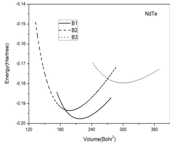
Fig.2. Total energy versus volume curves of NdTe in NaCl(B1), CsCl(B2) and ZB(B3) structure.
