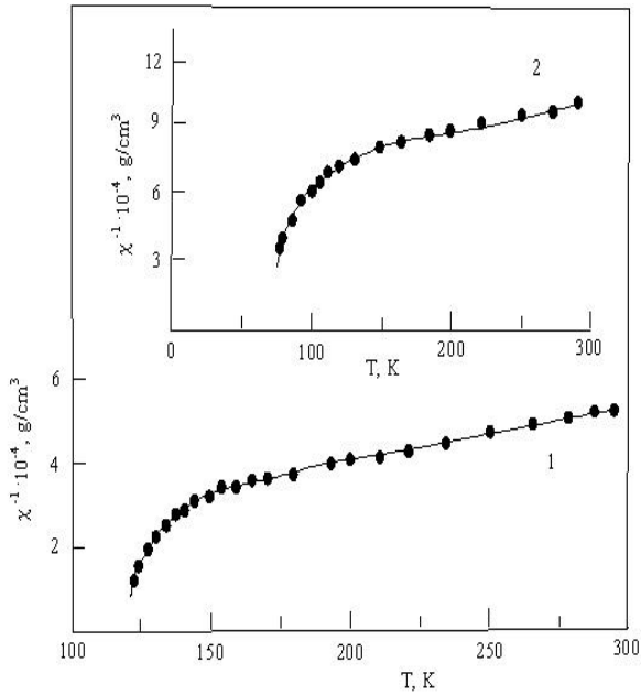
Fig.5. The temperature dependence of the inverse paramagnetic susceptibility of \text{TlCoS}_2 (1) and \text{TlCoSe}_2 (2). (Figure corresponds to publication [15].)
