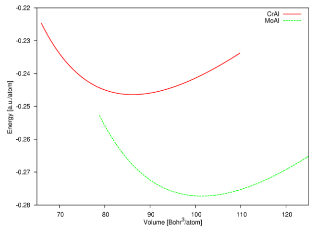
Fig. 1. The Energy-Volume curves of CrAl and MoAl in B32 structure.
