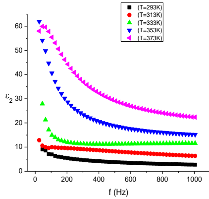
Fig.6. Frequency dependence of the dielectric loss factor \epsilon_2 , of TlSb 2 thin films at different temperatures. Film Thickness: 4090 Å
