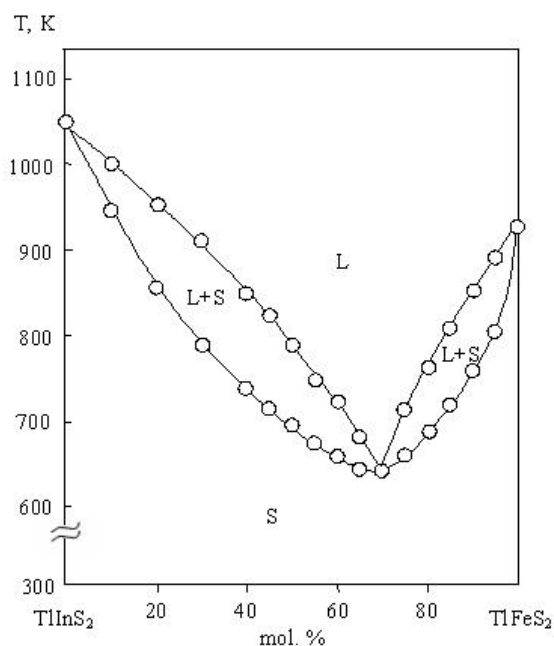
Fig.8. \text{TlInS}_2\text{-TlFeS}_2 system state diagram.
