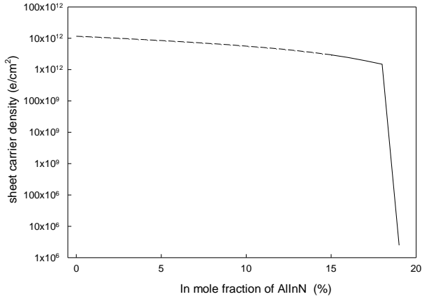
Fig.2. Determined In mole fractions for AlInN barrier with 25nm thickness in GaN quantum well. Dashed lines represent the strain relaxed situation.
