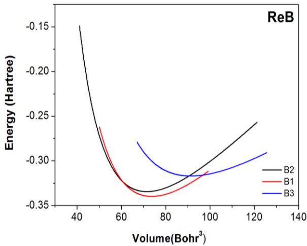
Fig. 1. Total energy versus volume curve of ReB in B1(NaCl), B2(CsCl), B3(ZB), phases.
