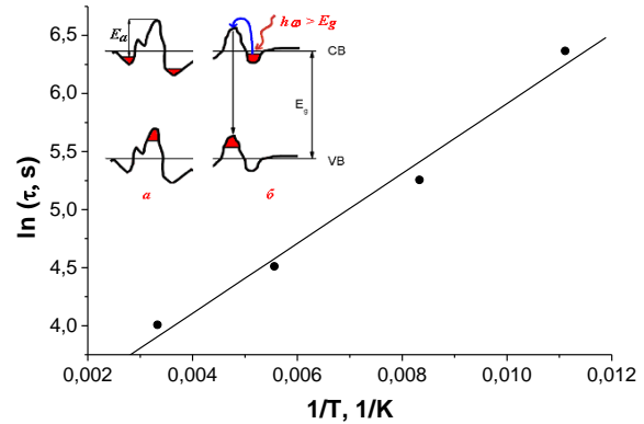
Fig. 2. Temperature dependences of PPC relaxation time constant \tau in Arrhenius scale for the undoped CdTe crystal. In Insert, a schematic presentation of the randomly modulated edges of energy bands with the mean values E_a of RLPF before (a) and after (b) lightening.
