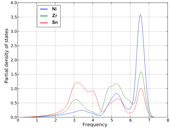
Fig. 4. Partial phonon density of states for NiZrSn compound.
