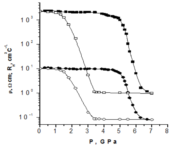
Fig.3. Baric dependence of specific resistivity (circles) and Hall coefficient (squares) at rise (dark symbols) and at fall (light symbols) of pressure for p-Cd_{0.94}Mn_{0.06}GeAs_2 sample.
