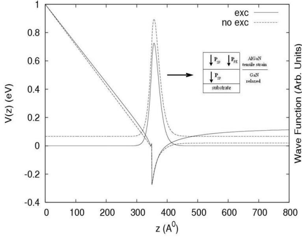
Fig.1. The conduction band profile obtained from Poisson/Schrödinger equations and the wavefunctions corresponding to ground state at 300 K. Solid lines are for the case when exchange potential is considered and dashed lines are for the case when it is neglected. The inset shows the geometry of the \text{Al}_{0.2}\text{Ga}_{0.8}\text{N}/\text{GaN} heterostructure considered in this study. The barrier length is 350 \text{ \AA} , the GaN width is 4500 \text{ \AA} . The chemical potential is assumed to be 1 eV below the conduction band of AlGaIn.
