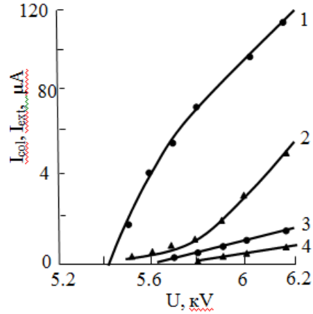
Fig. 2. Dependence of current components in collector and extractor circuits from extracting voltage (In): 1 – I col , 2 – I ext , 3 – I ext ~ , 4 – I col ~
