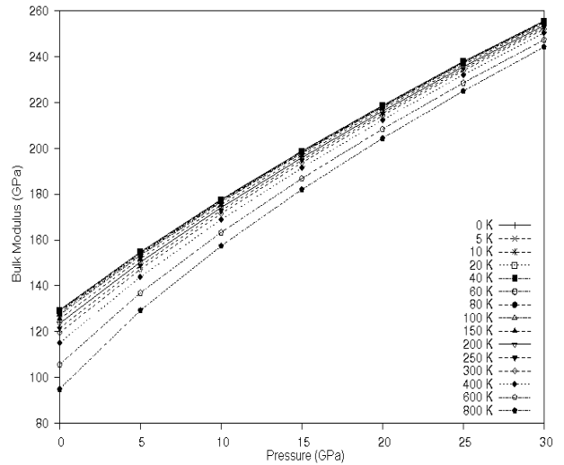
Fig.2. The variation of bulk modulus with pressure for various temperatures.
