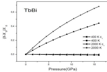
Fig.11. Variations of thermodynamic parameters X (X: Debye temperature or specific heat) with pressure P. They are normalized as (X-X_0)/X_0 , where X and X_0 are the Debye
