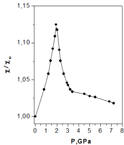
Fig.6. Baric dependence of relative magnetic susceptibility \chi/\chi_0 from pressure for p-Cd 0.94 Mn 0.06 GeAs 2 . The cut-in shows temperature dependence of magnetization for the studied sample.
