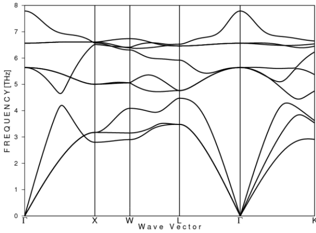
Fig. 2. Phonon dispersion curves with LO-TO along first Brillouin zone for NiZrSn compound.
