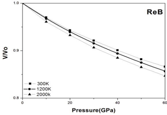
Fig. 4. The normalized volume-pressure diagram of the B1 for ReB at different temperatures
