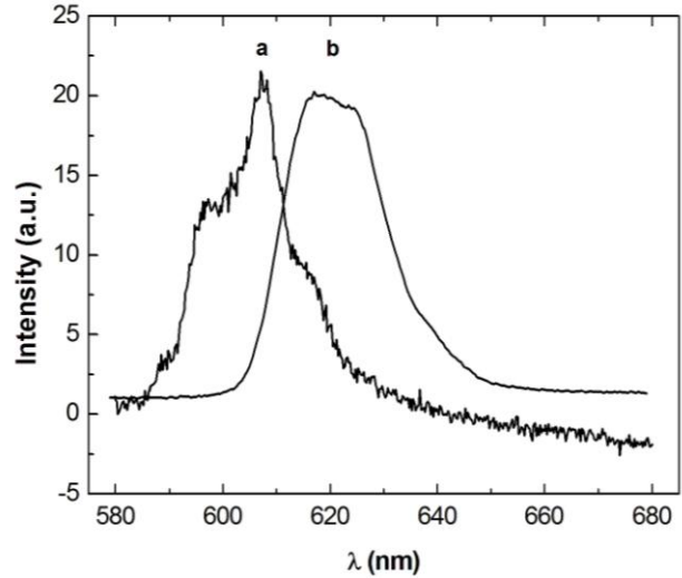
Fig.5. The PL spectra of a) GaSe face of MnS-GaSe junction and b) MnS thin film deposited face. The PL measurements were conducted at 50 K.
