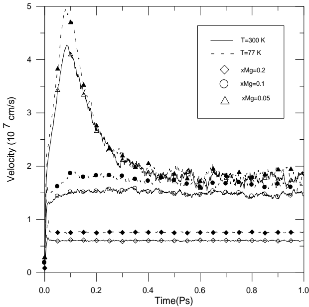
Fig.3 The electron drift velocity at different alloy concentrations in Zn_{1-x}Mg_xO at an applied field of F_x= 800 kV/cm for two different temperatures. The filled symbols with dashed lines are for T=77 K and empty symbols with solid lines refer to T=300 K.
