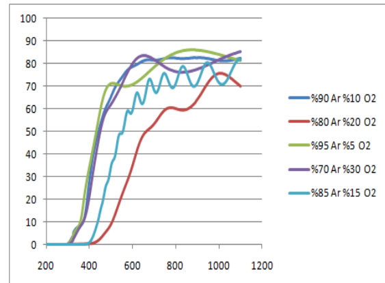
Fig. 2. Transmittance spectra of deposited ZnO thin films
