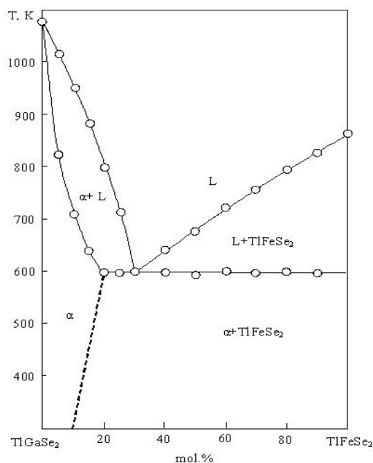
Fig.9. \text{TlGaSe}_2\text{-TlFeSe}_2 system state diagram.
