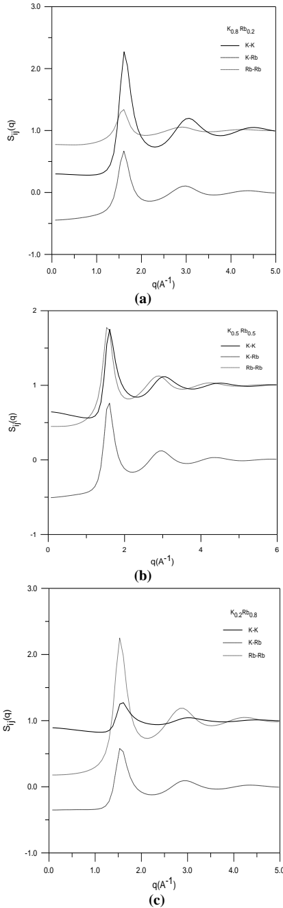
Fig. 2 Ashcroft-Langreth partial structure factors for the three alloys under consideration. Solid, dot-dashed and dotted
