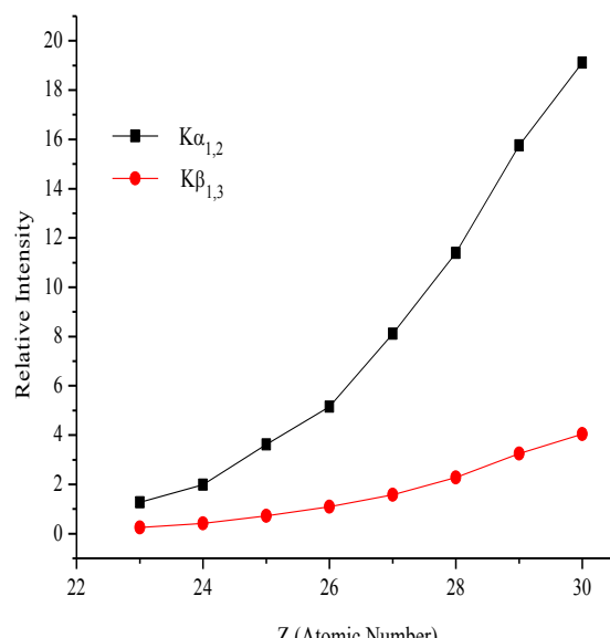
Fig. 5 Relative intensity of the K_{\alpha 1,2} and K_{\beta 1,3} lines plotted as a function of the atomic number.
