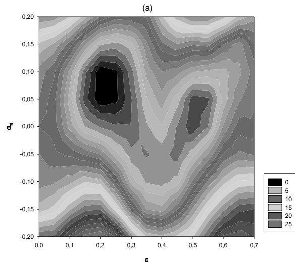
Fig.4 The same as in fig 1 but for ^{233}\text{Pa} .
