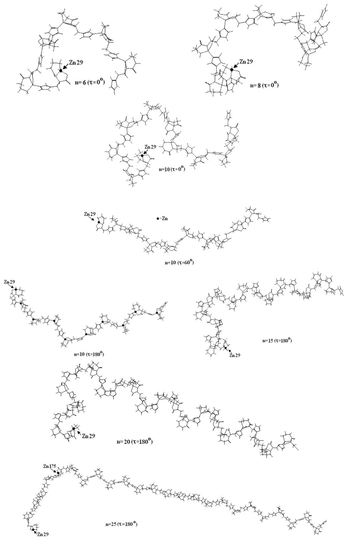
Fig.1. Model of the carnosine polymeric complex with Zn ( n=6, 8, 10, 15, 20 and 25 )
