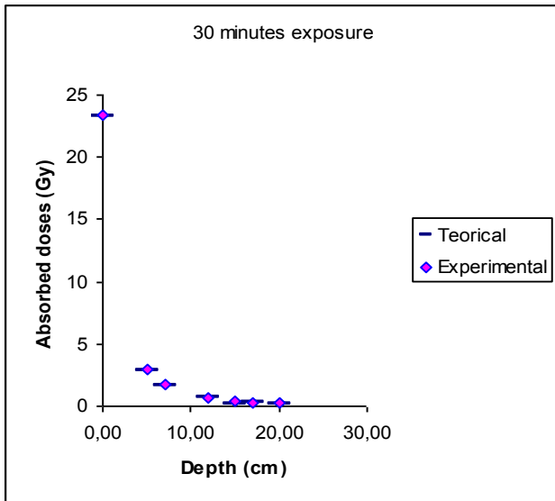
Fig. 3. Absorbed organ doses versus depth ranging from 0 to 20 for estimated exposure time (30 minutes)
