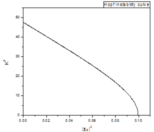
Fig.3. Instability domain for the Hopf instability, J = 1.288 , \theta = 2 , \alpha = 4 .
