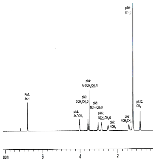
Fig.4. 400 MHz ^1\text{H-NMR} spectrum of ligand2 ( \text{CDCl}_3 ). Peak1:Ar-H; peak2:Ar-OCH 2 ; peak3:OCH 2 CH 2 O; peak4:Ar-OCH 2 CH 2 N; peak5:NCH 2 CH 2 O; peak6:NCH 2 CH 2 O; peak7:NCH 2 ; peak8:NCH 2 CH 2 ; peak9:(CH 2 ); peak10:CH 3
