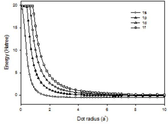
Fig. 1 Energy of the ground state 1s , the first 1p , the second 1d and the third 1f excited states versus the dot radius for a one-electron GaAs/Al x Ga 1-x As QD for x=0.3 .
