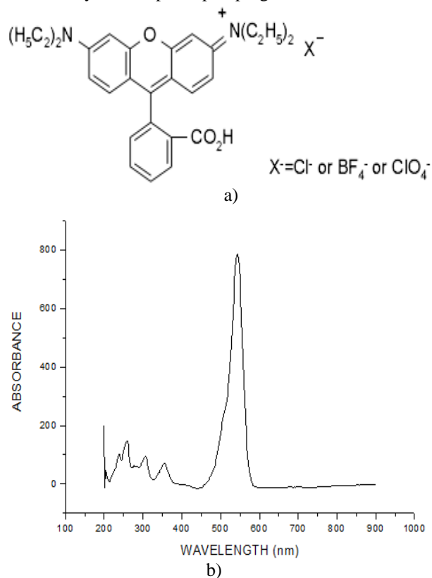
Fig. 1 a) chemical structure and b) absorption spectrum of rhodamine 610 in ethanol at room temperature.
