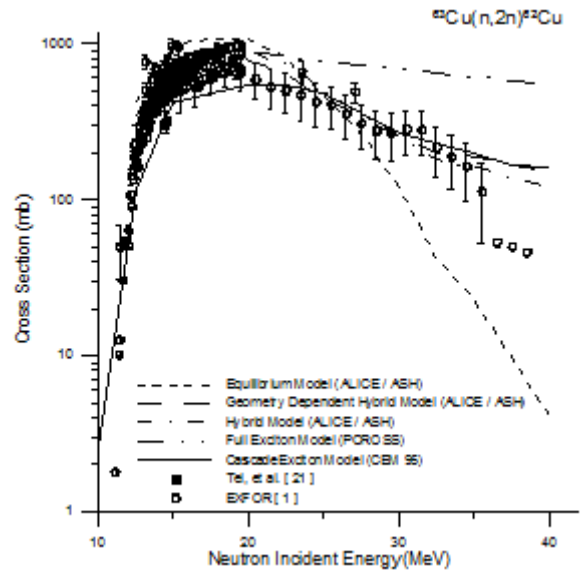
Fig.3. The comparison of calculated excitation function of ^{63}\text{Cu}(n,2n)^{62}\text{Cu} reaction with the values reported in [1].
