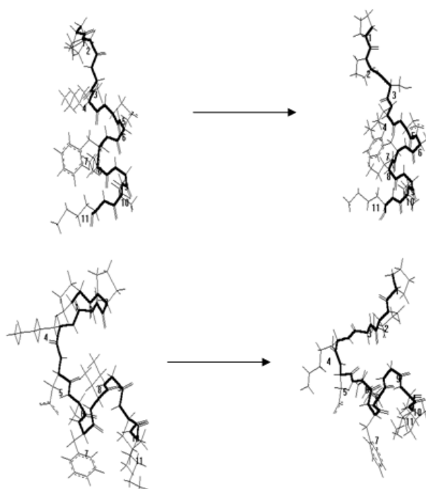
Fig.2. Conformational reorganization of the eledoisin molecule at the molecular dynamic simulation in vacuum (at the top) and in water (below).
