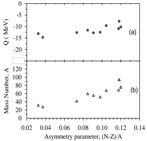
Fig.1.a. (n, {}^3\text{He}) reaction Q-values by depending up on asymmetry parameter; b. Asymmetry parameter values for the target nuclei mass number-A used in this work.
