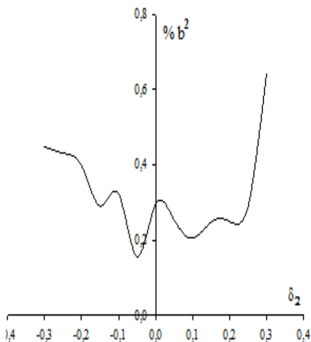
Fig. 1. Dependence on deformation parameter of isospin admixture for ^{122}\text{Xe} isotope.
