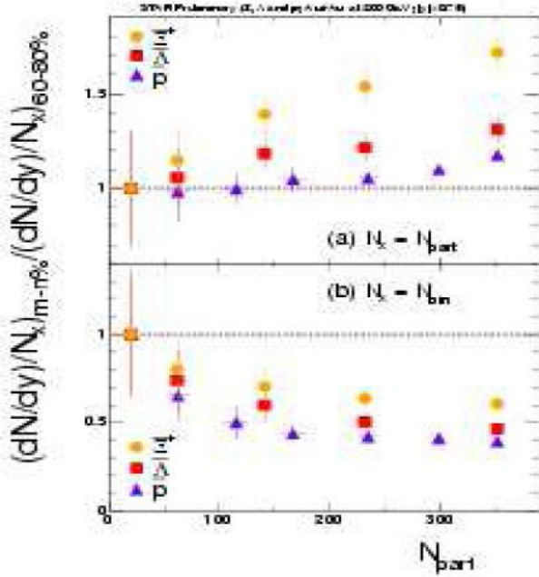
Fig.7. The nuclear modification factors of the strange particles as a function of centrality.
