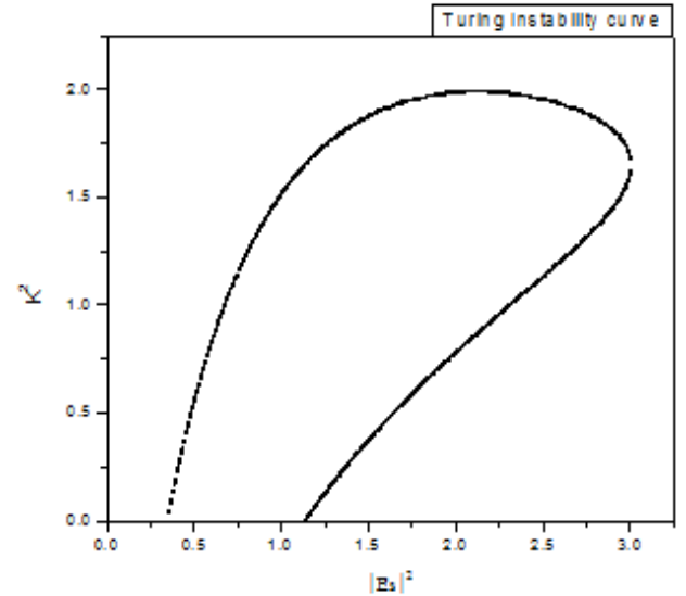
Fig.2. Instability domain for the Turing instability, J = 1.288 , \theta = -2 , \alpha = 4 .
