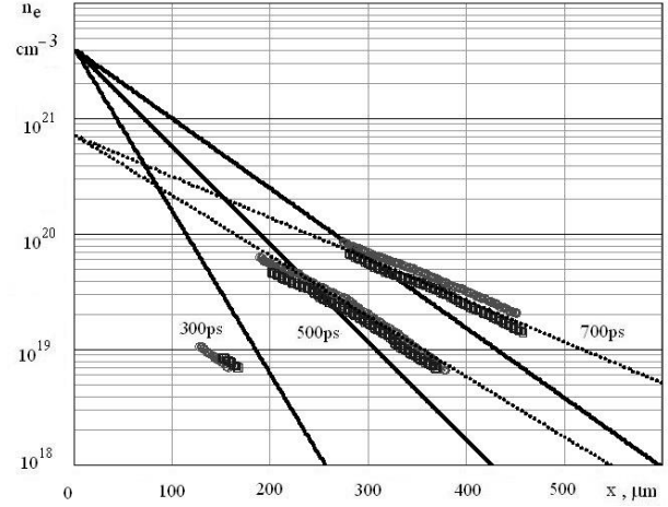
Fig. 4: Comparison of experimental profiles of electron density with the predictions of the analytic 1D model: experimental data for shot # 7 (rings) and shot # 10 (squares), prediction of 1D self-similar model (solid straight lines), and the linear extrapolation of experimental results (middle between shock # 7 shot # 10, dotted straight lines).
