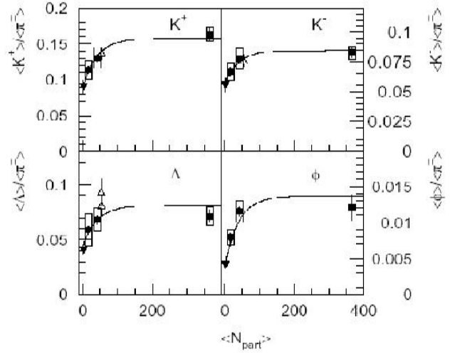
Fig.5 The experimental ratios of \langle K^+ \rangle , \langle K^- \rangle , \phi , and \Lambda to \langle \pi^\pm \rangle plotted as a function of system size ( \nabla p+p , \square C+C and \bullet Si+Si , \circ S+S , \blacksquare Pb+Pb ).
