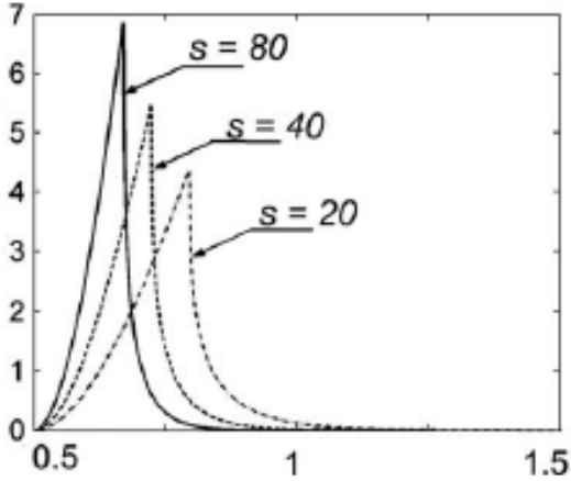
Fig. 3. Splitting gap behavior for three values of the ratio s of characteristic Josephson energy E_J to Coulomb energy E_C at the presence of the second harmonic
