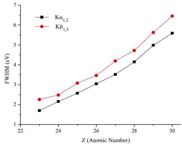
Fig. 3 FWHM of the K\alpha_{1,2} and K\beta_{1,3} lines plotted as a function of the atomic number.
