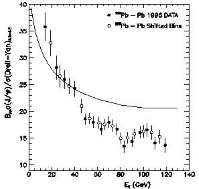
Fig.6. The ratio of the J/\psi to Drell-Yan cross-sections as a function of centrality.
