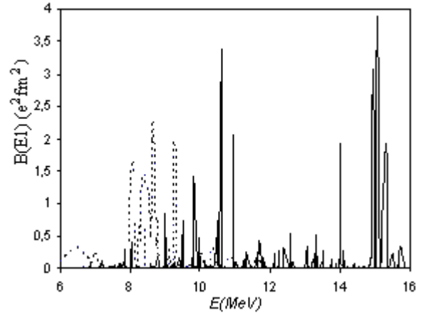
Fig. 3. K=0 and K=1 electric dipole distributions in ^{236}\text{U} nuclei
