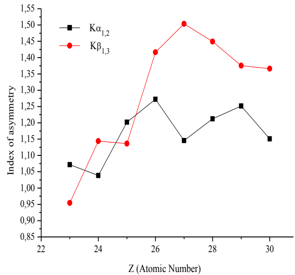
Fig. 4 Asymmetry index of the K\alpha_{1,2} and K\beta_{1,3} lines plotted as a function of the atomic number.
