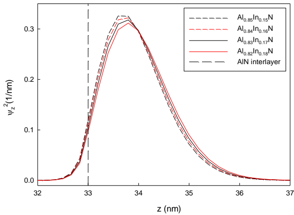
Fig.3. Probability densities of the 2DEG carriers of well for different In-mole fractions in 25nm AlInN barrier thickness.
