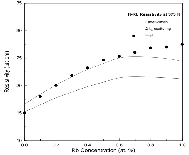
Fig. 3 Calculated electrical resistivities of K-Rb alloys together with available experimental data [18] at 373 K.
