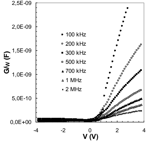
Fig 2. The frequency dependent G/ω-V characteristics of Au/SrTiO 3 /n-Si SBD.
