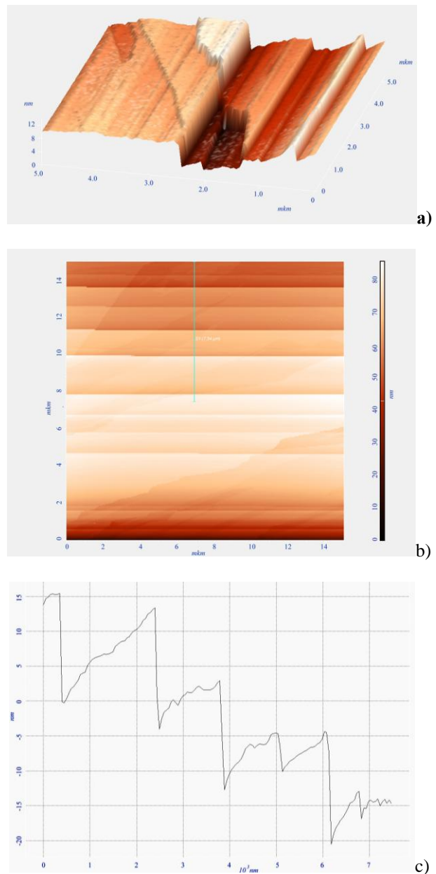
Fig.3 (a, b, c) SPM images of bismuth telluride doped by Ni: a) image of steps in 3D-scale; b) image of steps in 2D- scale; c) step profile along vertical like in the middle of pattern on the part.
