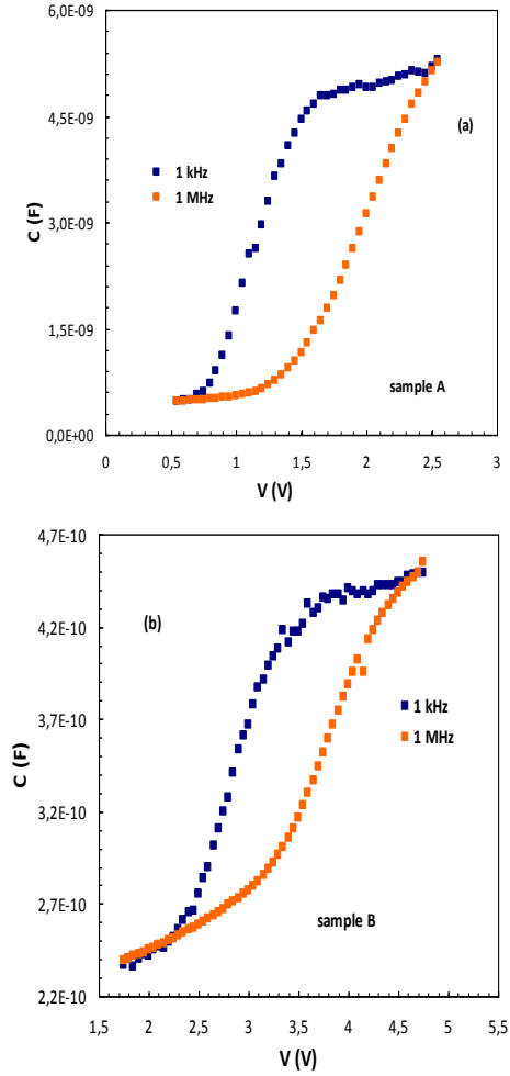
Fig. 1. The measured high-low frequency capacitance (C HF - C LF ) plots of the Al/SiO 2 /p-Si Schottky diodes for samples A and B at room temperature.
