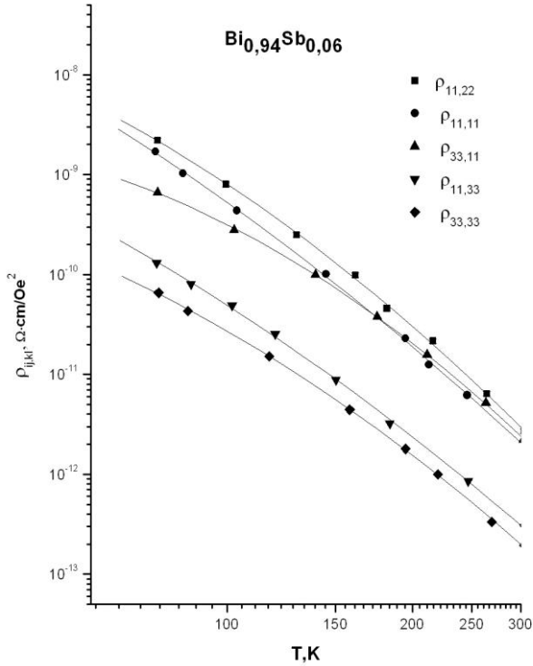
Fig.2. Temperature dependence of the magnetoresistance coefficients.
