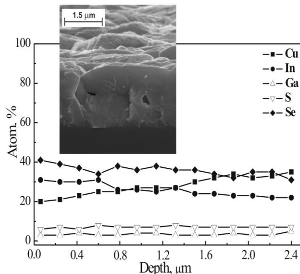
Fig. 2. SEM cross-section image and AES profiles of CIGSS layer grown under 520 °C
