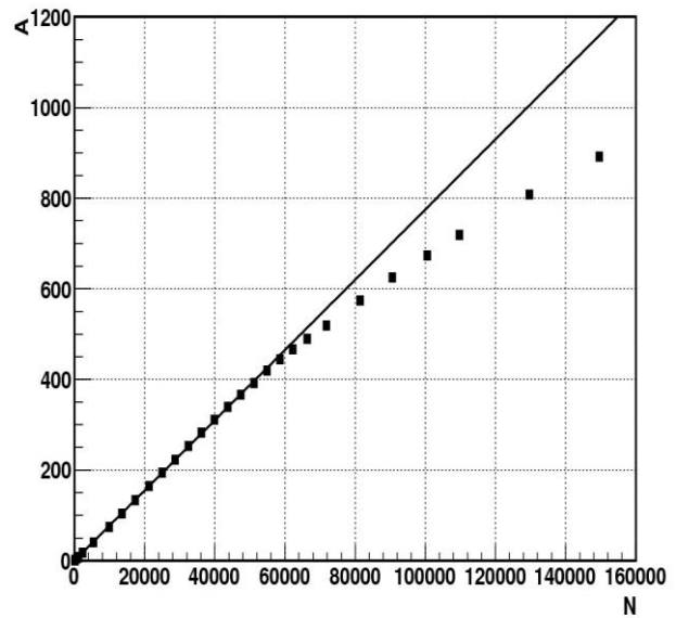
Fig.3. Dependence of MC APD photoresponse amplitude A (in relative units) on a number of incident photons N.
