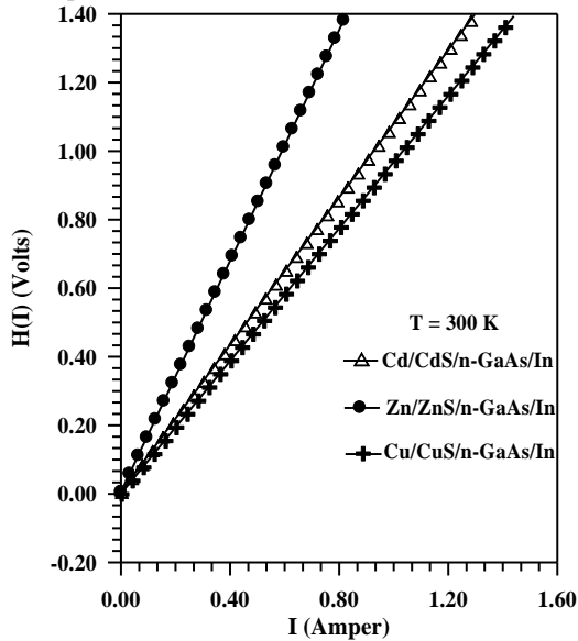
Fig 3. Experimental H(I)-I curves of sandwich structures
