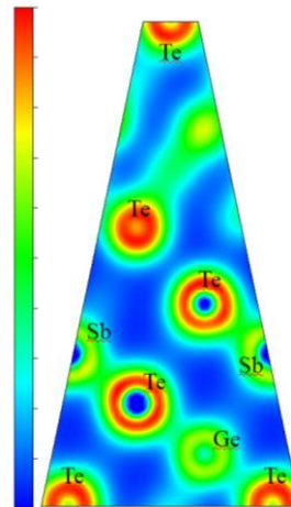
Fig. 4. Electronic charge density contour plot of \text{Ge}_2\text{Sb}_2\text{Te}_5 compound for model II.
