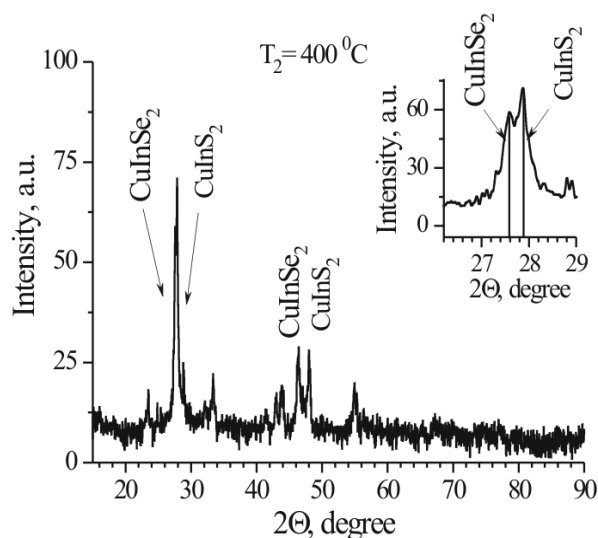
Fig. 3. XRD pattern of CIGSS film grown under 400 °C
