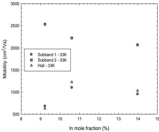
Fig. 5 In mole fraction dependent mobility for hall, first and second subband
