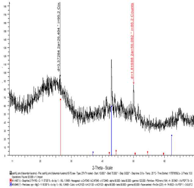
Fig. 1. XRD of the sample
