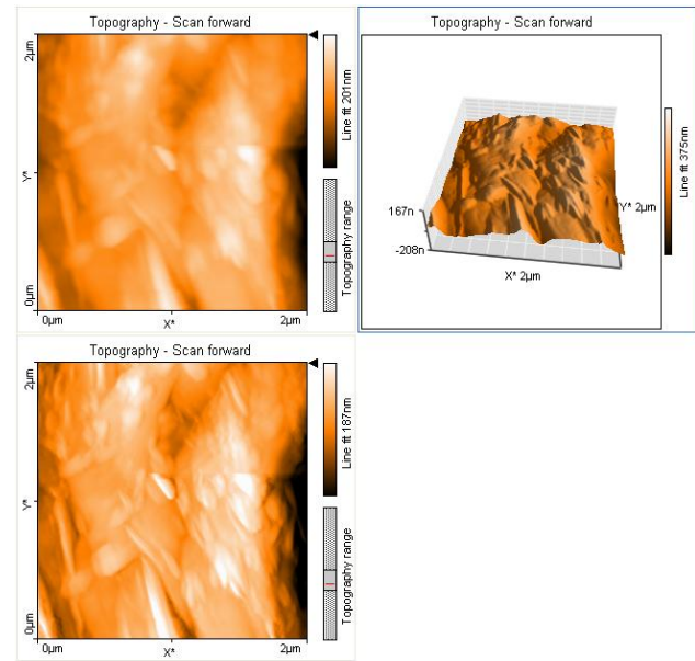
Fig.2. The AFM image of MnS films grown on glass substrate.
