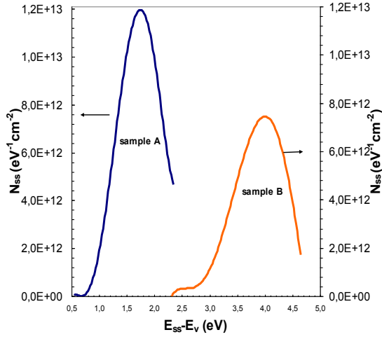
Fig. 3. The energy density distribution profile of surface states in the Al/SiO 2 /p-Si Schottky diodes for samples A and B at room temperature.
