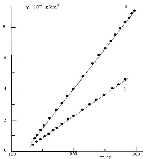
Fig.3. The temperature dependence of the inverse paramagnetic susceptibility of \text{TlCrS}_2 (1) and \text{TlCrSe}_2 (2). (Figure corresponds to publication [9].)
