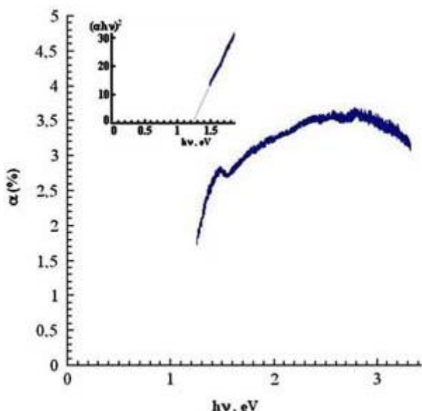
Fig.3. Optical absorption spectrum and energy band gap estimation (inserted figure show the (\alpha h\nu)^2 dependence to h\nu ) for \text{In}_2\text{Se}_3 thin films prepared by sol-gel method
