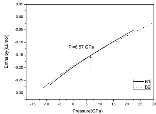
Fig.4. Enthalpy versus pressure curves of NdTe
