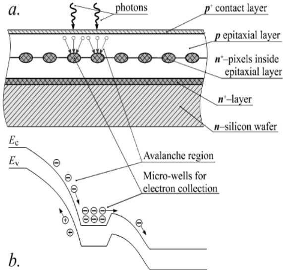
Fig.1. MC APD cross-section (a) and energy zone diagram (b) then bias voltage is applied.
