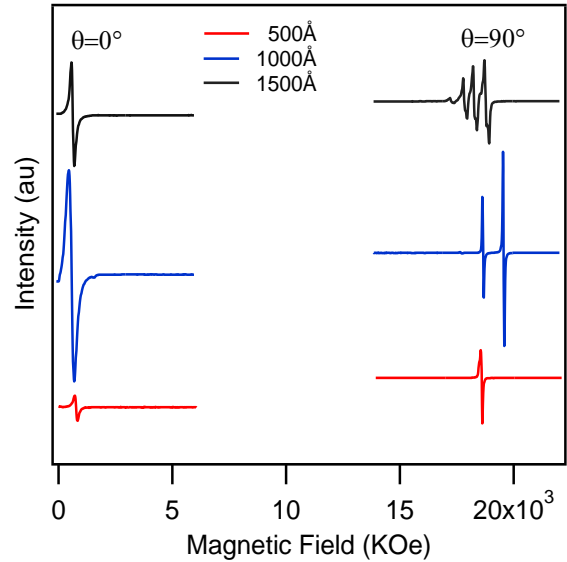
Fig. 3. Room temperature experimental SWR spectra taken X-band from three different cobalt thicknesses for both parallel \theta = 90^\circ and perpendicular \theta = 0^\circ geometries.
