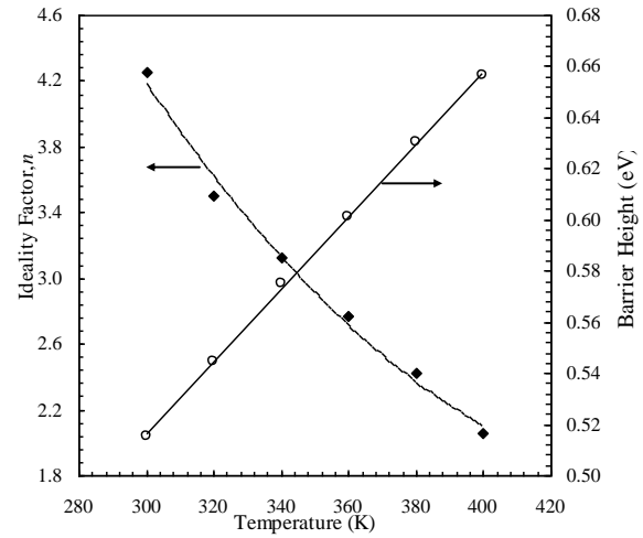
Fig. 2. The variation of the ideality factor and the barrier height.
