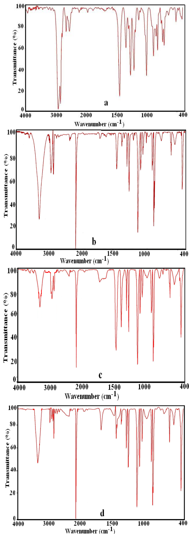
Fig. 1. The FT-IR spectra of the liquid CHT (a), the \text{Co}(\text{CHT})_2\text{Ni}(\text{CN})_4 \cdot \text{D} (b), the \text{Ni}(\text{CHT})_2\text{Ni}(\text{CN})_4 \cdot \text{D} (c) and the \text{Cd}(\text{CHT})_2\text{Ni}(\text{CN})_4 \cdot \text{D} (d) clathrates.
