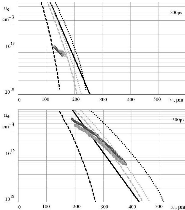
Fig.5. The dependences of electron density (rings for shot #7 and squares for shot # 10), calculation from the 1D self-similar model (solid straight lines), results of 1D MULTI simulation: with LTE (grey), without LTE (black), with account of radiation transport (dashed), without account of radiation transport (dotted).
