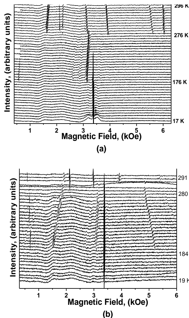
Fig.2. Temperature dependence of the EPR spectra of BaTiO 3 substrate possessing Fe impurities measured at “in-plane” (a) and “out-of-plane” (b) geometries.
