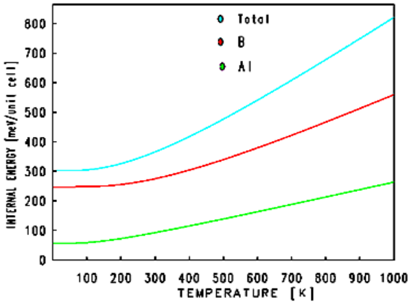
Fig. 2. Temperature dependence of internal energy for for \text{AlB}_2
