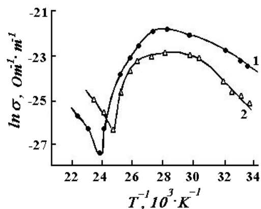
Fig. 1. Dependence \ln \sigma from 1/T . 1-HDPE+BN; 2-HDPE+AlN.
