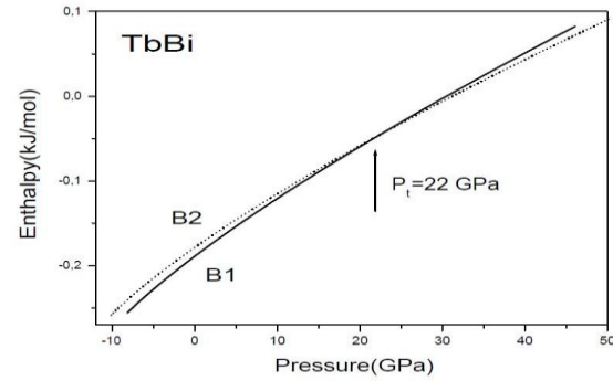
Fig. 3. Estimation of phase transition pressure from B1 to B2 of TbBi
