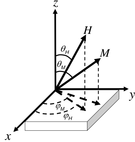
Fig.1. Relative orientations of the external dc magnetic field and magnetization vectors with respect to the sample plane
