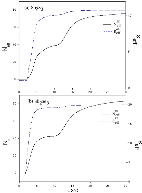
Fig. 3. Energy spectra of N_{eff} and \epsilon_{eff} along the z- axes
