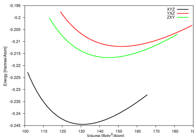
Fig. 1. Calculated cohesive Energy curves for NiZrSn. (X=Ni, Y=Zr, Z=Sn)
