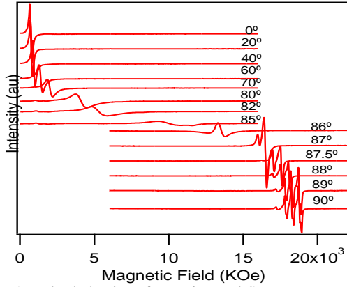
Fig. 5. Angular behavior of experimental SWR spectra taken at room temperature from 1500 Å thickness Co thin film. Direction for magnetic field is same as in the figure 4.
