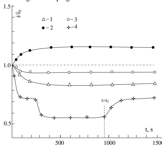
Fig. 1. Kinetics of the dark current in p-GaSe<Ho> crystals at different values of an external voltage. U, V: 1 - 20; 2 - 30; 3 - 40; 4 - 60. N = 10^{-4} at. %, T = 77 K.
