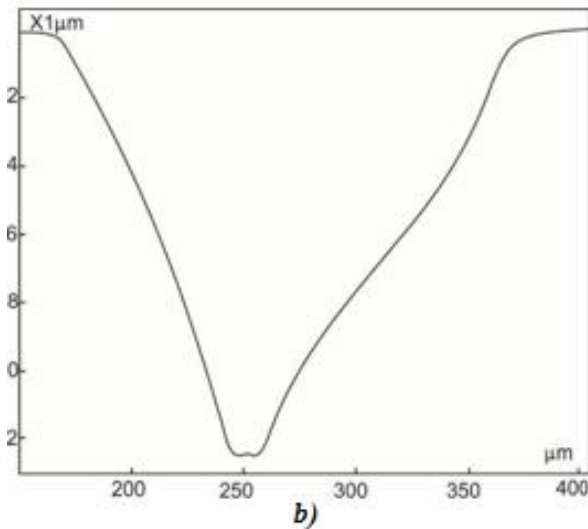
Fig. 4. The micro funnel like defects on the surface of the epilayer ; a-micro-funnel ; b-profile of the defect
