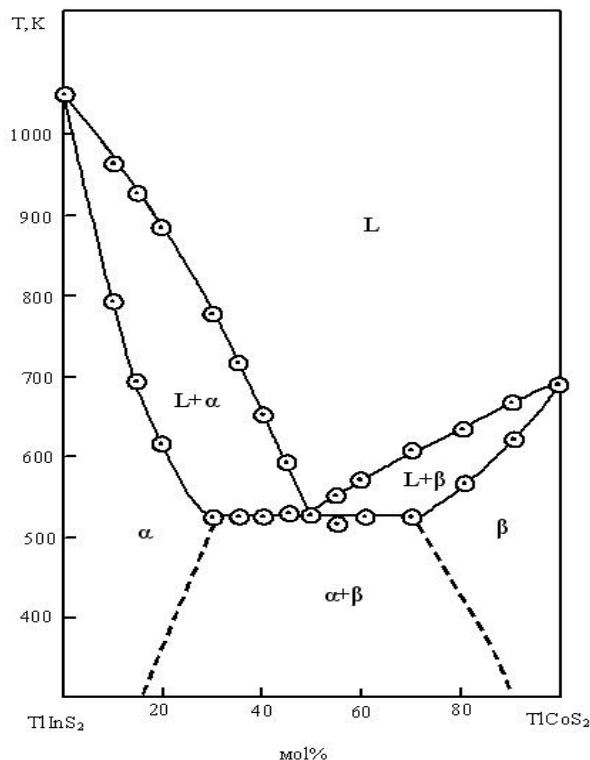
Fig.10. \text{TlInS}_2\text{-TiCoS}_2 system state diagram.
