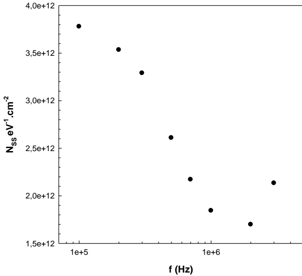
Fig.4. The variation of interface state density N_{ss} for Au/SrTiO 3 /n-Si SBD at room temperature.
