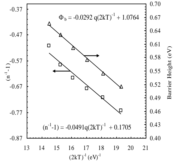
Fig. 6. The barrier height and ideality factor versus 1/T curves according to Gaussian distribution of the barrier heights
