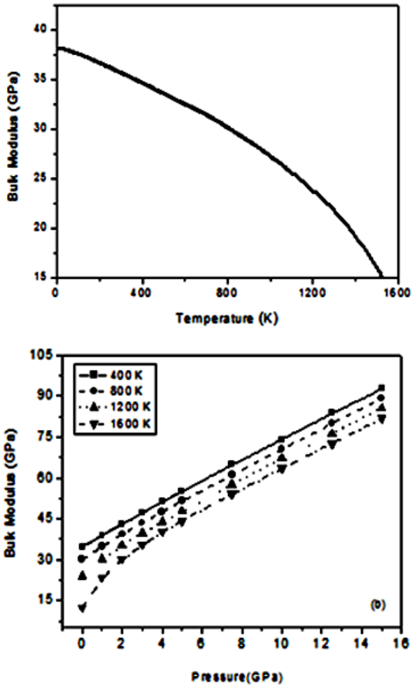
Fig. 2. (a) Bulk modulus as a function of temperature up to 1600K at zero pressure (b) Variations with pressure of the bulk modulus at different temperatures.
