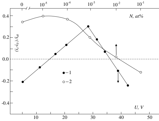
Fig. 2. Dependence of \frac{i_s - i_{s0}}{i_{s0}} on the applied voltage (curve 1) and doping level (curve 2) in p\text{-GaSe}\langle\text{Ho}\rangle crystals N , at. %: 1 - 10^{-4} ; U , V: 2 - 35; T = 77 K
