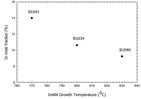
Fig. 6. InAlN Growth Temperature dependent In mole fraction
