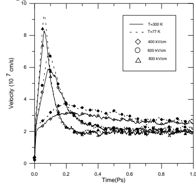
Fig.1 The electron drift velocity for bulk ZnO for various applied electric fields and the temperature of T=77 K (filled symbols with dashed lines) and T=300 K (empty symbols with lines).
