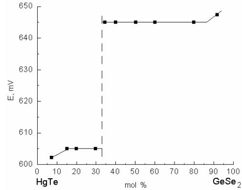
Fig. 4. Dependence of e.m.f. on composition in the HgTe–GeSe 2 system at 298 K.
