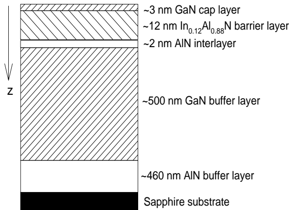
Fig. 1. Layer structure of the investigated samples.
