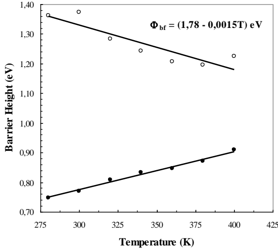
Fig. 4. Temperature dependence of zero-bias barrier height and flat-band barrier height for Au/ PVA (Co, Ni-doped)/n-Si Schottky diodes.
