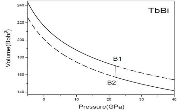
Fig. 2. Pressure versus volume curve of TbBi
