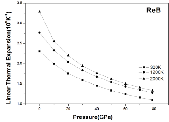
Fig. 8. The thermal expansion versus pressure for ReB.
