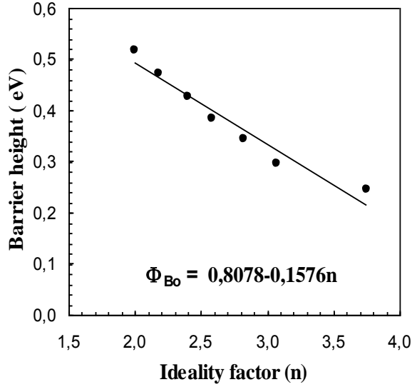
Fig. 3. Linear variation of apparent barrier height versus ideality factors at various temperatures.
