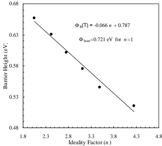
Fig.3. The barrier height vs. ideality factor with temperature
