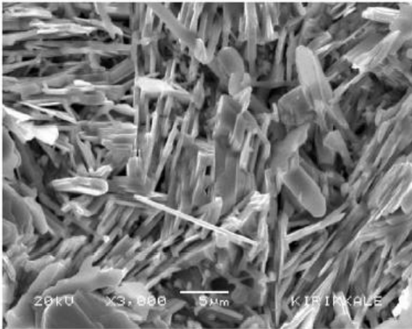
Fig. 2. SEM micrographs of the sample
