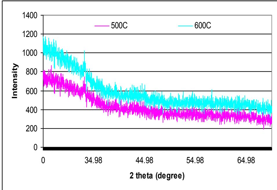
Fig. 2. The X-ray diffractograms of iron oxide thin films deposited at 500 0 C and 600 0 C substrate temperature.
