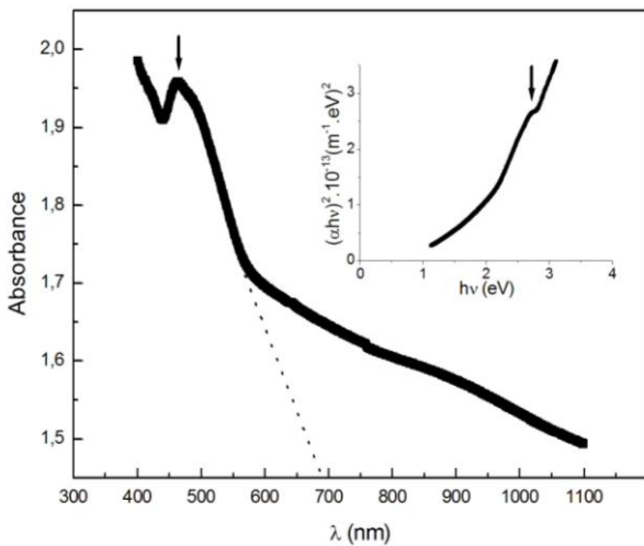
Fig.4. The optic absorption spectrum of MnS film grown on glass substrate.
