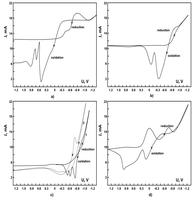
Fig. 1. Cyclic voltammogram for (a) 0.01M CdCl 2 , (b) 0.09M ZnCl 2 , (c1) 0.02M Na 2 S 2 O 3 , (c2) 0.08M Na 2 Se 2 O 3 and (d) mixture of (a), (b) and (c) solutions at room temperature.
