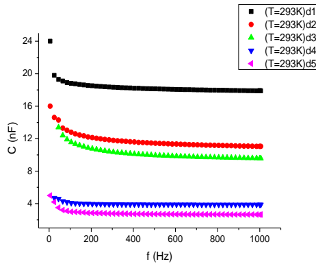
Fig.7. Variation of the capacitance with frequency of TlSb 2 thin films at different thickness. d_1 < d_2 < d_3 < d_4 < d_5
