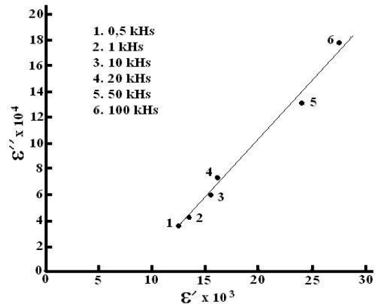
Fig.3. Cole-Cole plot of the complex dielectric constant of TlGaTe 2
