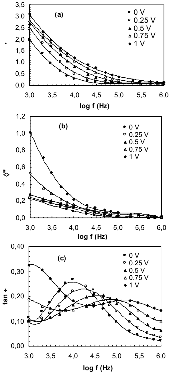
Fig. 2. Frequency dependence of the (a) \epsilon' , (b) \epsilon'' and (c) \tan\delta for various applied voltage of Au/n-GaAs (MS) structure.
