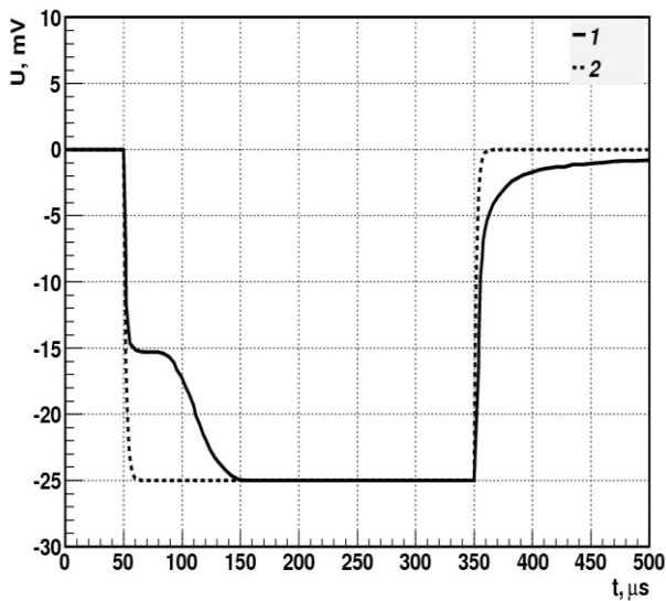
Fig.2. Oscilloscope picture of MC APD (1) and regular APD (2) photoresponse to 300 μs long light pulses. Applied voltage was equal to 20 V and gain was equal to 1.
