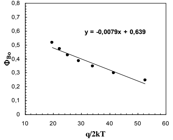
Fig. 5. The plot of \Phi_{B0} versus q/2kT for n-GaAs structure.
