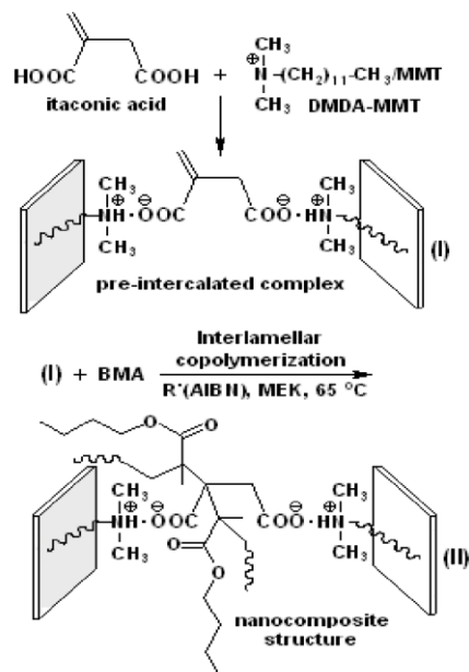
Fig.2. Intercalative complex-radical copolymerization of monomer complex of IA-COOH...N(CH 3 ) 2 -DMDA-MMT with n -butyl methacrylate (BMA): (I) structure of pre-intercalated monomer complex and (II) poly(IA- co -BMA)/O-MMT nanocomposite.
