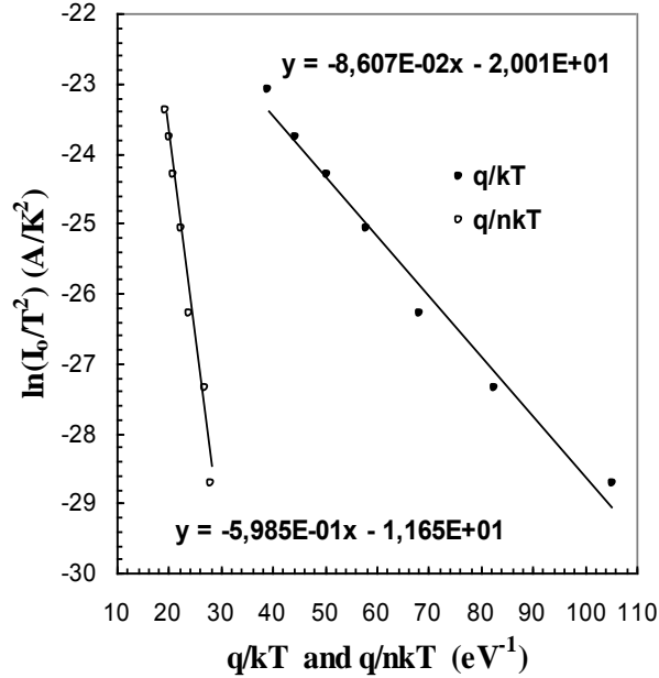
Fig. 4. The plot of \ln(I_0/T^2) vs q/kT and q/nkT for n-GaAs structure.
