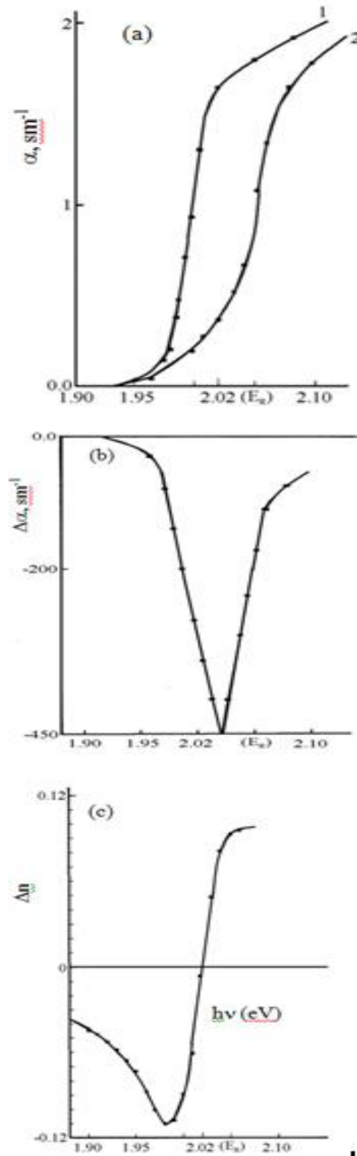
Fig. 2. (a) Absorption spectra of GaSe at low ( \sim 3.5 \text{ MW/cm}^2 , curve 1) and high ( \sim 12 \text{ MW/cm}^2 , curve 2) intensity excitation; (b) The change in the absorption coefficient \Delta\alpha ; (c) The change in the refractive index \Delta n(\omega) .
