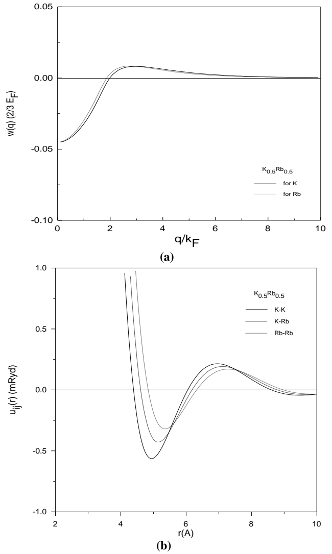
Fig. 1 Screened form factors of pseudopotential (a) and partial pair potentials (b) for K_{0.5}Rb_{0.5} liquid alloy at 373K.
