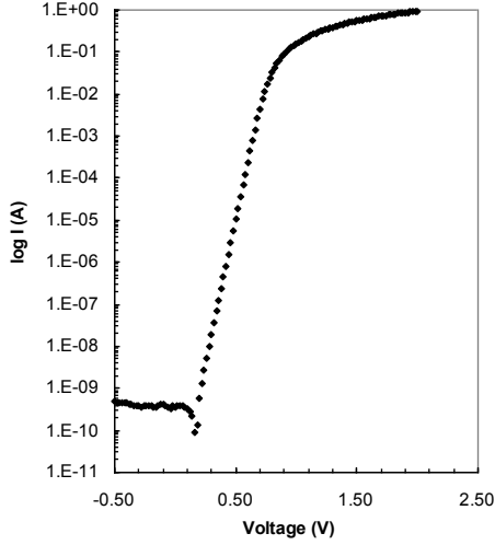
Fig. 1. Forward and reverse bias semi-logarithmic I - V characteristics of GaP Schottky diode at room temperature in darkness.
