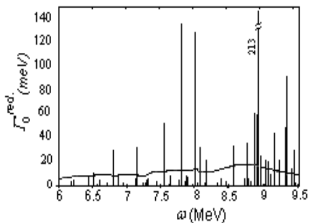
Fig.3. The reduced dipole ground-state transition widths for PDR (impulses) and for spin-flip resonance (the curved line) for ^{238}\text{U} .
