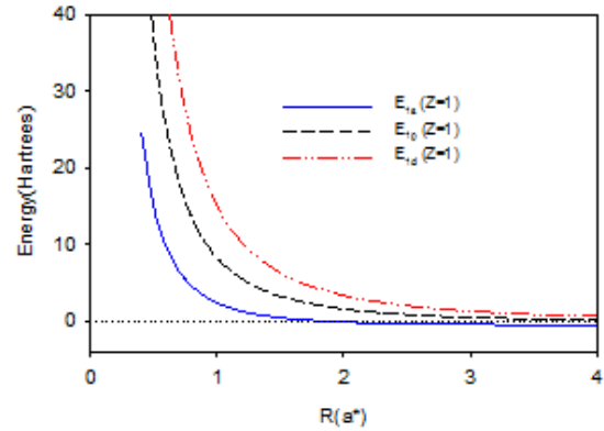
Fig. 1 Energies of the ground (1s), the first (1p) and the second (1d) excited states of a spherical QD with impurity as a function of dot radius.
