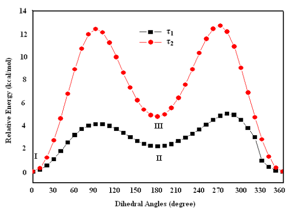
Fig. 2. Conformational energy profile for the rotation around the \tau_1 (N4, C13, C14, O2) and \tau_2 (H16, O1, C14, C13) angles of PAH
