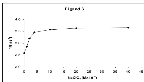
Fig.4. Spin-lattice relaxation rates versus concentration of Na+ ions for ligand 3
