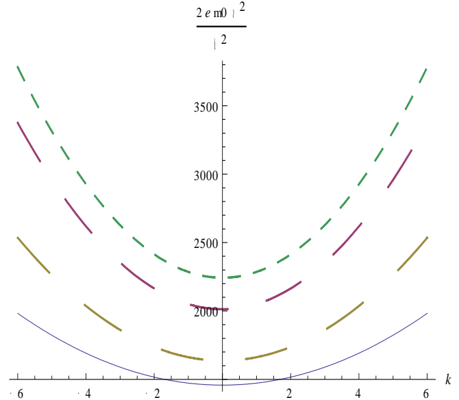
Fig.1. Energy spectrum of electrons as a function of wave number k for InSb.
