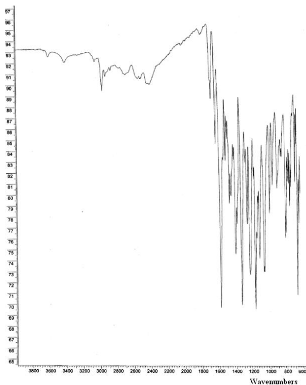
Fig. 3. FTIR spectrum of rhodamin-610.
