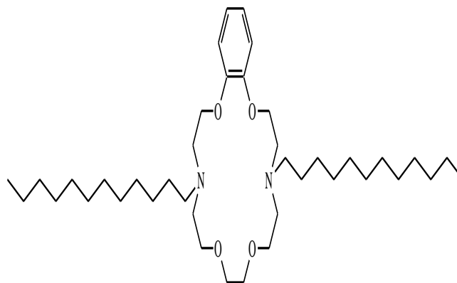
Fig.2. Ligand 2 N,N'-DiDodesil-7,16-diaza-1,4,10,13-tetraoksa-2,3-benzosikloktadek-2-ene
