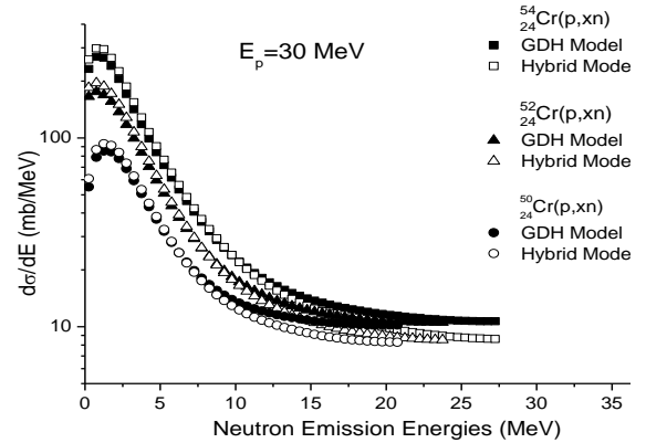
Fig. 2. Calculated neutron spectra from ^{50,52,54}\text{Cr}(p, xn) at 30 MeV.
