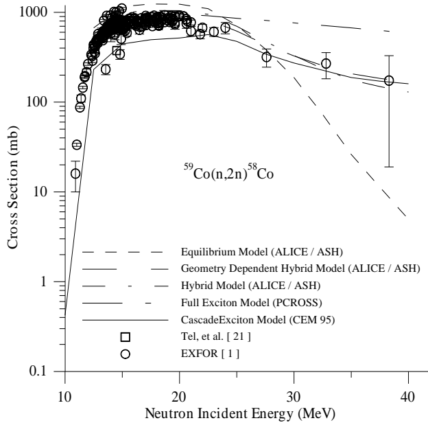
Fig.1. The comparison of calculated excitation function of ^{59}\text{Co}(n,2n)^{58}\text{Co} reaction with the values reported in [1].
