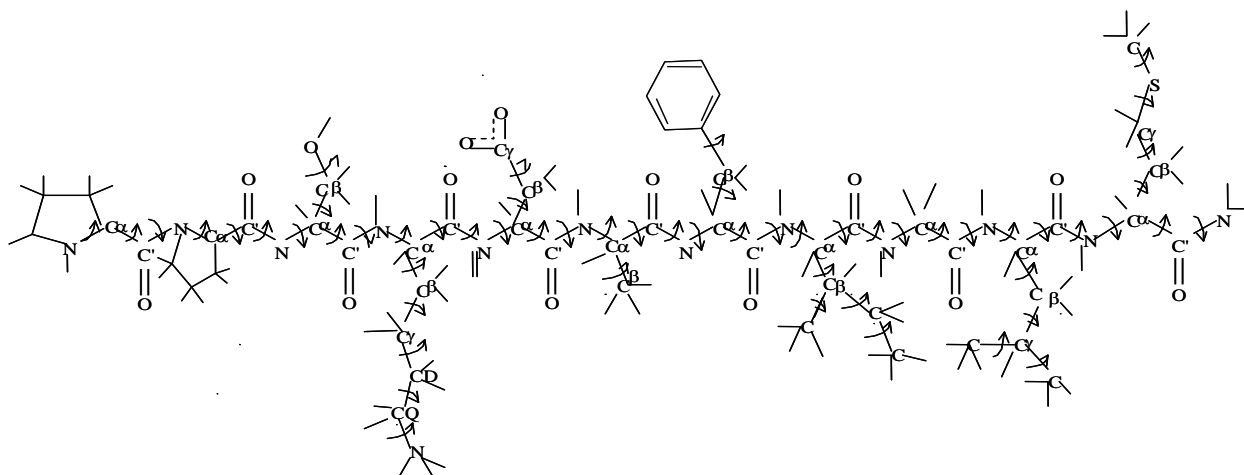
Fig.1. Atomic calculation model and variable dihedral angles of the eleodoisin molecule.
