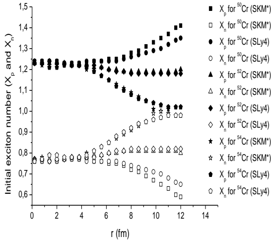
Fig. 1. Calculated density dependent initial neutron and proton exciton numbers for proton induced reaction on ^{50,52,54}\text{Cr} .
