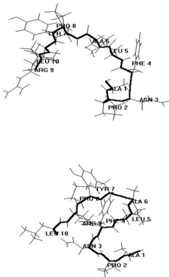
Fig.1. Atomic model of spatial structures of B_2RR_{11}B_2B_{22}B_2B_1BB_{1222}B_{21} ( U_{rel}=0 kJ/mol) of SCP(a) and B_2RR_{21}B_1R_{32}R_2B_1BB_{1222}B_{31} ( U_{rel}=3.8 kJ/mol) of SCP (b).
