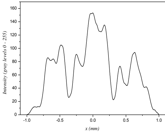
Fig.3. Profile of the interferogram for l = 0 along the horizontal direction.
