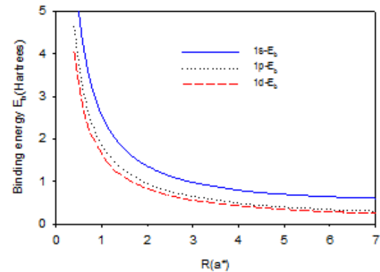
Fig. 2 Binding energy of the ground (1s), the first (1p) and the second (1d) excited states of a spherical QD as a function of dot radius.
