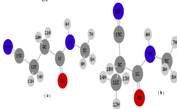
Fig. 1. The optimized molecular structures of C1 (a) and C2 (b) form at B3LYP/6-311+G(d,p) model.
