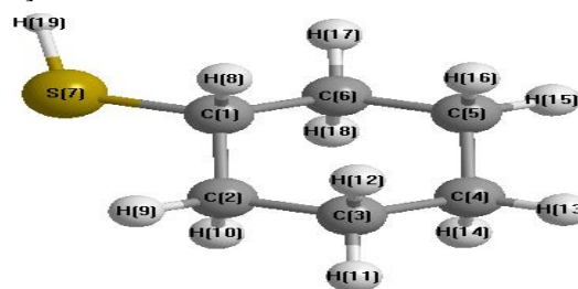
Fig. 2. The molecular structure of the CHT.
