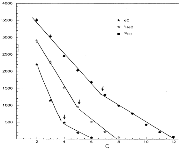
Fig.4 The number of dC -, HeC - and CC - reactions as a function of centrality at 4.2 A GeV/c.
