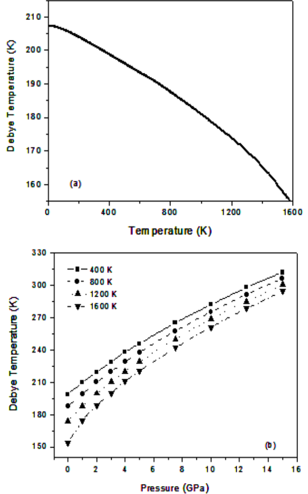
Fig. 3. (a) Debye temperature versus temperature for \text{La}_3\text{Tl} at zero pressure (b) Variations with pressure of the Debye temperature at different temperatures
