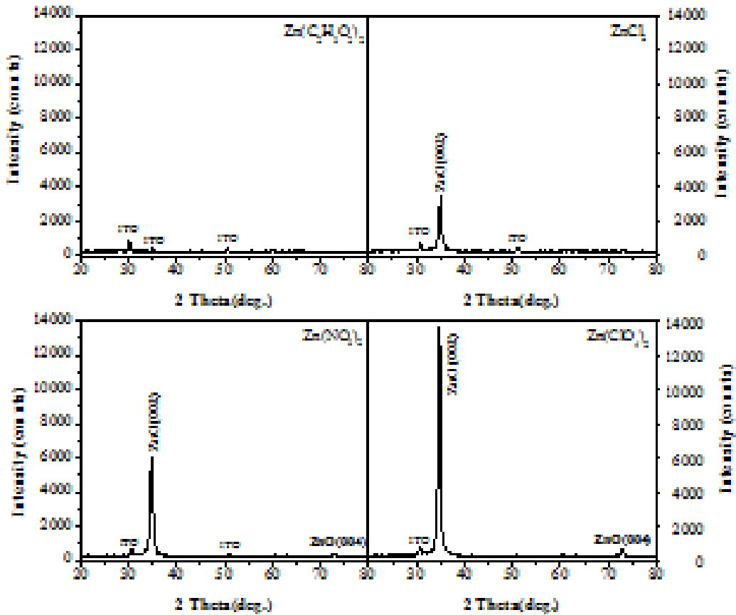
Fig. 2. XRD results of the ZnO thin films grown in DMSO
