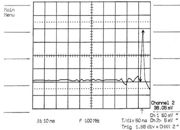
Fig.6. Oscillogram taken of the GaSe structure.
