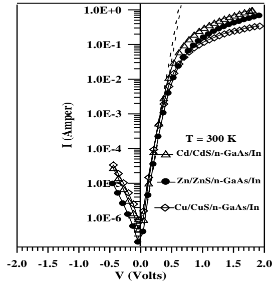
Fig.1. The semi-log forward bias current–voltage characteristics of sandwich structures at room temperature.
