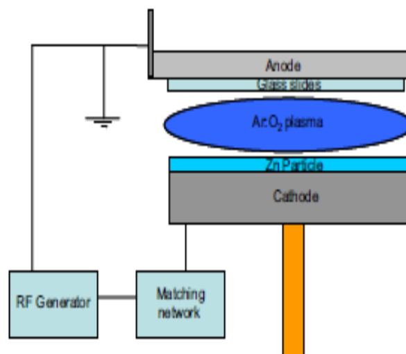
Fig. 1. Schematic of an reactive sputtering system[1].
