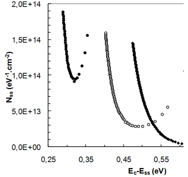
Fig.3. The energy distribution profile of N_{ss} obtained from the forward bias I-V characteristics of the Au/n-Si SBD with the native \text{SiO}_2 layer at different temperatures.
