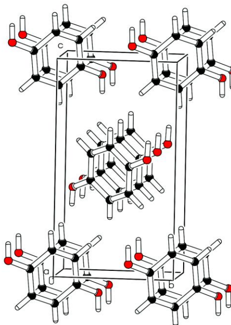
Fig. 2. The packing diagram of the title compound in the unitcell.
