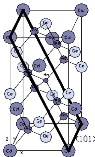
Fig.1. A scheme of \text{CdGeAs}_2 unit cell according to lattice parameters and atom coordinates in the unite cell (marked out a crystallographic plane (101), were obviously can be the Mn atom)
