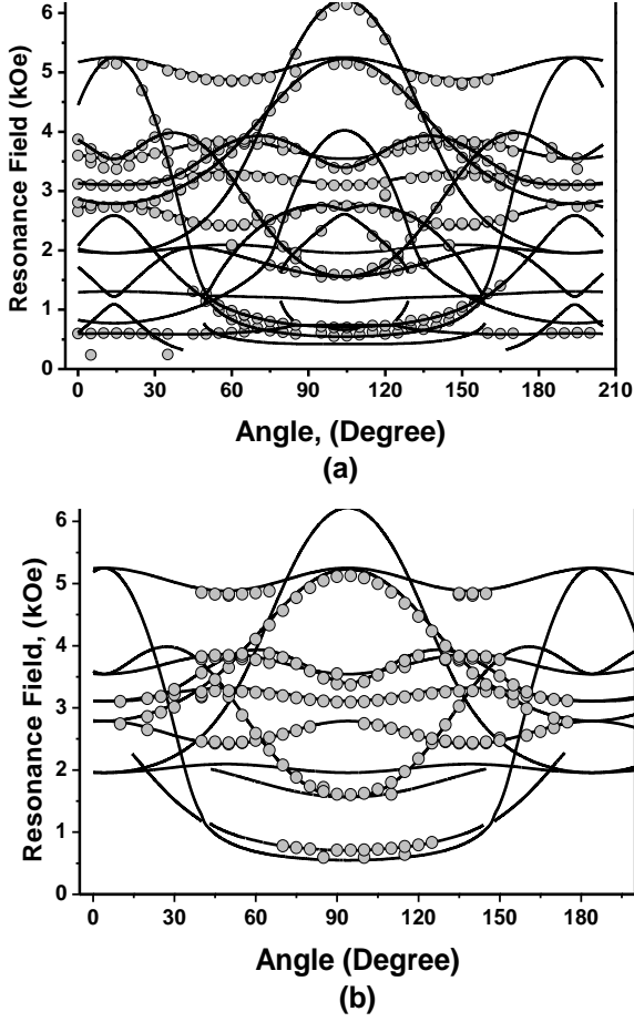
Fig.3. (a) Angular dependence of resonance field at 215 K for the rotation of magnetic field in (100) plane of single crystalline BaTiO 3 . (b) Angular dependence of resonance field at 220 K for the rotation of magnetic field in (001) plane of single crystalline BaTiO 3 . The solid circles show the experimental position of each resonance line in EPR spectra. The solid lines show the simulation of angular behaviors of the resonance lines.
