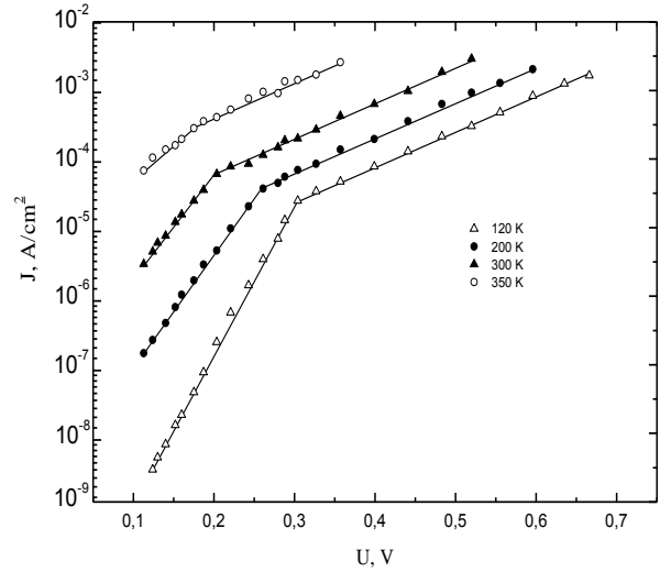
Fig.3. Semilogarithmic plot of forward bias of J-V curves for p- GaAs/n-Cd 1-x Zn x S 1-y Se y heterojunctions at different temperatures.
