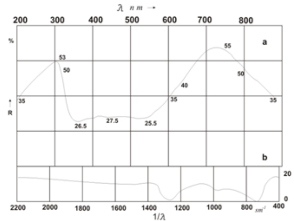
Fig.1. The reflections spectrums of p-CuAgTe a- in range 1.0 \div 6.2 eV; b- in range 0.05 \div 0.50 eV
