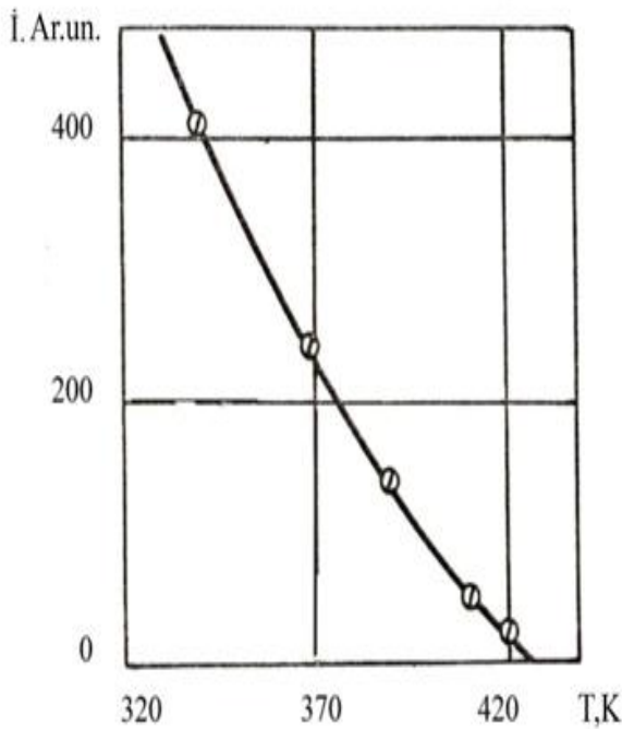
Fig.2. Temperature dependence of relative intensiveness of ESR lines of Co_{0,7}Cu_{0,3}Cr_2S_4 .
