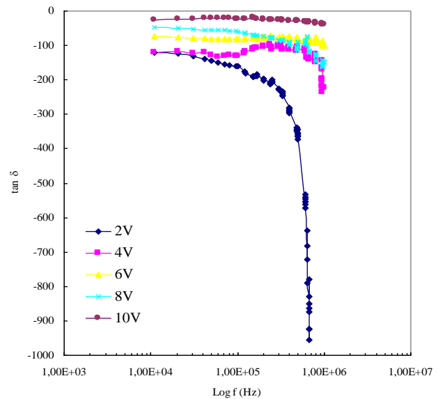
Fig. 5. Plot of dielectric loss ( \tan \delta ) versus frequency at different voltages
