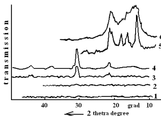
Fig. 1. The diffraction patterns of PP and composites on its basis and PZT-4. 1. PP + PZT-4, \Phi=50\% ; 2. PP + \text{CaTiO}_3 , \Phi=40\% ; 3. PP + \text{CaTiO}_3 , \Phi=10\% ; 4. PP + PZT-4, \Phi=10\% ; 5. PP – slowly cooled; 6. PP – hardened.
