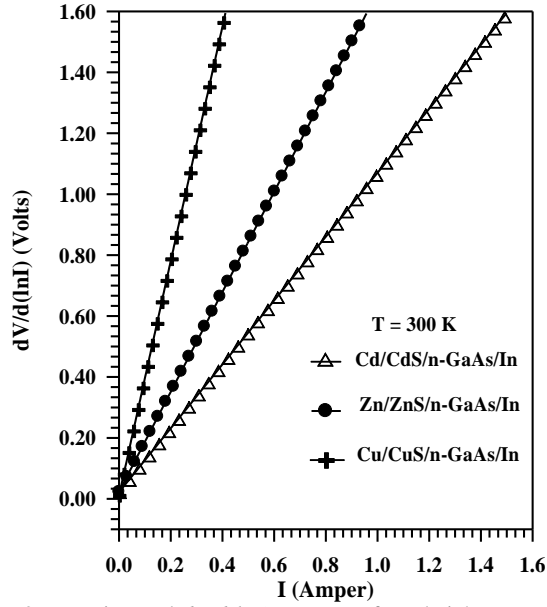
Fig. 2. Experimental dV/d(lnI)-I curves of sandwich structures
