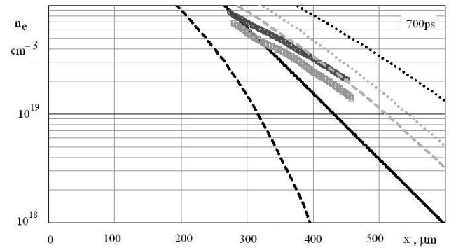
Fig.5. The dependences of electron density (rings for shot #7 and squares for shot # 10), calculation from the 1D self-similar model (solid straight lines), results of 1D MULTI simulation: with LTE (grey), without LTE (black), with account of radiation transport (dashed), without account of radiation transport (dotted).
