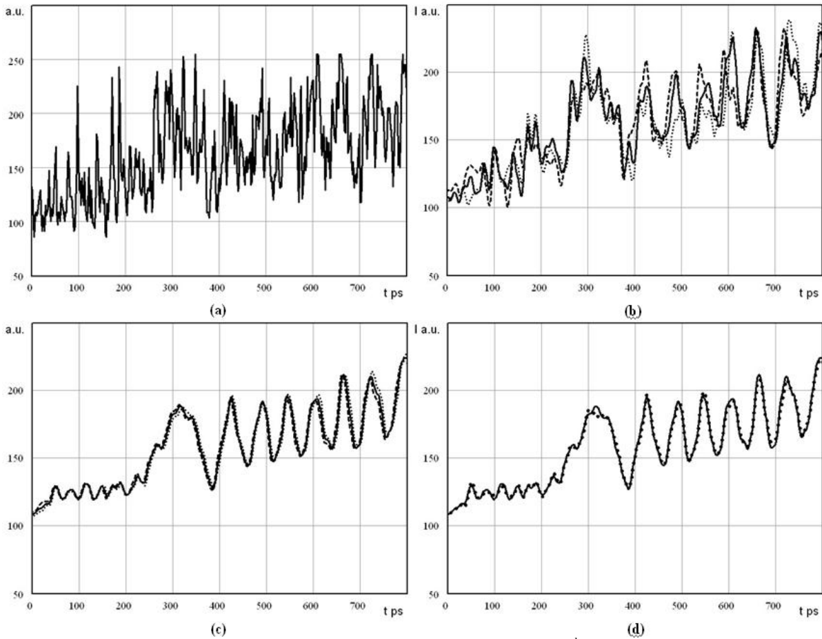
Fig. 3. (a) Time-dependence of intensity of a streak-camera image (Au, shot #7, for the 3 rd minimum from the right, that is 320 pixel from the left). (b) The Gauss-filter application for the line on fig.a (solid line) and for the neighbour intensity lines, corresponded to 319 pixel (dotted line) and 321 pixel (dashed line). (c) The same but with the prior time-shift averaging in the spatial interval \pm 10 pixels ( 7.3 \mu\text{m} ) with characteristic velocity 3.5 \cdot 10^7 \text{ cm/sec} . (d) Time-shift averaging in the spatial interval \pm 7.3 \mu\text{m} (10 pixels). The dotted line corresponds to characteristic velocity 4.6 \cdot 10^7 \text{ cm/sec} , the solid line to 3.5 \cdot 10^7 \text{ cm/sec} , finally a time Gauss-filter has been applied.
