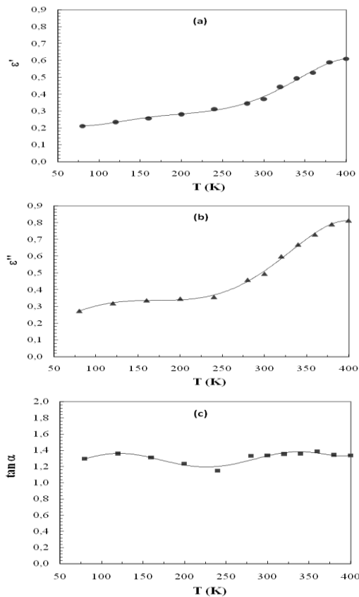
Fig. 2. Temperature dependence of the (a) \epsilon' , (b) \epsilon'' and (c) \tan \alpha of Au/ PVA(Co, Ni-doped)/n-Si structure
