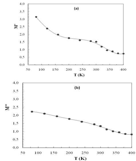
Fig. 4. (a) The real part M' and (b) the imaginary part M'' of electric modulus M^* vs temperature for Au/ PVA(Co, Ni-doped)/n-Si structure.
