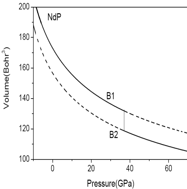
Fig. 2. Pressure versus volume curves of NdP
