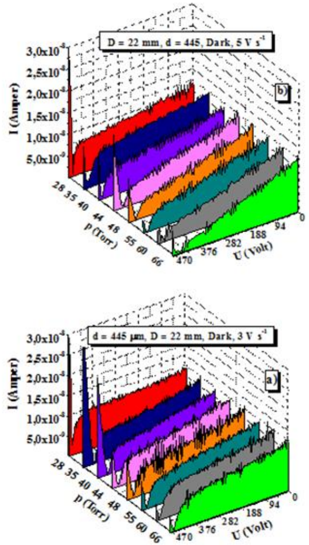
Fig.2. CVC of a planar discharge cell with respect to pressure (a) 3 \text{ Vs}^{-1} rate of ramping applied voltage per unit time, (b) 5 \text{ Vs}^{-1} rate of ramping applied voltage per unit time. System parameters; D = 22 mm, d = 445 \mu\text{m} and in darkness.
