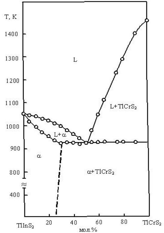
Fig.6. \text{TlInS}_2 - \text{TlCrS}_2 system state diagram.
