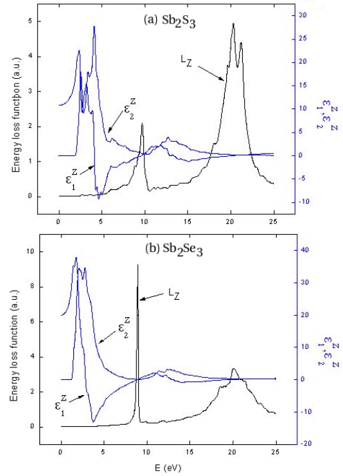
Fig. 2. Energy spectra of dielectric function \epsilon = \epsilon_1 - i\epsilon_2 and energy-loss function (L) along the z-axes for Sb_2S_3 and Sb_2Se_3 .
