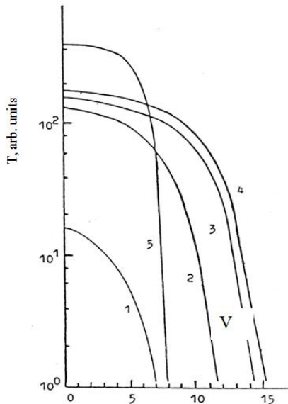
Fig. 5. Intensity of laser radiation with wavelengths of (1) - 625 nm, (2) - 629nm, (3) - 632,8nm, (4) - 634nm and (5) - 1060nm transmitted through the attenuator (GaSe crystal - 1-4; InSe crystal - 5) as a function of constant voltage applied to the device.
