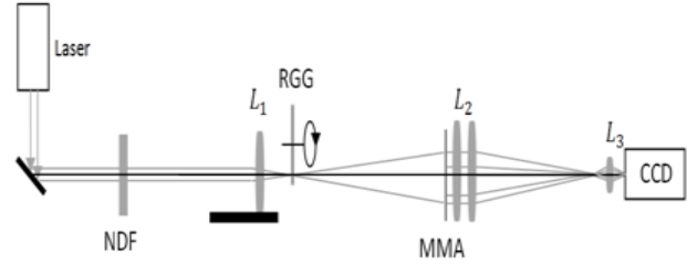
Fig.1. Experimental set-up to measure the complex degree of spatial coherence.
