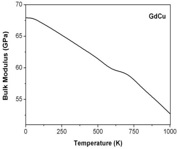
Fig.4. The bulk modulus (B) for GdCu as a function temperature T at P=0.
