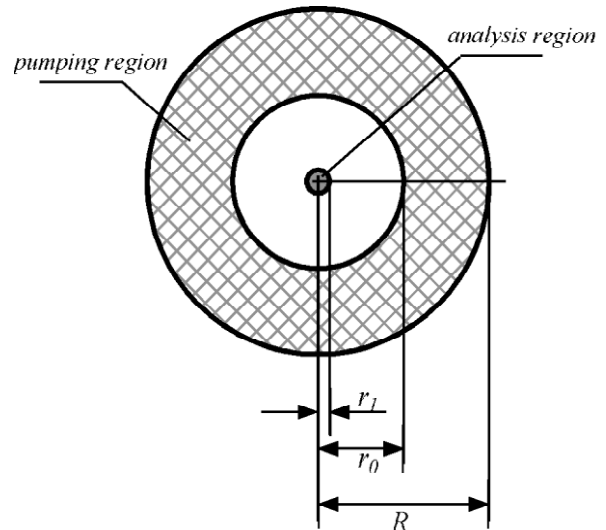
Fig.3. Irradiation of the thin gas cell (in the axial direction) by a monochromatic laser beam, having the ring-shaped cross-section with the external radius R and the inner radius r_0 . The excited state population is probed by a second laser beam in the central region of radius r_1 .
