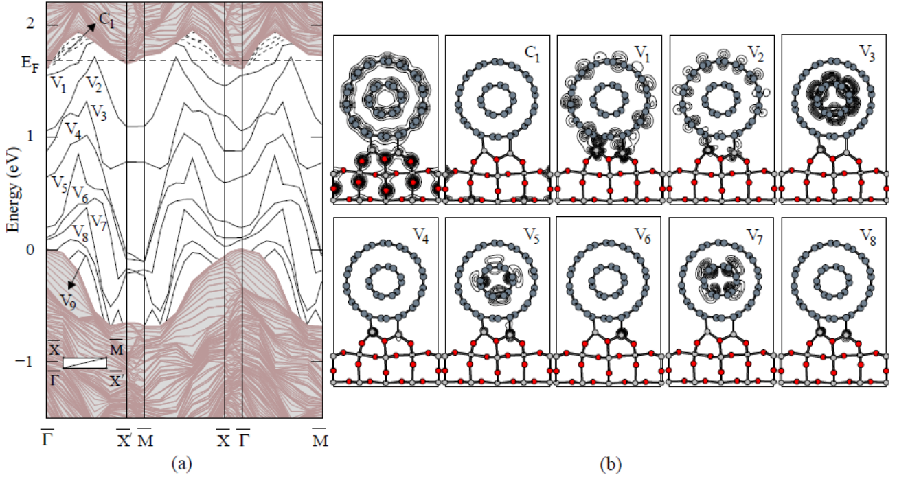
Fig. 2. (a) The surface electronic band structure for the (3,3)-in-(7,7) DWCNT adsorbed on the ORAR rutile surface. (b) The first one is the total electronic charge density, the others are electronic charge density plots for the individual gap states.
