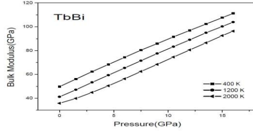
Fig. 8. The relationships of TbBi between bulk modulus (B) and pressure P at temperatures of 400 K, 1200 K, 2000 K
