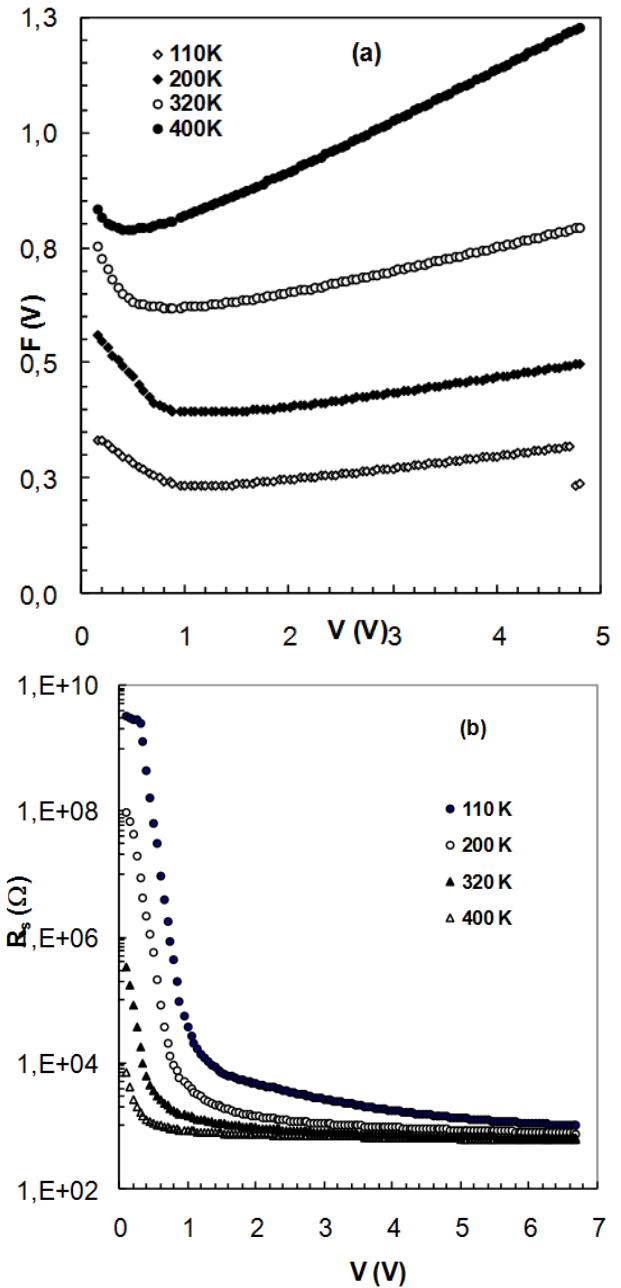
Fig.2. The F(V) vs V and R_s vs V plots of the Au/n-Si(111) SBDS with native insulator layer at four temperatures, respectively.
