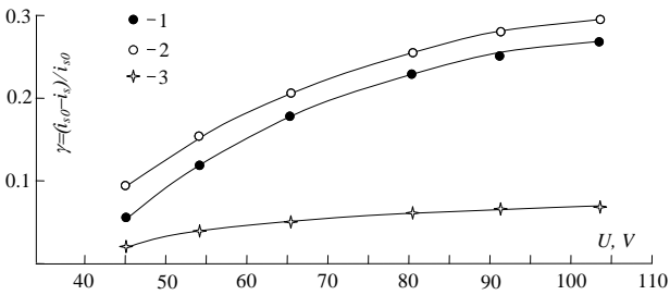
Fig. 3. Dependence of \gamma = \frac{i_{s0} - i_s}{i_{s0}} on voltage in p\text{-GaSe}\langle\text{Ho}\rangle crystals with different level of doping N , at. %: 1 - 0; 2 - 10^{-4} ; 3 - 10^{-1} ; T = 77 K
