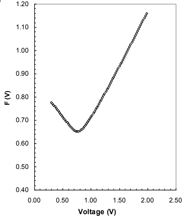
Fig. 3. F(V) vs. V plot of the Au/n-GaP Schottky barrier diode.
