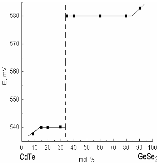
Fig. 3. Dependence of e.m.f. on composition in the CdTe–GeSe 2 system at 298 K.
