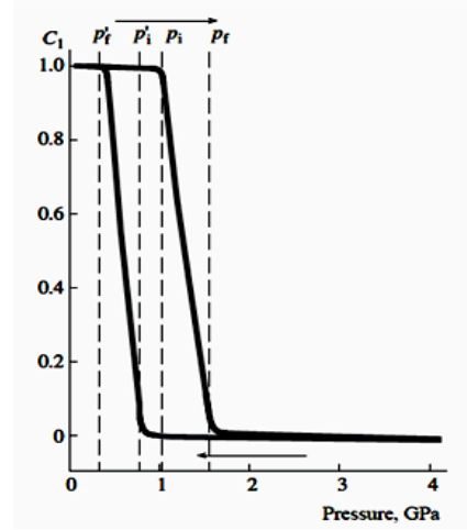
Fig. 4. Volume fraction of phase 1 as a function of pressure for p-Cd 1-x Mn x GeAs 2 with x = 0.06 .
