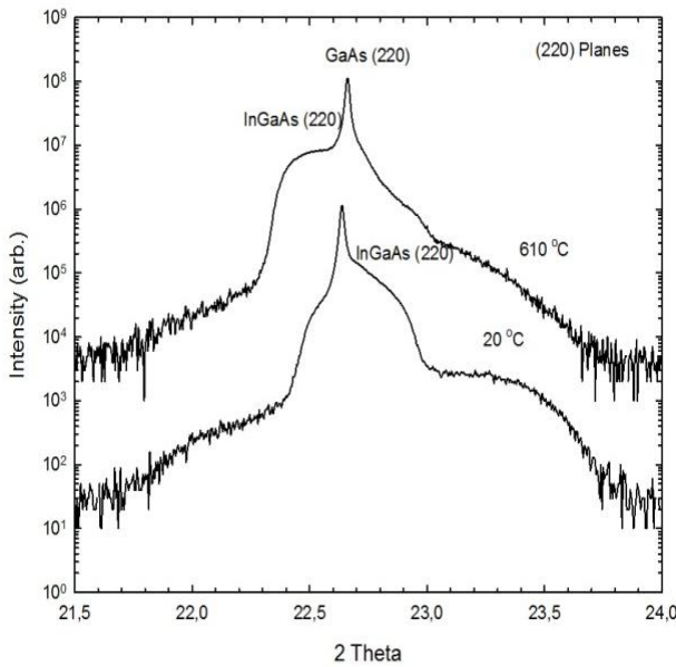
Fig. 2. The \omega/2\theta scans of InGaAs/GaAs QWSCs.
