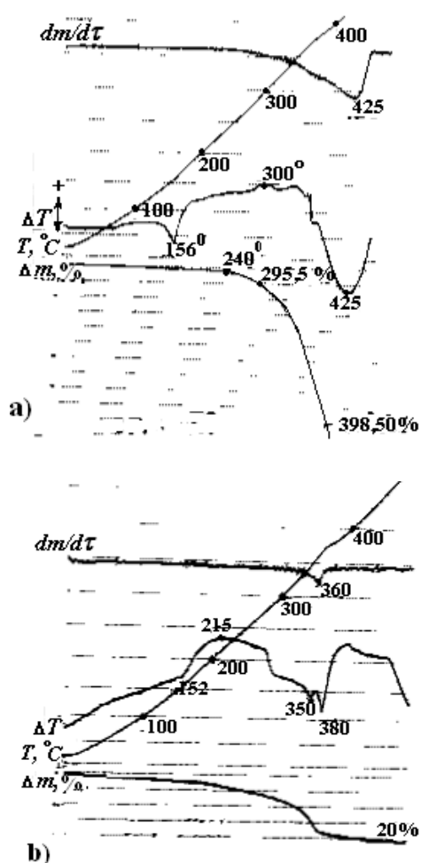
Fig. 6. Derivatogram polymer composites: a - PP; b - PP+50% vol. PZT-4.
