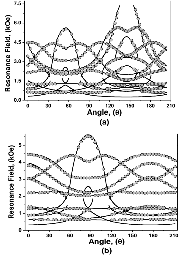
Fig.1. The observed and fitted rotation patterns of the EPR resonance field values of BaTiO 3 substrate possessing Fe impurities for “in-plane” (a) and “out-of-plane” (b) geometries. Full curves are calculated using the obtained spin-Hamiltonian parameters.
