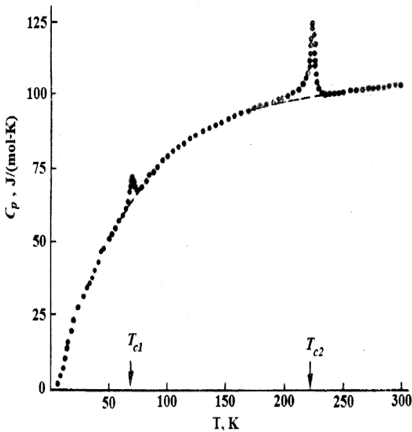
Fig.1 Dependence C p (T) for TlFeTe 2
