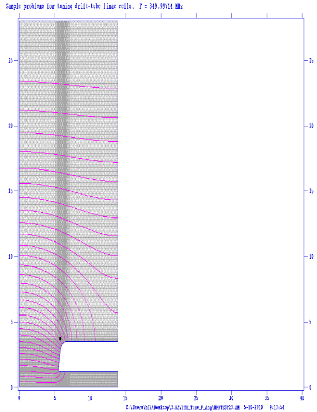
Fig 4. Sample DTL and maximum surface electric field shape for g=11.0 cm
