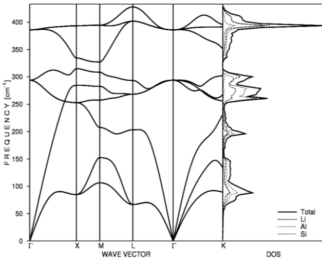
Fig. 3. The calculated phonon dispersions and total and partial density of states for arrangement II.
