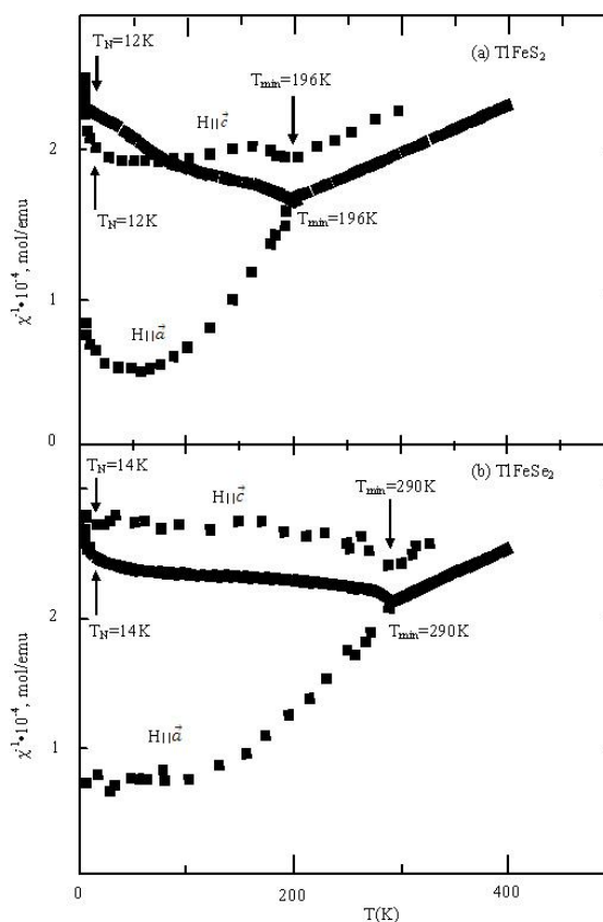
Fig.4. The temperature dependence of the inverse magnetic susceptibility of \text{TlFeS}_2 (a) and \text{TlFeSe}_2 (b). (Figure with our comments corresponds to publication [12].)
