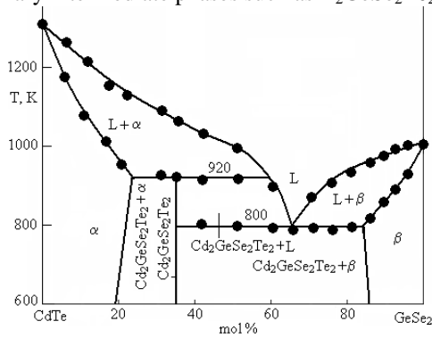
Fig. 1. Phase diagram of the CdTe-GeSe 2 system.
