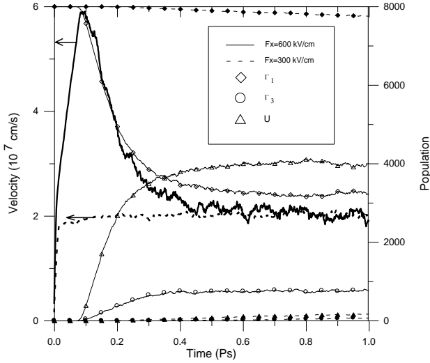
Fig.2 The drift velocity and \Gamma_1 , \Gamma_3 , U valley occupancies at applied two different electric fields F_x= 300 kV/cm (solid symbols) and F_x= 600 kV/cm (empty symbols) for bulk ZnO at room temperature.
