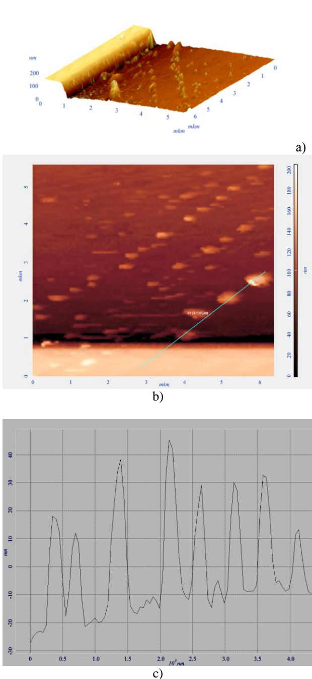
Fig.2(a, b, c) SPM images of surface (0001) \text{Bi}_2\text{Te}_3\langle\text{Cu}\rangle : a) SPM images of \text{Bi}_2\text{Te}_3\langle\text{Cu}\rangle in 3D-scale, b) Image of step and nanoprotusions in 2D scale, c) step profile along light horizontal line on the part of Fig.2(b).
