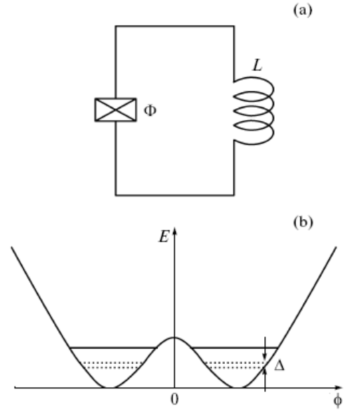
Fig. 2. Single quantum superconducting interferometer as a phase qubit: (a) equivalent circuit diagram; (b) symmetric double well potential.
