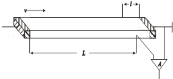
Fig. 1. The structure of the SPRITE detector. + U - plus DC bias voltage, L - band drift NCC, l - the zone read, A - signal processing circuit, v - velocity of ambipolar diffusion and scanning, v = v_a = v_s
