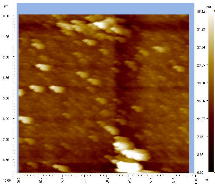
Fig. 3-b AFM image of iron oxide nano thin films at 600 °C.
