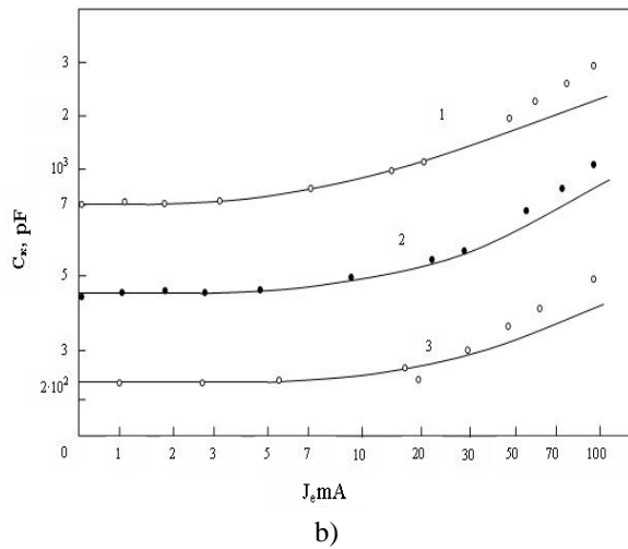
Fig.2. The dependence of barrier capacitance of collector junction of TC(a) and TG(b) on emitter current for various U_{rev} (300K, f=100 kHz): 1-1V; 2-6V; 3-50V; 4-4V; 5-10V; points – experimental data, curves – calculated data.
