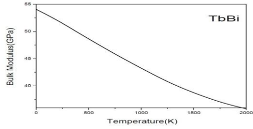
Fig. 7. The bulk modulus (B) for TbBi as a function temperature T at P=0
