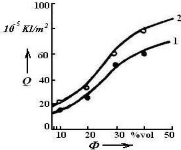
Fig. 8. The dependence of the boundary charge of the composite PP - PZT-4 from the bulk PZT-4. 1- spheruliteless; 2- spherulitic.
