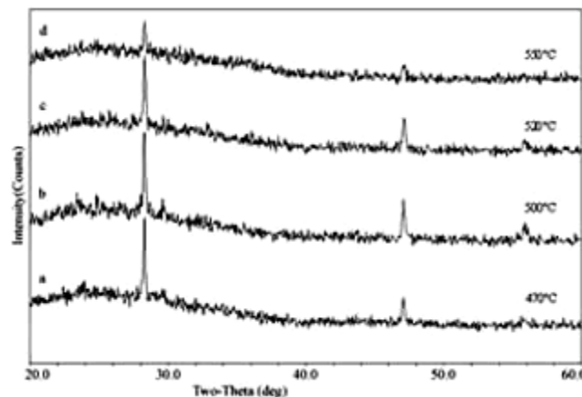
Fig.2. X-ray diffraction spectrums of Ga_2Se_3 thin films prepared by sol-gel method.
