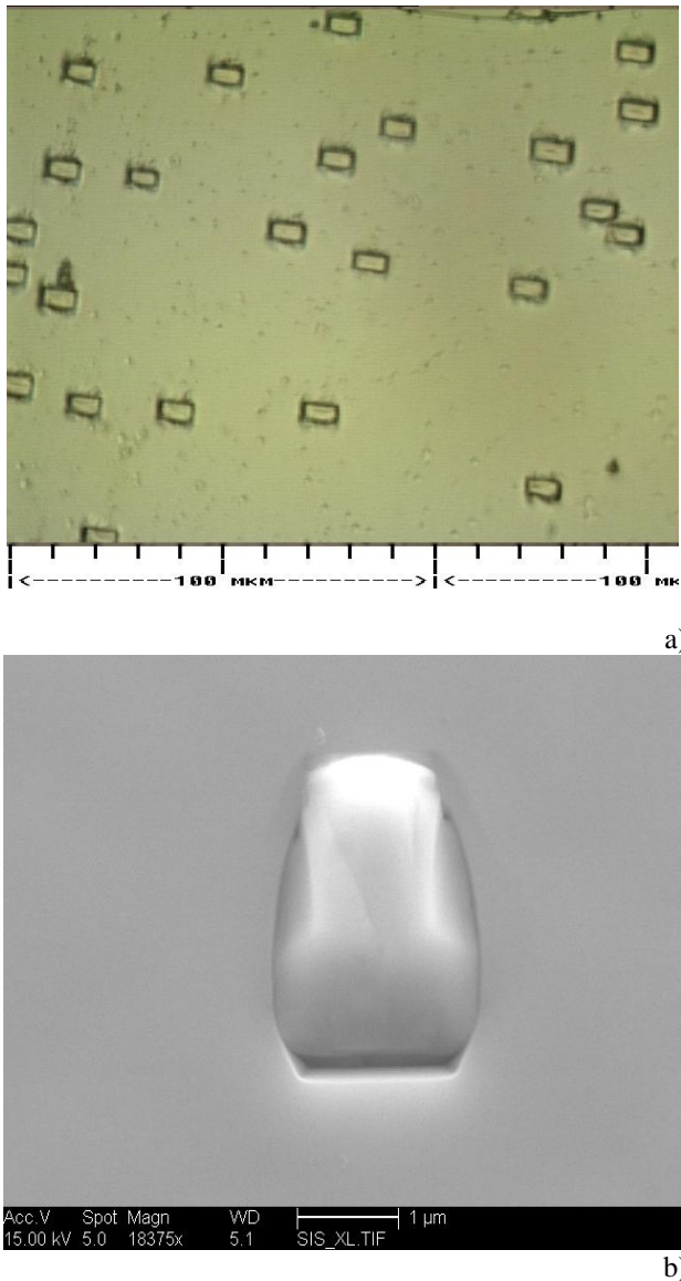
Fig.3. Images of microcrystallites in GaInAsPSb epitaxial layers. Images were taken by optical microscope (a) and electron microscope “CamScan” (b).
