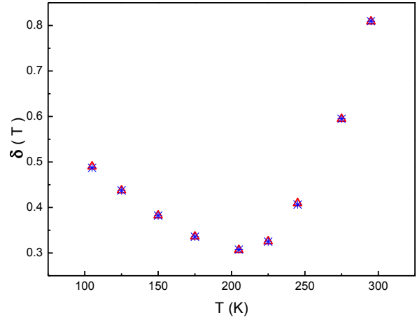
Fig. 5. The exponent \delta vs temperature for CdTe(Sb) for two values of relaxation times (20 s and 120 s). Curves were recorded after 70 seconds lightening and with bias voltage 3 volts.
