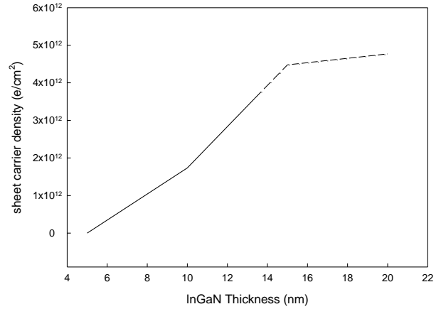
Fig.4. Sheet carrier density in different InGaN thickness for 5, 10, 15, 20 nm. Dashed lines represent the strain relaxed situation.
