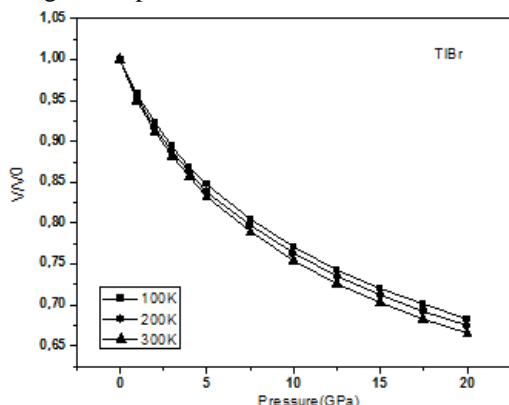
Fig. 3. The normalized volume-pressure diagram of the B2 structures for TlBr at different temperatures.
