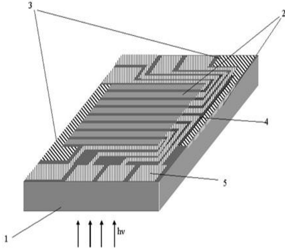
Fig. 3. SPRITE-detector on the base of epitaxial layer. 1 – substrate, 2 – epilayer, 3- current contact, 4 – dielectric layer, 5 read-out contacts.
