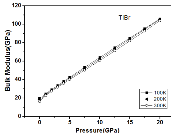
Fig. 4. The relationships of TlBr between bulk modulus and pressure P at temperatures of 100, 200 and 300 K for TlBr.
