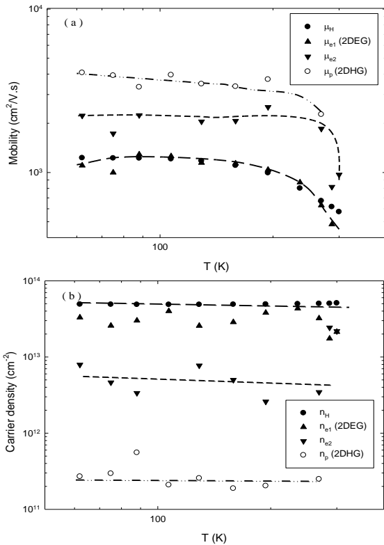
Fig. 2. (a) Mobility and (b) carrier density versus temperature. The closed circles represent the measured mobility and carrier density taken at 0.5 Tesla. The triangles represent the extracted 2DEG mobility and carrier density. The open circles represent the extracted 2DHG mobility and carrier density. The stars and squares represent the bulk carriers. The lines are guide for the eyes.
