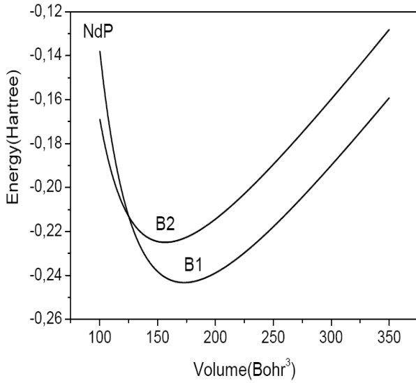
Fig. 1. Total energy versus volume curves of NdP
