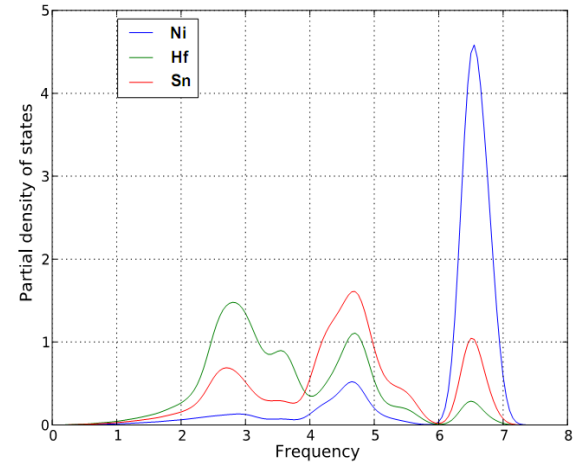
Fig. 5. Partial phonon density of states for NiHfSn compound.
