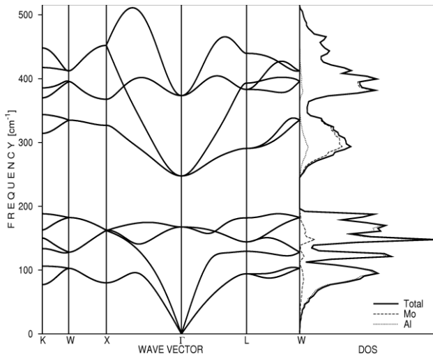
Fig. 3. The calculated phonon dispersions and total and partial density of states for MoAl in B32 structure
