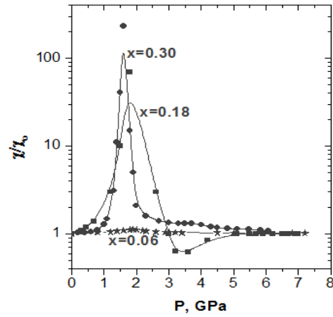
Fig.5. Baric dependence of relative magnetic susceptibility for Cd 1-x Mn x GeAs 2 ( x=0.06, 0.18, 0.30 ) samples.
