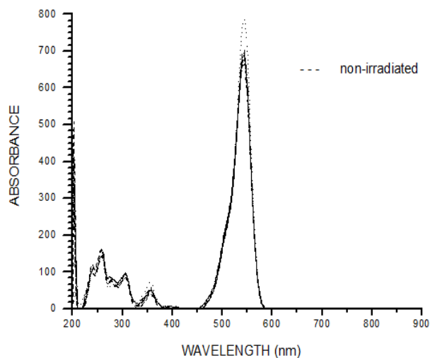
Fig.4. Photochemical change in rhodamin-610 from 0 to 10 hours at room temperature
