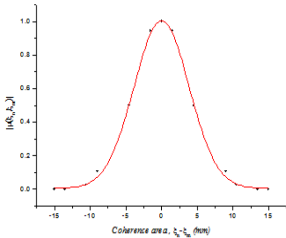
Fig.5. Modulus of the complex degree of spatial coherence vs. coherence area.
