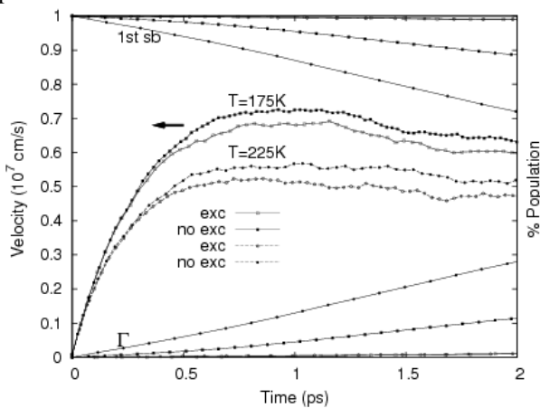
Fig.5. The occupancy of energy sub bands and three dimensional valleys with regard to temperature. Empty circles and squares are when exchange is included and filled circles and squares are when it is not. It appears that the temperature almost has no effect on the occupancy of the levels in the temperature range considered here , but rather the exchange potential is more responsible for holding the particles in two dimensions.
