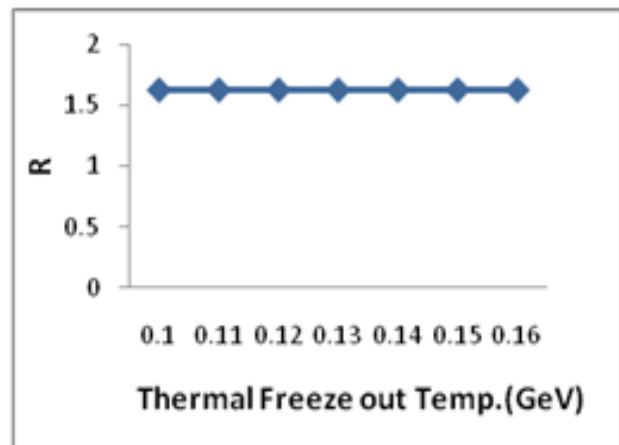
Fig.5 Dependences of nuclear modification factor on different variables
