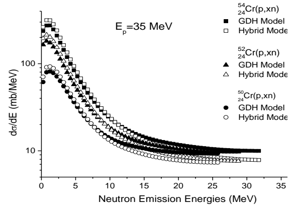
Fig.3. Calculated neutron spectra from ^{50,52,54}\text{Cr}(p, xn) at 35 MeV.
