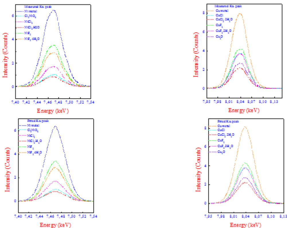
Fig. 2. Measured and fitted K\alpha lines by Voight function for Ni and Cu compounds.
