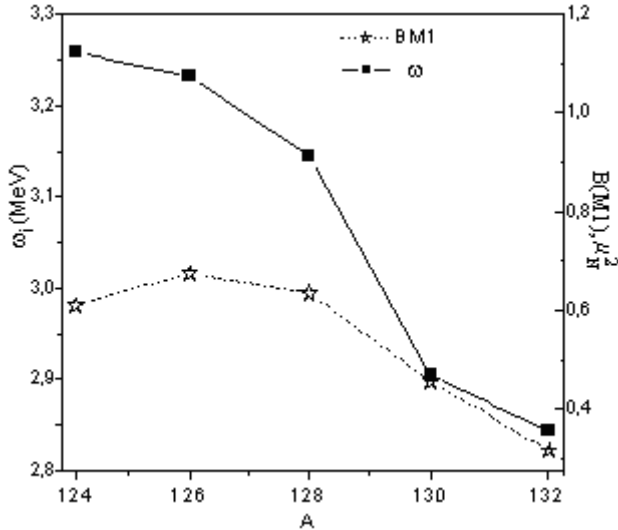
Fig.1. Variation of the lower 1^+ states with B(M1) > 0.3 \mu_N^2 versus mass number A .
