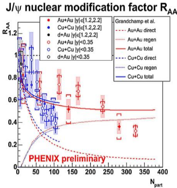
Fig.8 The values R_{AA} as a function of N_{part} for heavy flavor coming from RHIC.
