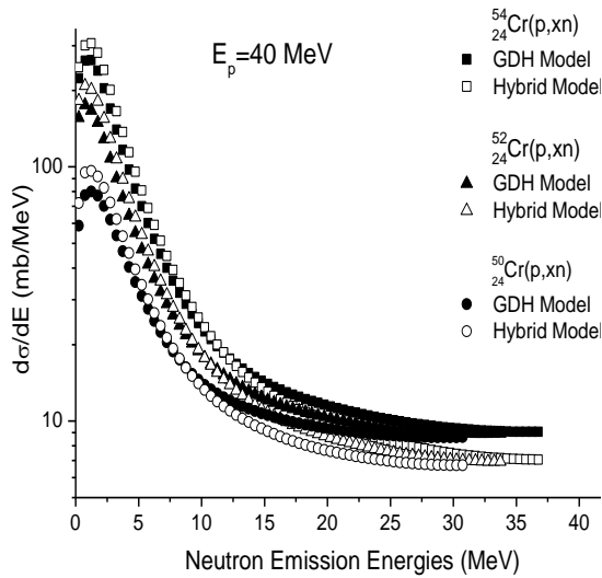
Fig. 4. Calculated neutron spectra from ^{50,52,54}\text{Cr}(p, xn) at 40 MeV.
