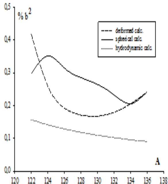
Fig. 2. Isospin admixture in the ground state for investigated isotopes.
