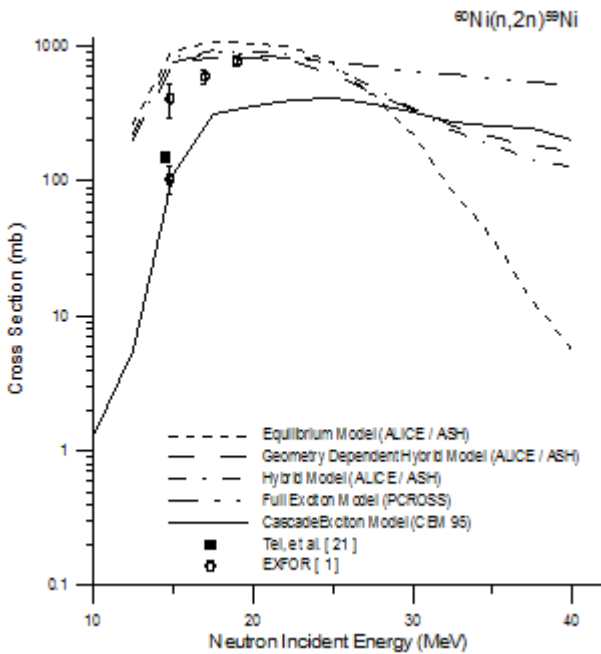
Fig.2. The comparison of calculated excitation function of ^{60}\text{Ni}(n,2n)^{59}\text{Ni} reaction with the values reported in [1].
