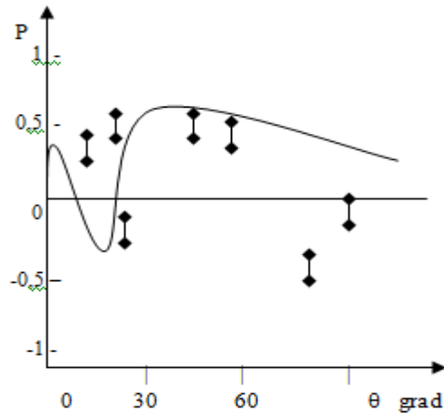
Fig.1 The polarisation of the neutron in n^{12}C scattering.
