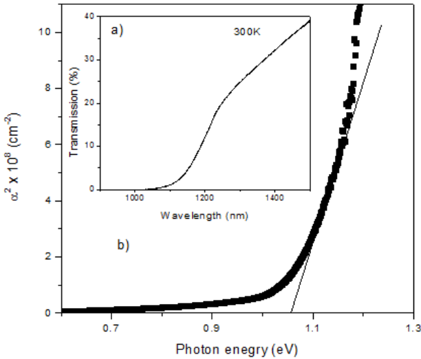
Fig. 5. Transmittance (a) and the dependence of \alpha^2 vs h\nu (b) for CIGS film on glass substrate (sample 2X118).
