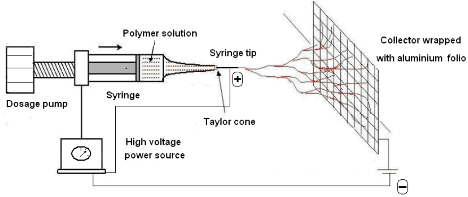
Fig. 1. Schematic representation of the electrospinning process.
