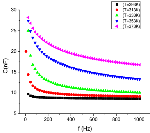
Fig.2. Variation of the capacitance with frequency of TlSbS 2 thin films at different temperatures. Film Thickness: 730A°
