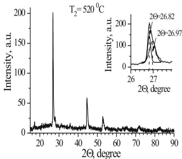
Fig. 4. XRD pattern of CIGSS film grown under 520 °C
