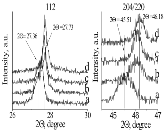
Fig. 5. Shift of (112) and (204/220) reflections CIGSS films in dependence on S/Se ratio: a - 0.77, b - 2.0, c - 3.3, d - 5.40.
