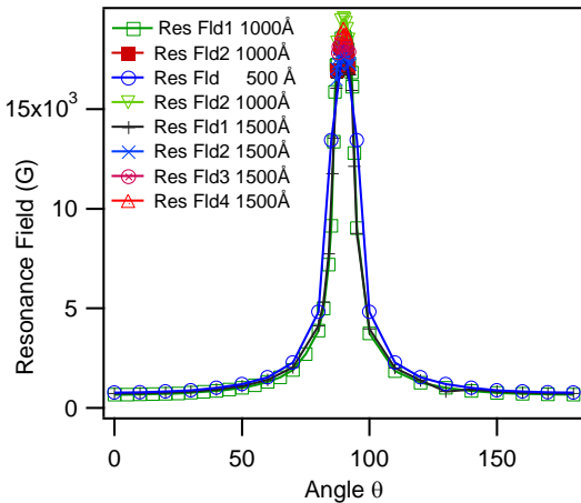
Fig. 6. The angular dependence of the resonance fields for all samples taken at room temperature for the perpendicular geometry. The value of resonance field is maximum at 90° where magnetic field is perpendicular to the film surfaces.
