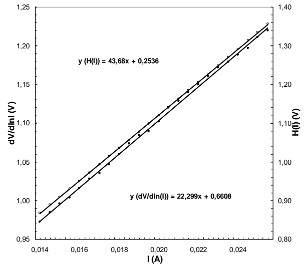
Fig 4. The dV/d\ln I - I and H(I) - I plots of Au/SrTiO 3 /n-Si (MFS) SBD.
