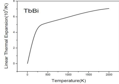
Fig. 9. The thermal expansion verses temperature for TbBi.
