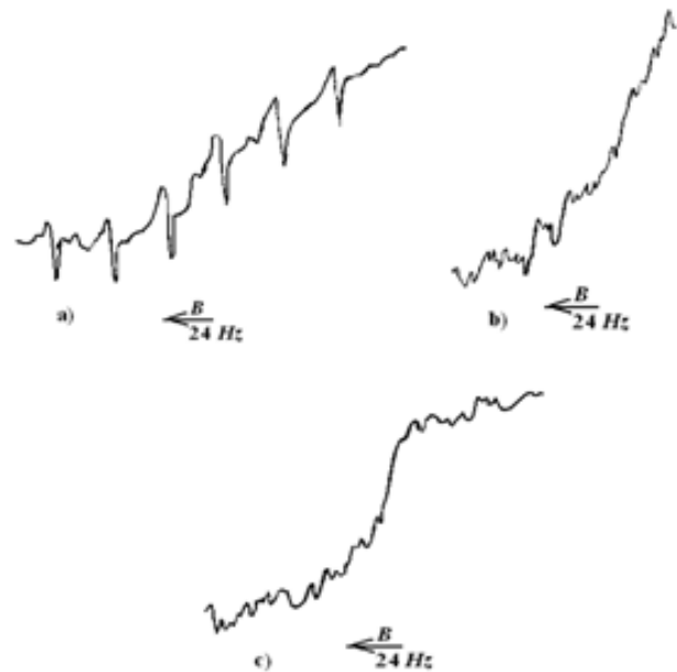
Fig. 4. The ESR spectra for the PP filled with segnetopiezoelectric PZT - 4.
