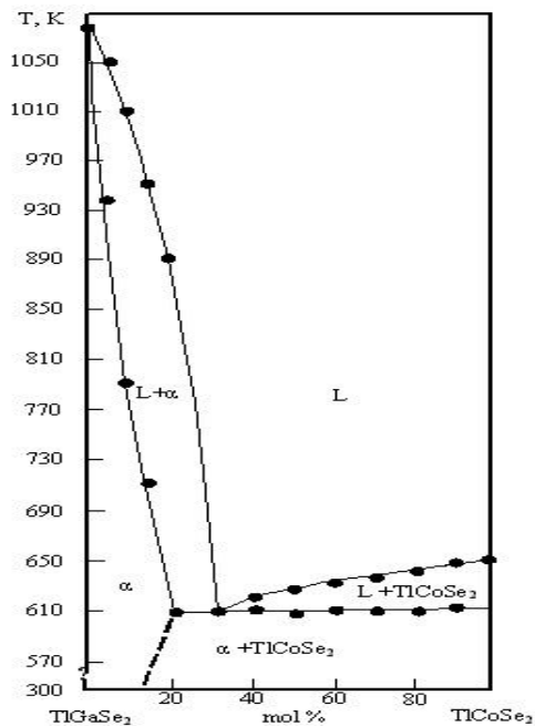
Fig.11. \text{TiGaSe}_2\text{-TiCoSe}_2 system state diagram.
