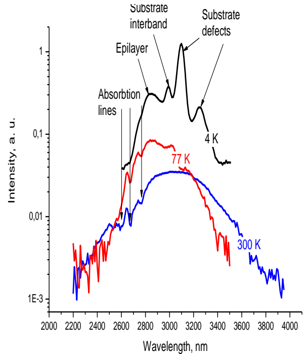
Fig.4. PL spectra of \text{Ga}_{0.04}\text{In}_{0.96}\text{As}_{0.77}\text{P}_{0.11}\text{Sb}_{0.11}/\text{InAs}(100)
