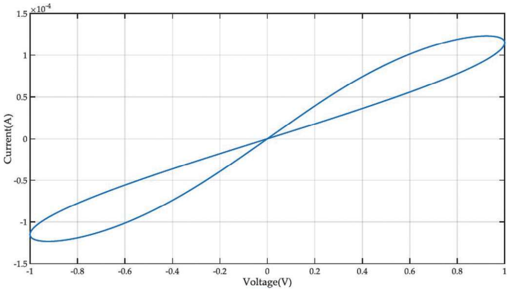
Figure 5. I-V pinched hysteresis loop of the memristor.
