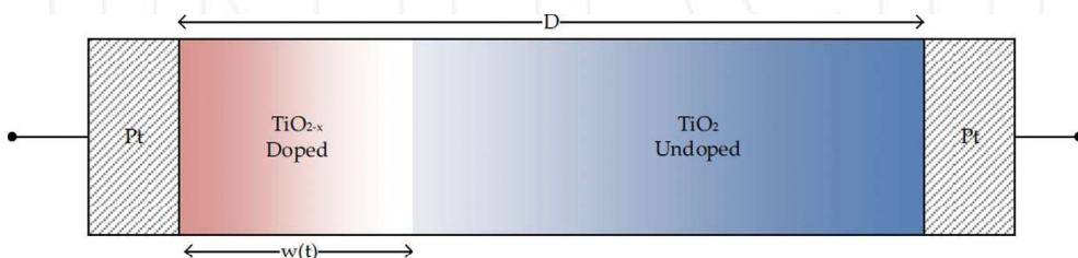
Figure 2. Structure of memristor reported by HP Lab [2].
