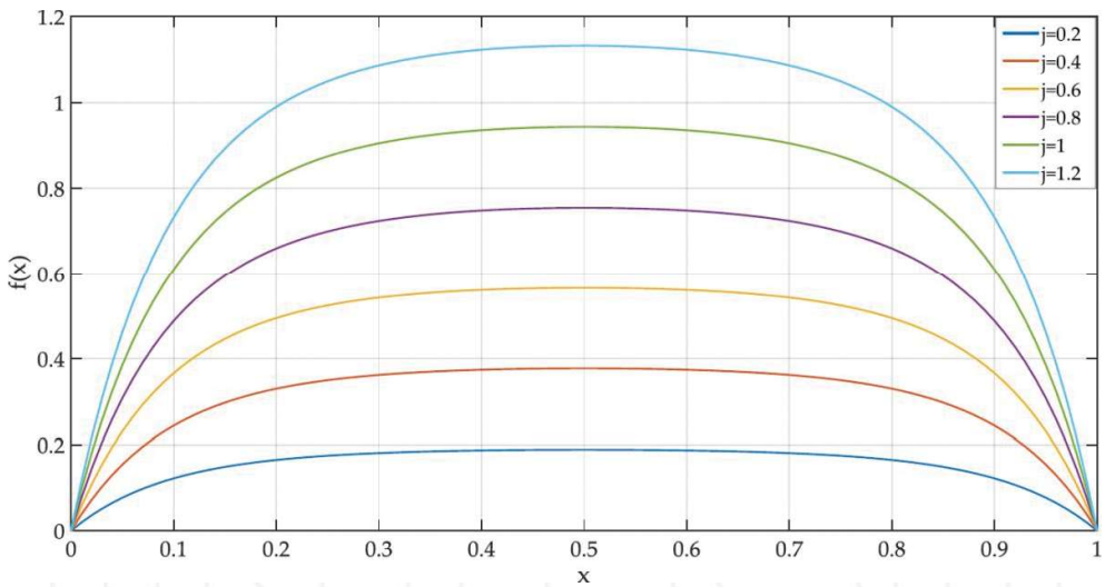
Figure 13. Prodomakis' window function for p = 10 and different j values.
