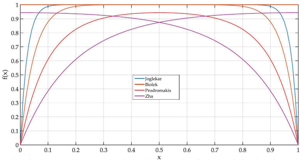
Figure 16. Different window functions for p = 10 and j = 1 .
