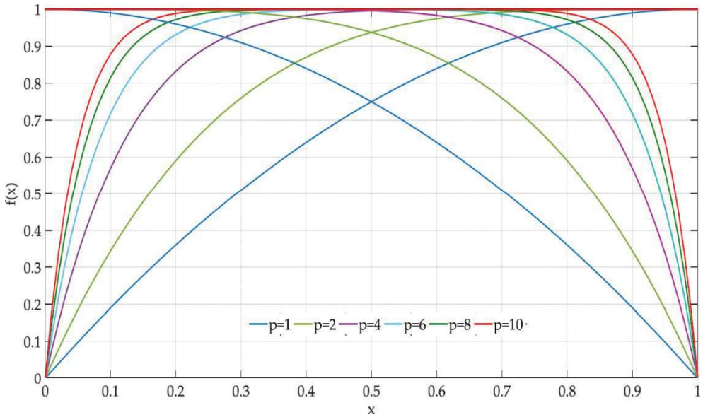
Figure 11. Biolek's window function for different p values.
