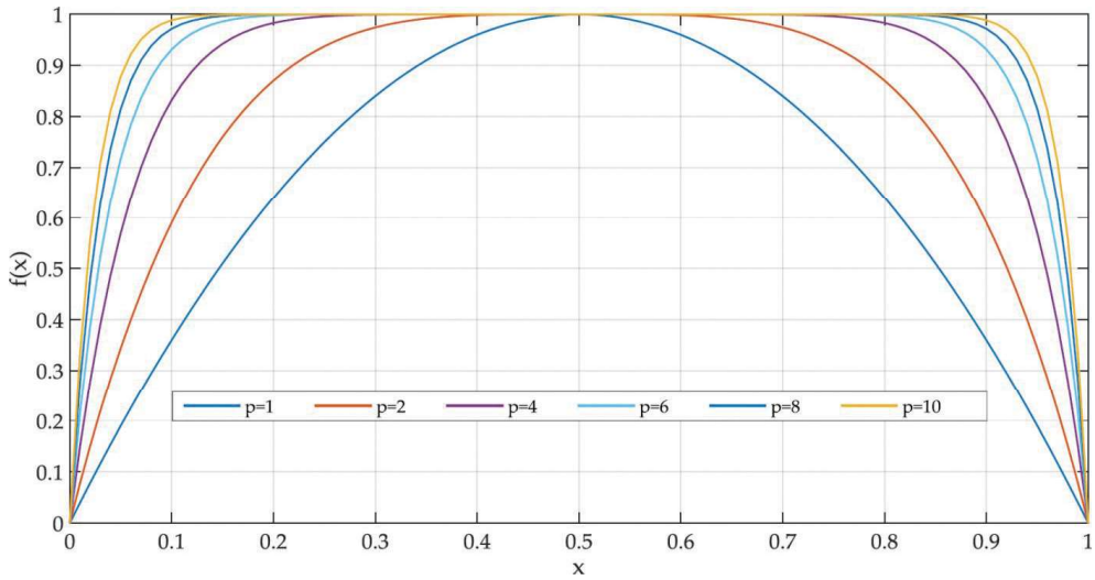
Figure 10. Joglekar window function for different p values.
