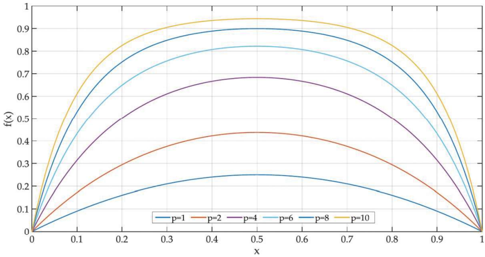
Figure 12. Prodomakis' window function for j = 1 and different p values.
