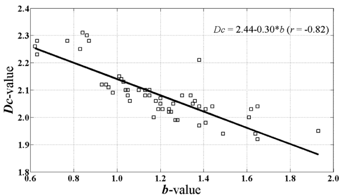
Figure 2. D_c -value compared to b -value for Turkish earthquakes occurring between 1970 and 2011. The statistical relationship (with its coefficient of correlation) is also given
