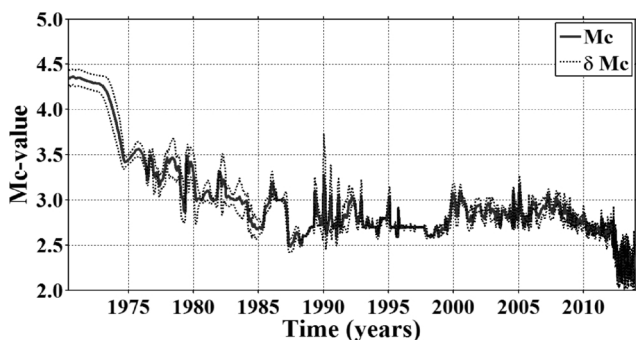
Figure 3: Variations of magnitude completeness M_c -value from 1970 to 2014 in the Western Anatolian region. Standard deviation ( \delta M_c ) of the completeness (dashed lines) is also given. M_c is plotted for overlapping samples, each containing 250 events
