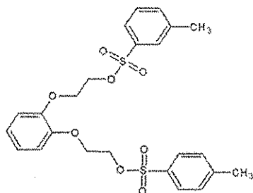
Fig. 1. Chemical structure of BTEB.
