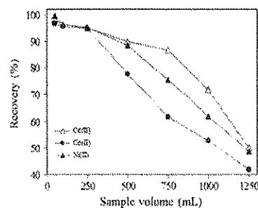
Fig. 4. Effect of sample volumes on the recoveries of analyte ions ( N=3 , sample pH: 7.0).
