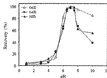
Fig. 2. Effect of pH on the recoveries of analyte ions ( N : 3, sample volume: 50 mL, quantity of BTEB: 15.0 mg, standing time: 30 min, centrifugation rate: 2,500 rpm, centrifugation time: 10 min).
