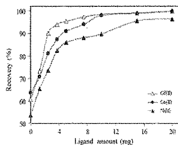
Fig. 3. Effect of BTEB amount on the recoveries of analyte ions ( N=3 , sample pH: 7.0, sample volume: 50 mL).
