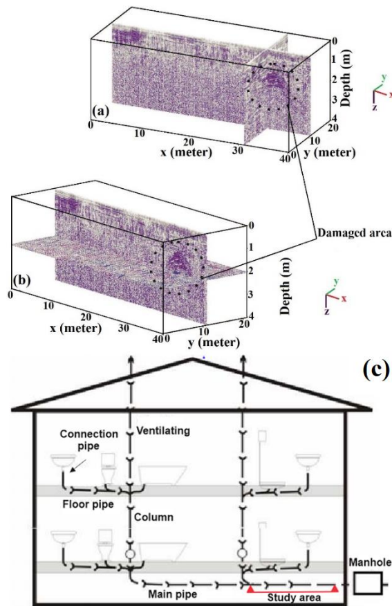
Figure 4. a) 3D image of damaged area by intersection of X and Y sections, b) Slice image of damaged area by intersection of Y section, c) Indoor wastewater installation pipe sections and representative study area (designed from URL-1, 2018).
