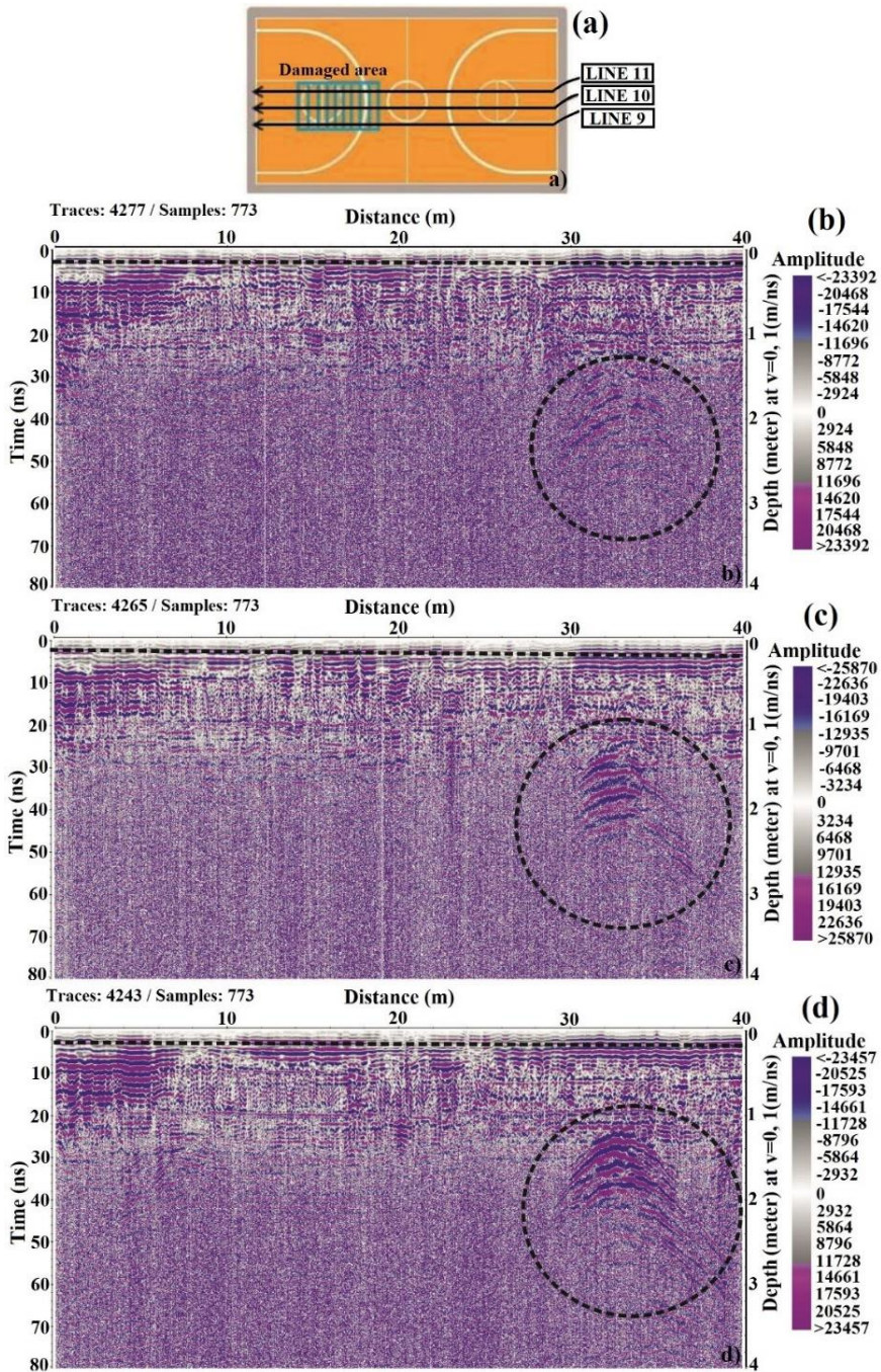
Figure 3. a) Field sketch and damaged area GUSC, b) Radargram section of line 9, c) Radargram section of line 10 and, d) Radargram section of line 11.
