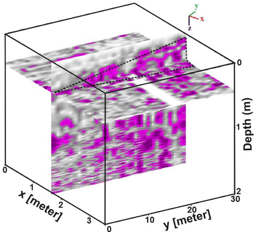
Figure 8. 3D image of slope by intersection of X and Y sections for study region 2.
