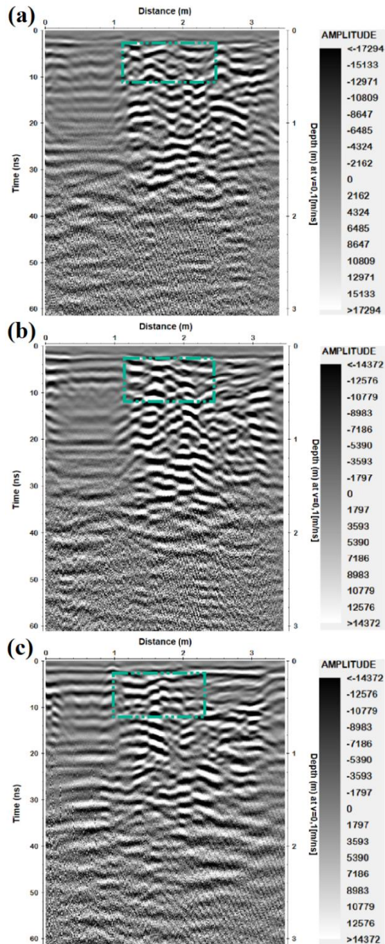
Figure 6. a) Radargram section of line 22 for study region 2, b) Radargram section of line 23 for study region 2 and c) Radargram section of line 29 for study region 2.
