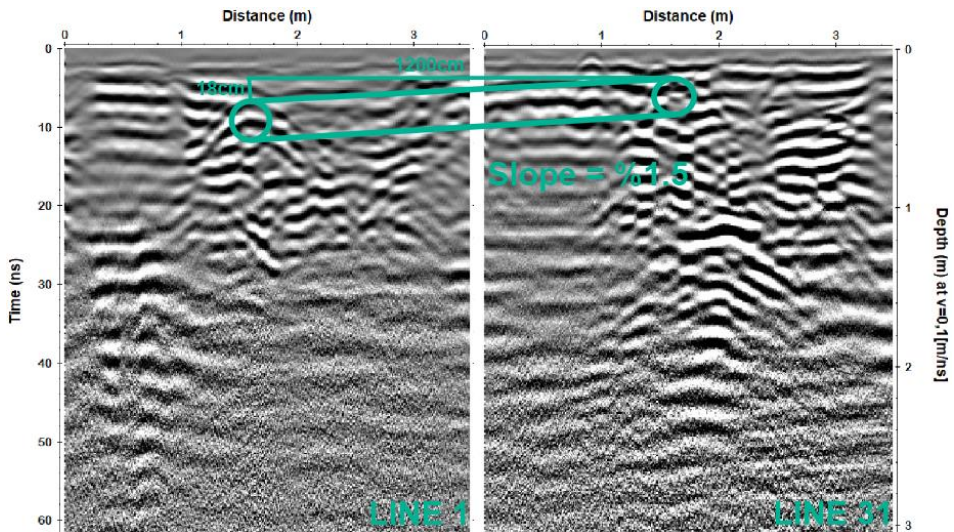
Figure 7. Slope image between line 1 st and line 31 st for study region 2.
