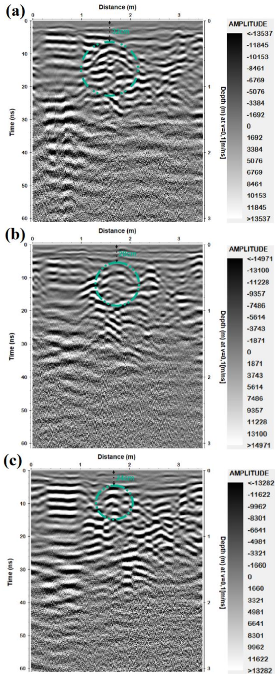
Figure 5. a) Radargram section of line 1 for study region 2, b) Radargram section of line 4 for study region 2 and c) Radargram section of line 14 for study region 2.
