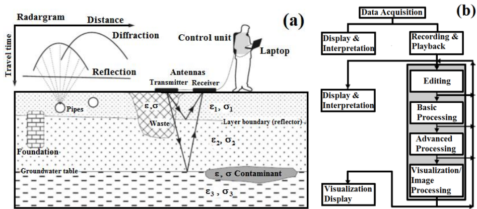
Figure 2. a) Representation of main components and principle of GPR system (modified from Knödel et al. [2]), b) Data processing stages of GPR method (modified from Annan [28]).
